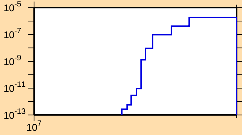
\sigma vs. E for ^{138}\text{Eu}(n,2n\alpha)
