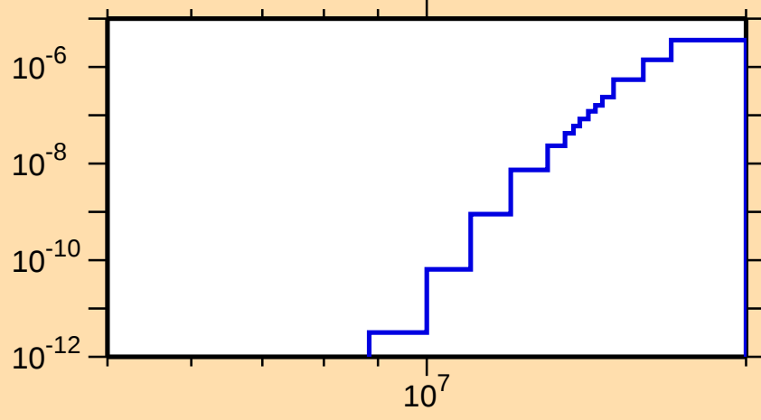
\sigma vs. E for ^{138}\text{Eu}(\text{mt117})
