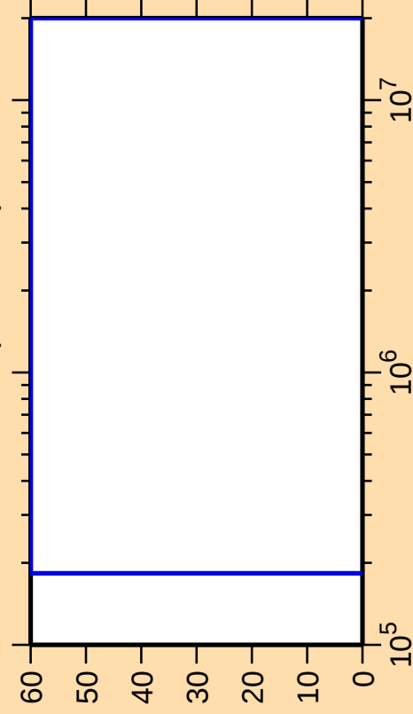
\Delta\sigma/\sigma vs. E for ^{138}\text{Eu}(\text{n},\text{ncont.})
