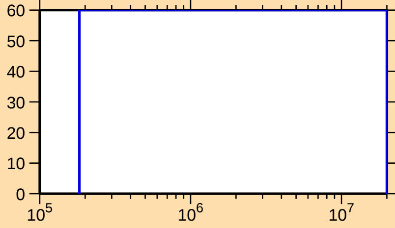
\Delta\sigma/\sigma vs. E for ^{138}\text{Eu}(n,n_1)
