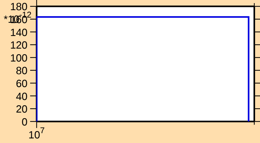
\sigma vs. E for ^{138}\text{Eu}(\text{mt } 34)
