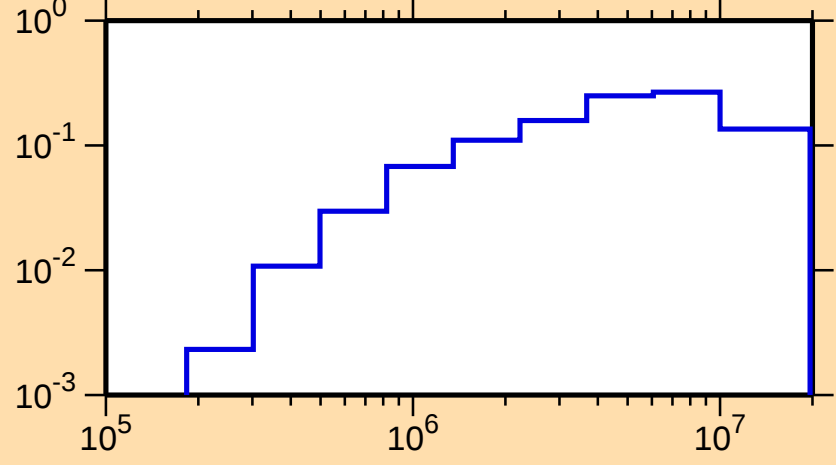
\sigma vs. E for ^{138}\text{Eu}(n,\text{inel.})
