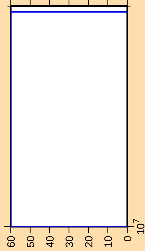
\Delta\sigma/\sigma vs. E for ^{138}\text{Eu}(\text{mt } 34)
