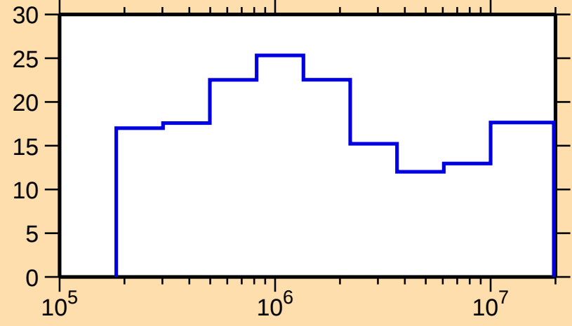
\Delta\sigma/\sigma vs. E for ^{138}\text{Eu}(n,\text{nonel.})
