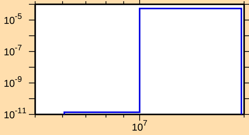
\sigma vs. E for ^{138}\text{Eu}(\text{mt } 45)
