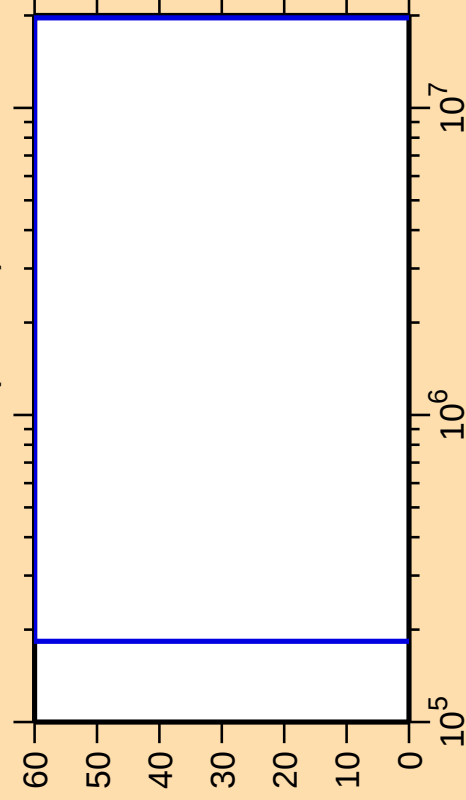
\Delta\sigma/\sigma vs. E for ^{138}\text{Eu}(n,\text{inel.})
