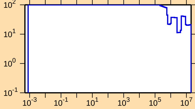
\Delta\sigma/\sigma vs. E for ^{142}\text{Eu}(n,\text{el.})
