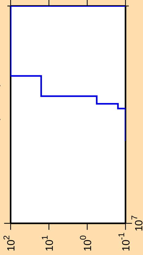
\Delta\sigma/\sigma vs. E for ^{142}\text{Eu}(\text{mt } 34)
