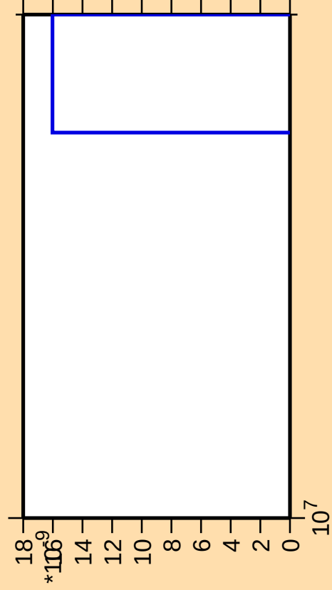
\Delta\sigma/\sigma vs. E for ^{142}\text{Eu} (mt 11)
