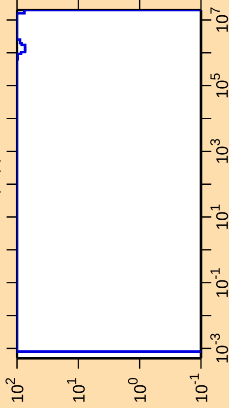
\Delta\sigma/\sigma vs. E for ^{142}\text{Eu}(n,p)
