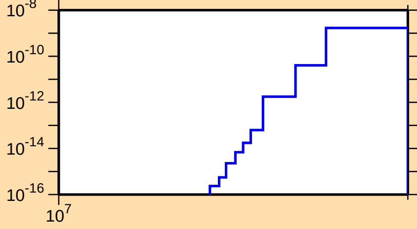
\sigma vs. E for ^{142}\text{Eu}(\text{mt } 34)
