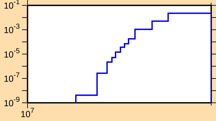
\sigma vs. E for ^{142}\text{Eu}(n,2np)
