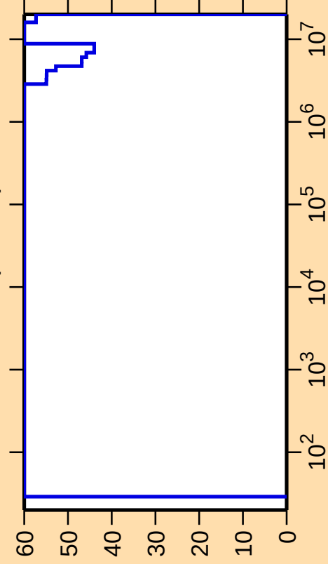
\Delta\sigma/\sigma vs. E for ^{142}\text{Eu}(n,\text{inel.})
