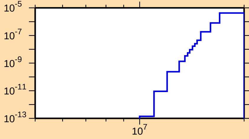
\sigma vs. E for ^{142}\text{Eu}(\text{mt } 45)
