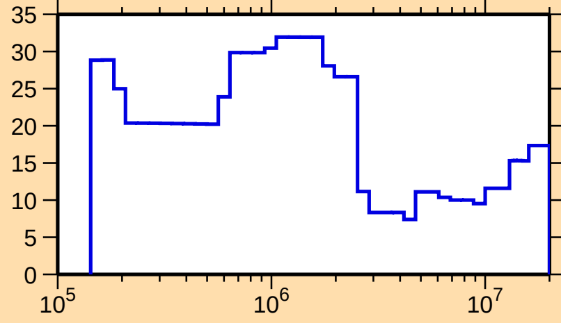
\Delta\sigma/\sigma vs. E for ^{162}\text{Eu}(n,\text{tot.})
