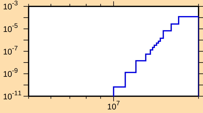
\sigma vs. E for ^{162}\text{Eu}(n,n\alpha)
