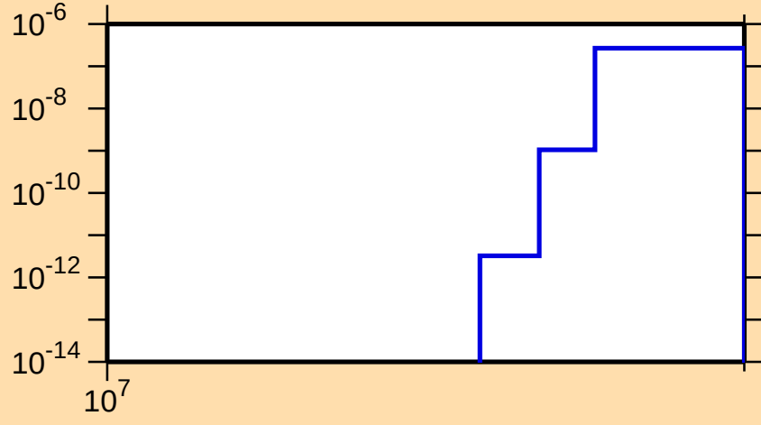
\sigma vs. E for ^{162}\text{Eu}(n,2np)
