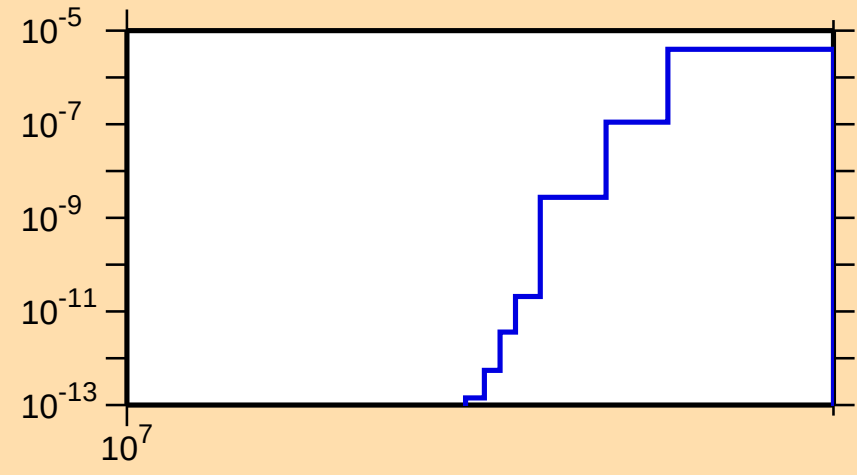
\sigma vs. E for ^{162}\text{Eu}(n,\text{nd})
