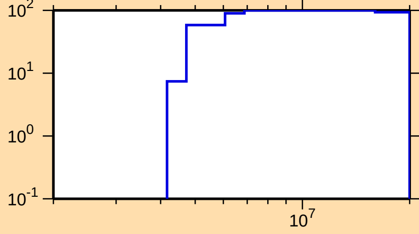
\Delta\sigma/\sigma vs. E for ^{162}\text{Eu}(n,\text{inel.})
