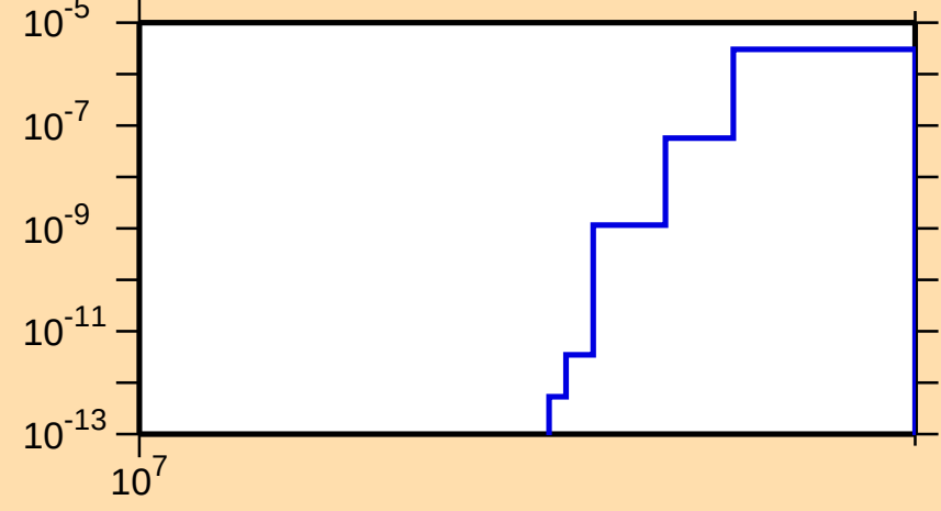
\sigma vs. E for ^{162}\text{Eu}(n,nt)
