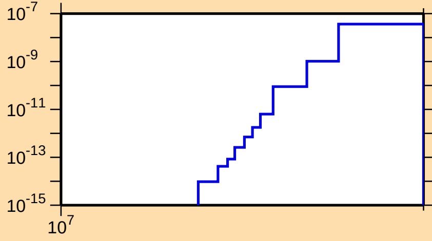
\sigma vs. E for ^{162}\text{Eu}(n,2n\alpha)
