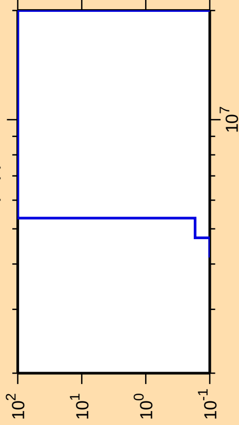
\Delta\sigma/\sigma vs. E for ^{162}\text{Eu}(n,p)
