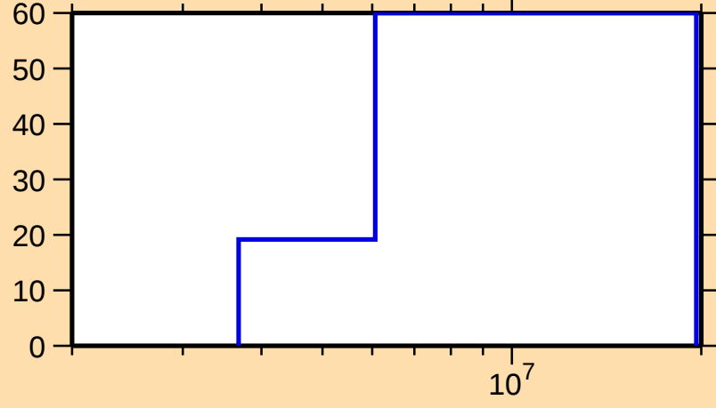
\Delta\sigma/\sigma vs. E for ^{162}\text{Eu}(n,n\text{cont.})
