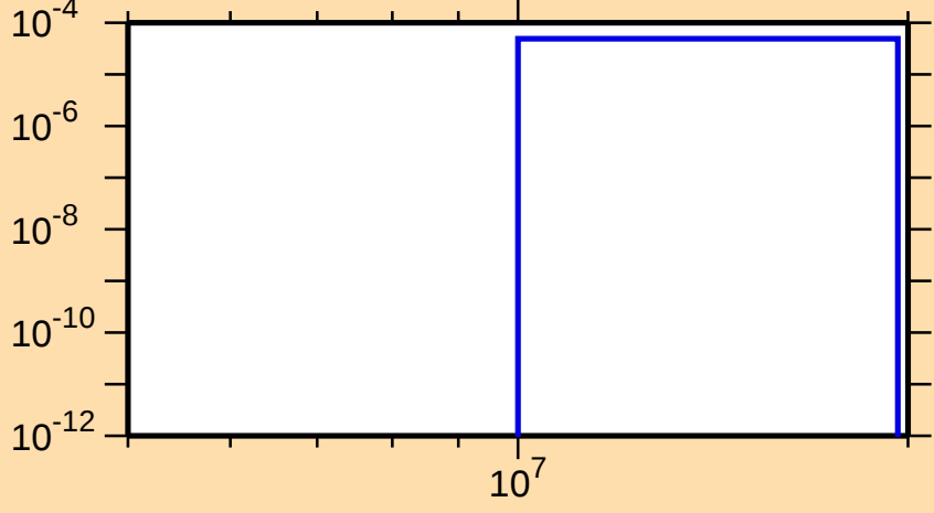
\sigma vs. E for ^{162}\text{Eu}(n,d)
