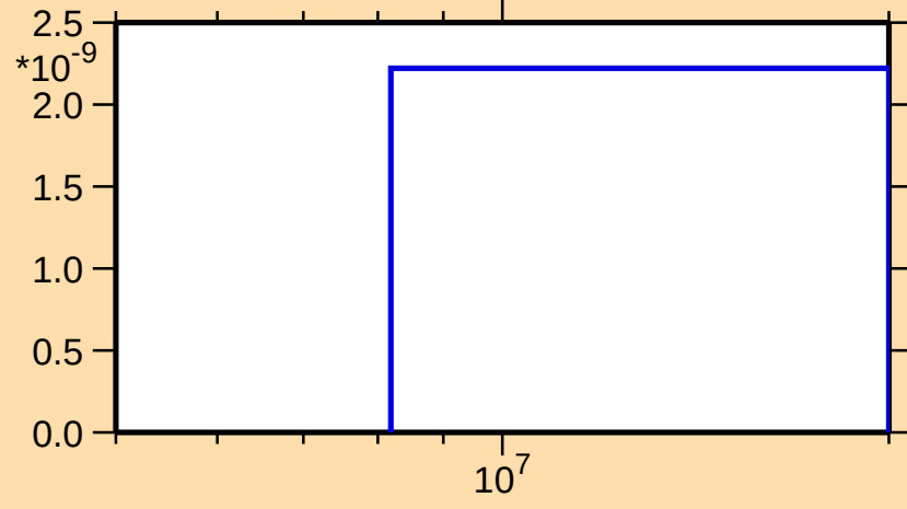
\sigma vs. E for ^{162}\text{Eu}(n,2np)
