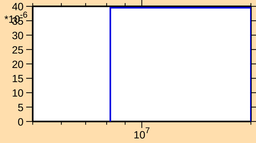
\sigma vs. E for ^{162}\text{Eu}(n,d)
