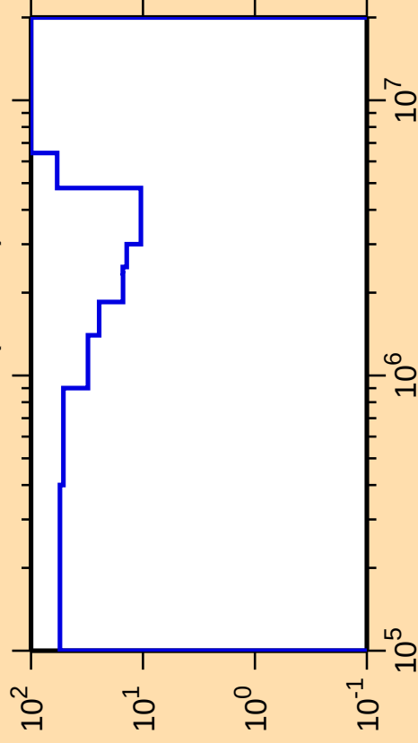
\Delta\sigma/\sigma vs. E for ^{162}\text{Eu}(n,\text{inel.})
