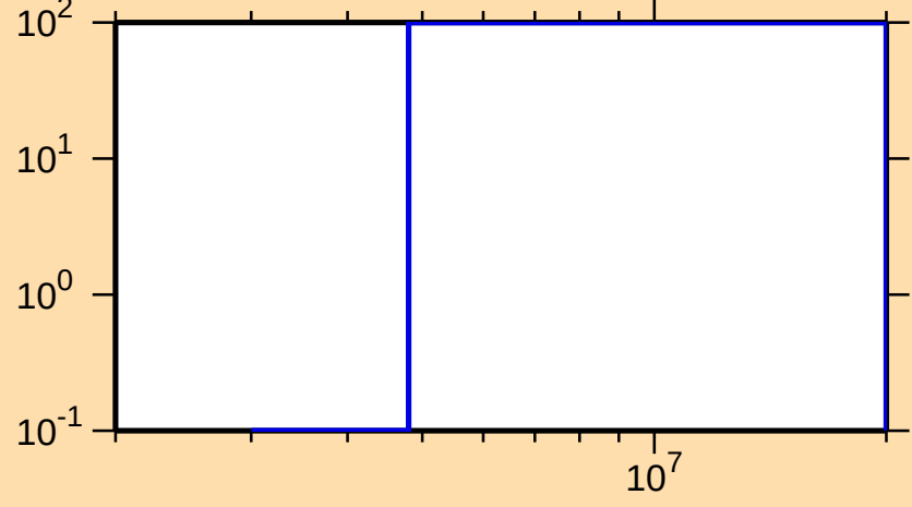
\Delta\sigma/\sigma vs. E for ^{162}\text{Eu}(n,p)
