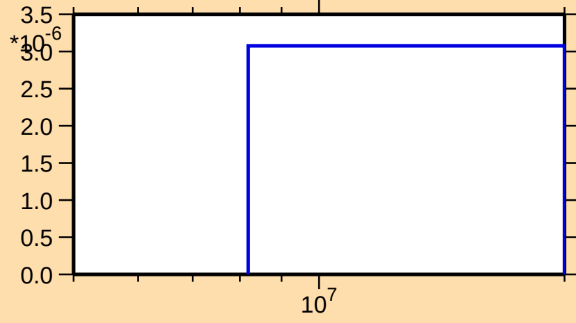
\sigma vs. E for ^{162}\text{Eu}(n,n\alpha)
