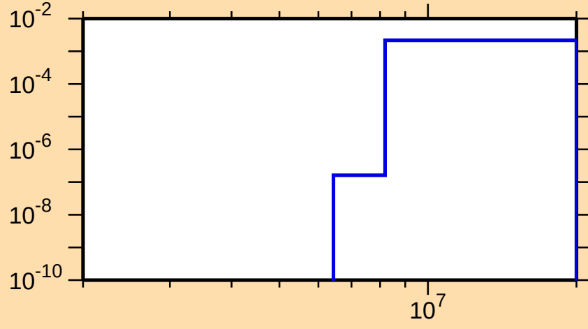
\sigma vs. E for ^{162}\text{Eu}(n,p)
