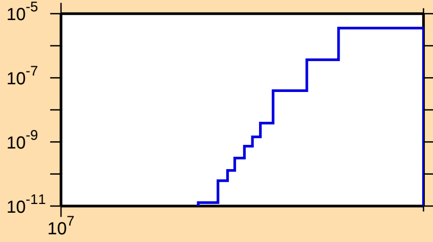
\sigma vs. E for ^{139}\text{Gd}(n,2n\alpha)
