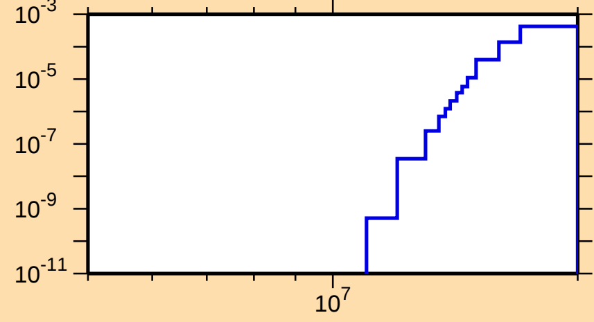
\sigma vs. E for ^{139}\text{Gd}(n,\text{pt})
