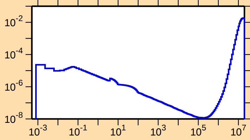
\sigma vs. E for ^{139}\text{Gd}(n,p\alpha)
