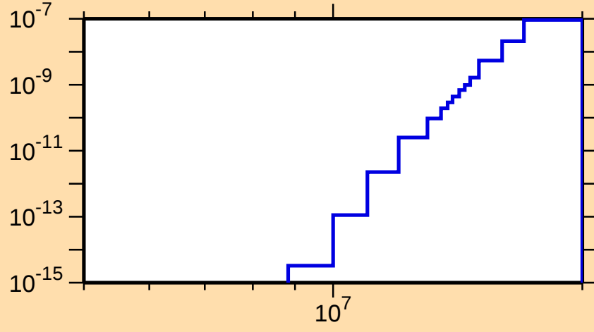
\sigma vs. E for ^{139}\text{Gd}(\text{mt117})
