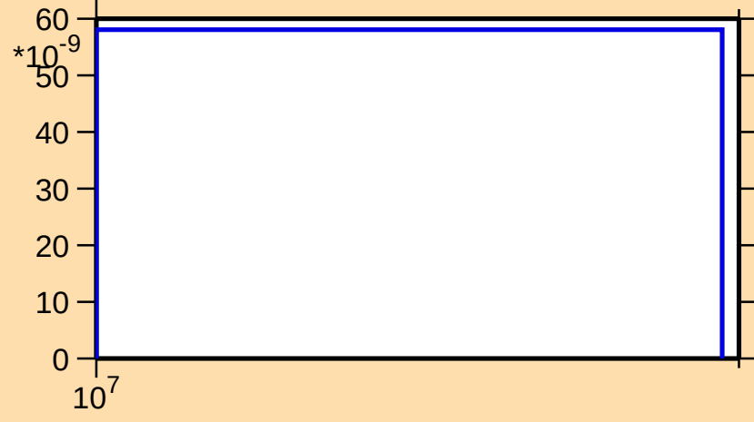
\sigma vs. E for ^{139}\text{Gd}(n,2n\alpha)
