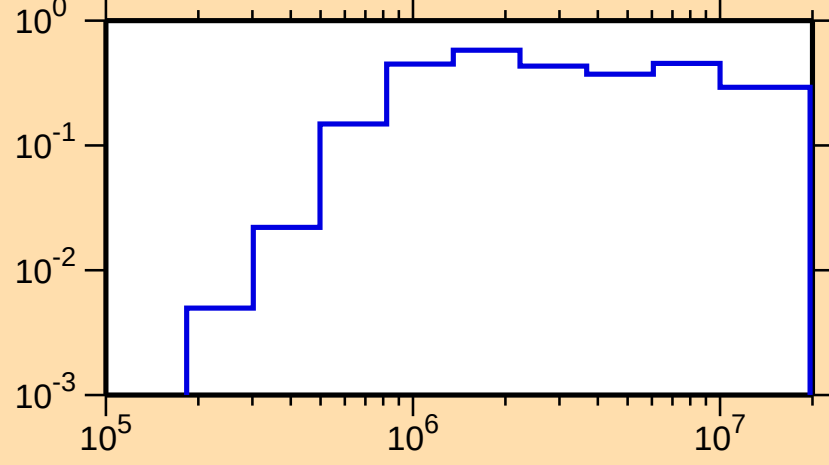
\sigma vs. E for ^{139}\text{Gd}(n,\text{inel.})
