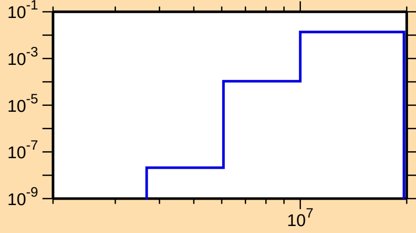
\sigma vs. E for ^{139}\text{Gd}(n,d)
