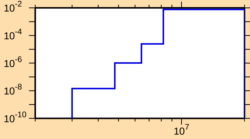
\sigma vs. E for ^{139}\text{Gd}(n,n\alpha)
