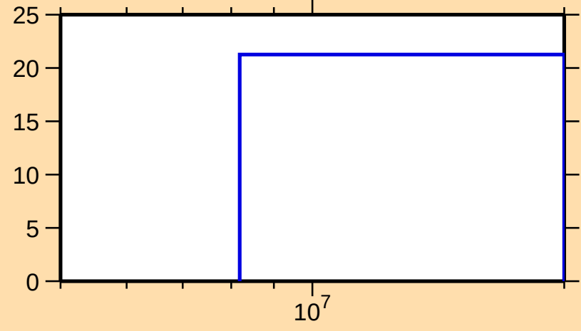
\Delta\sigma/\sigma vs. E for ^{139}\text{Gd}(n,\text{tot.})
