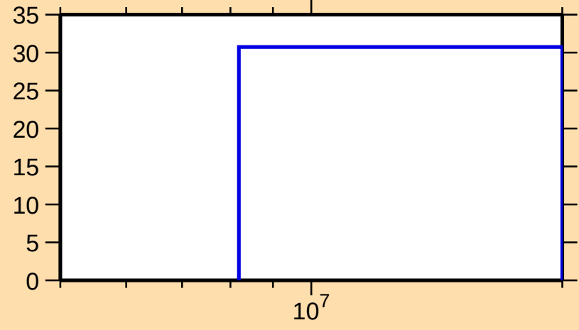
\Delta\sigma/\sigma vs. E for ^{139}\text{Gd}(n,\text{el.})
