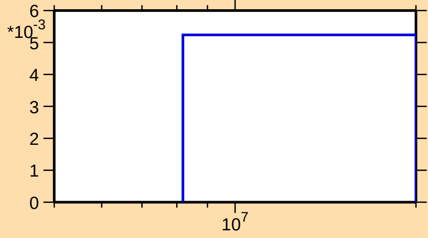
\sigma vs. E for ^{139}\text{Gd}(n,2n)
