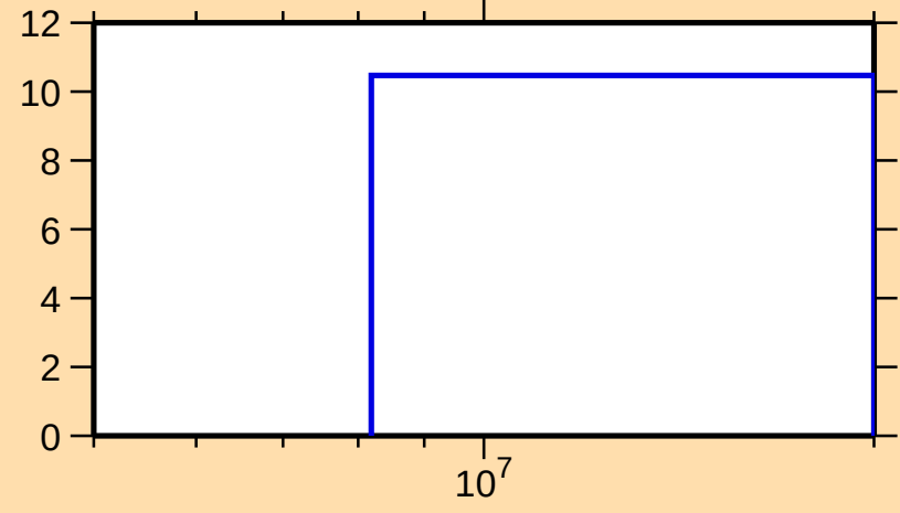
\Delta\sigma/\sigma vs. E for ^{139}\text{Gd}(n,\text{nonel.})
