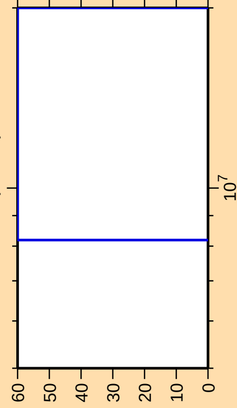
\Delta\sigma/\sigma vs. E for ^{139}\text{Gd}(\text{mt } 34)
