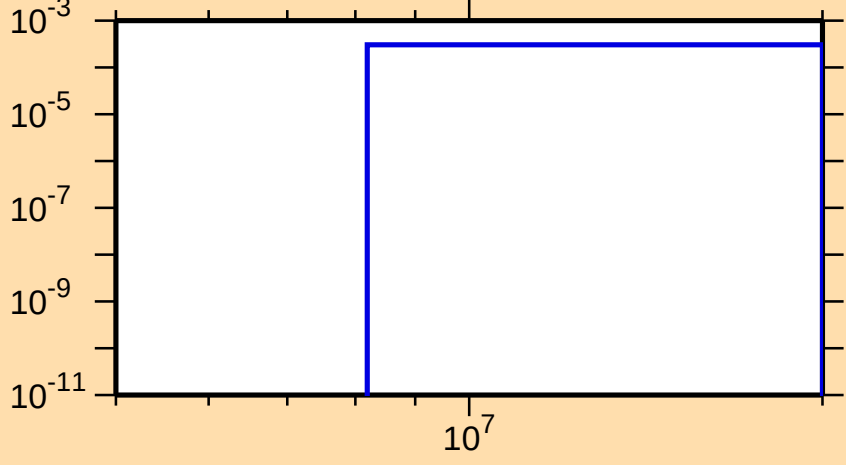
\sigma vs. E for ^{139}\text{Gd}(n,\text{pd})
