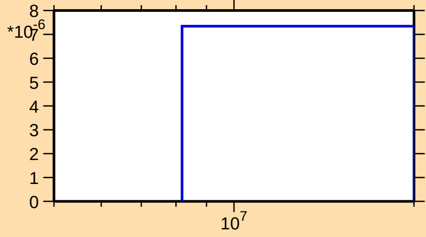
\sigma vs. E for ^{139}\text{Gd}(n,2np)
