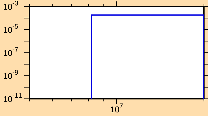
\sigma vs. E for ^{139}\text{Gd}(n,t)
