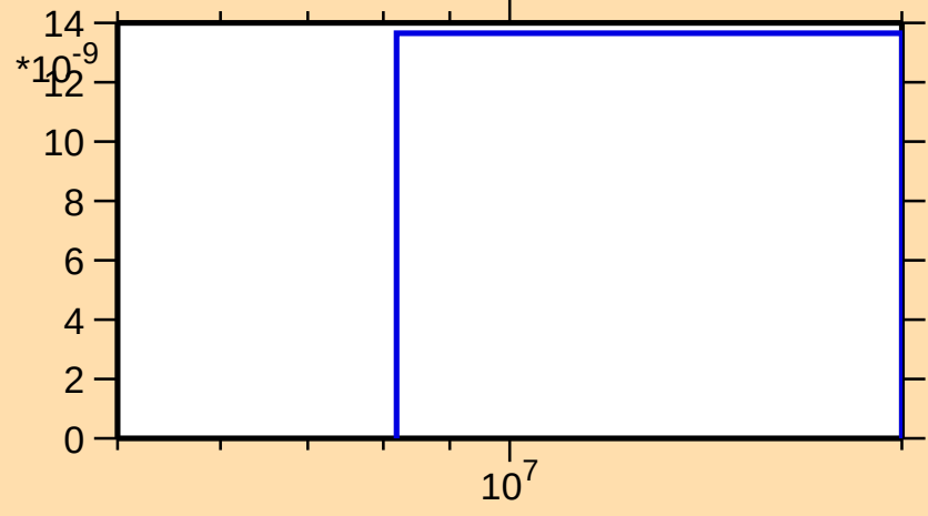
\sigma vs. E for ^{139}\text{Gd}(n,\text{nd})
