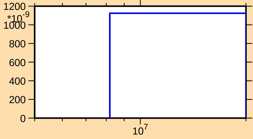
\sigma vs. E for ^{139}\text{Gd}(\text{mt } 45)
