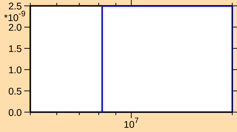
\sigma vs. E for ^{139}\text{Gd}(\text{mt117})
