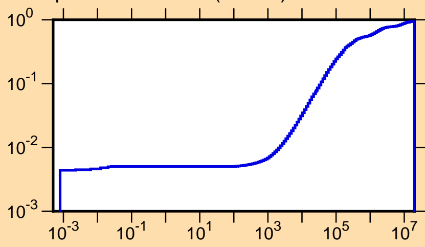
\mu vs. E for ^{155}\text{Gd}(\text{mt251})
