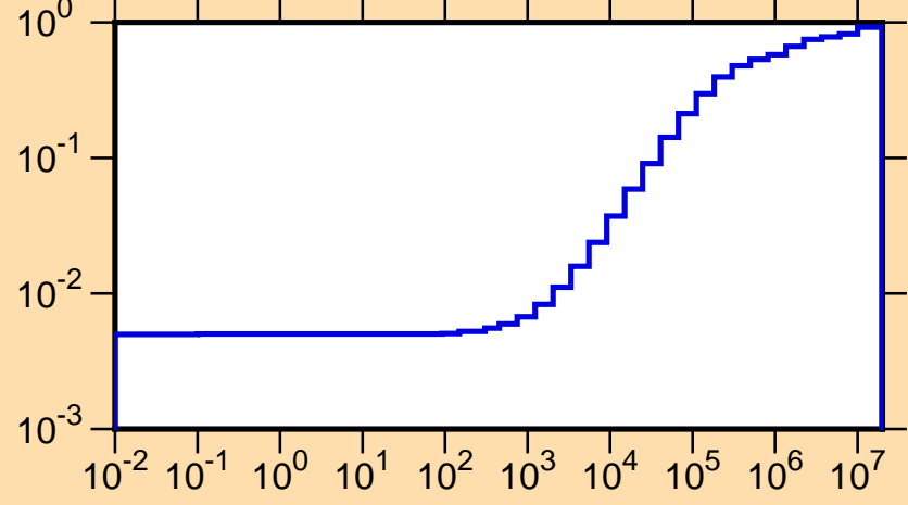
\mu vs. E for ^{155}\text{Gd}(\text{mt251})
