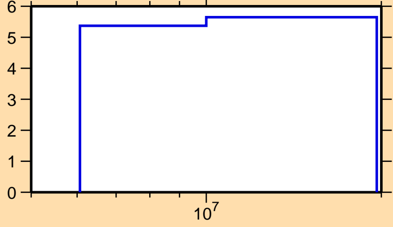
\Delta\sigma/\sigma vs. E for ^{155}\text{Gd}(n,\text{el.})
