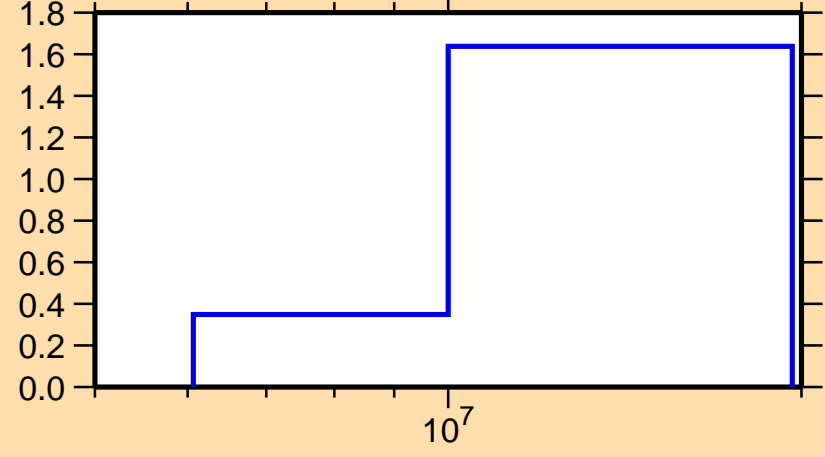
\sigma vs. E for ^{155}\text{Gd}(n,2n)
