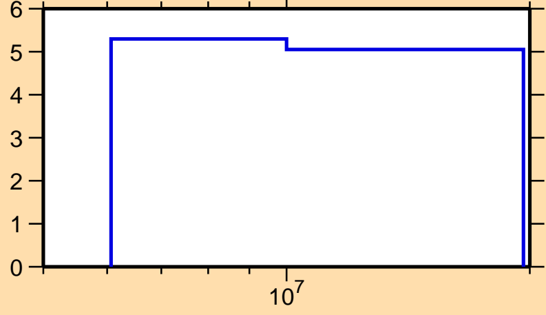
\Delta\sigma/\sigma vs. E for ^{155}\text{Gd}(n,\text{nonel.})
