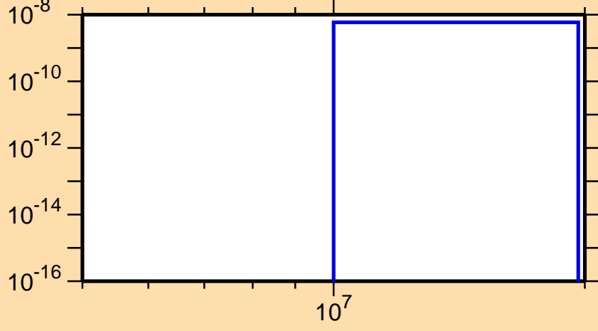
\sigma vs. E for ^{155}\text{Gd}(n,2n\alpha)
