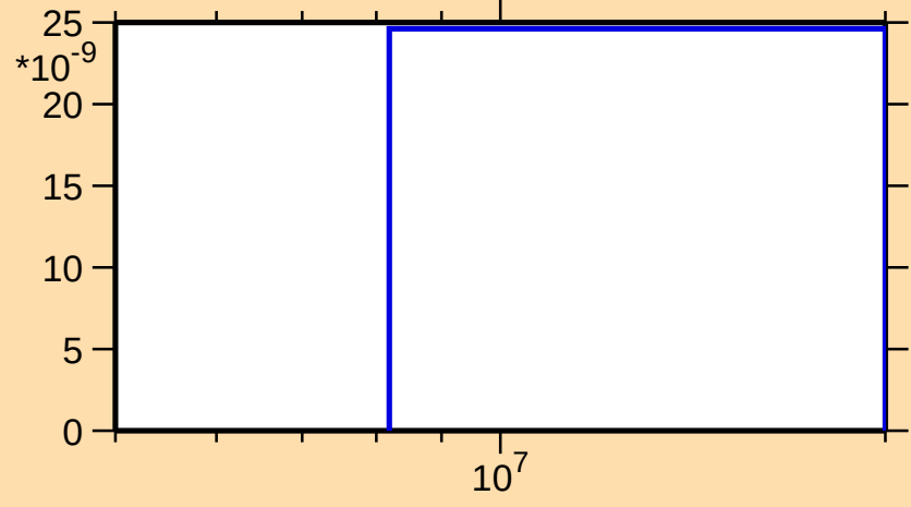
\sigma vs. E for ^{155}\text{Gd}(n,\text{nd})
