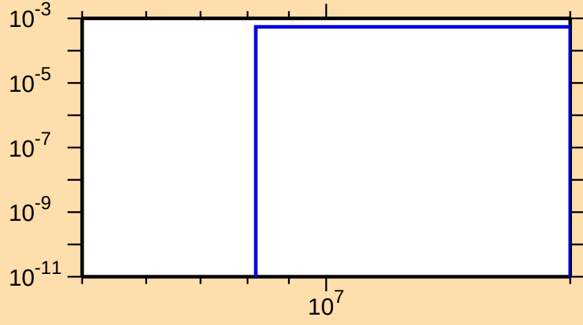
\sigma vs. E for ^{155}\text{Gd}(n,d)
