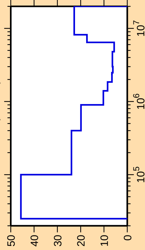
\Delta\sigma/\sigma vs. E for ^{155}\text{Gd}(n,\text{inel.})
