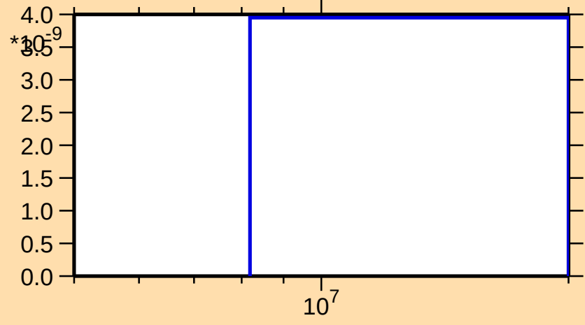
\sigma vs. E for ^{155}\text{Gd}(n,2np)
