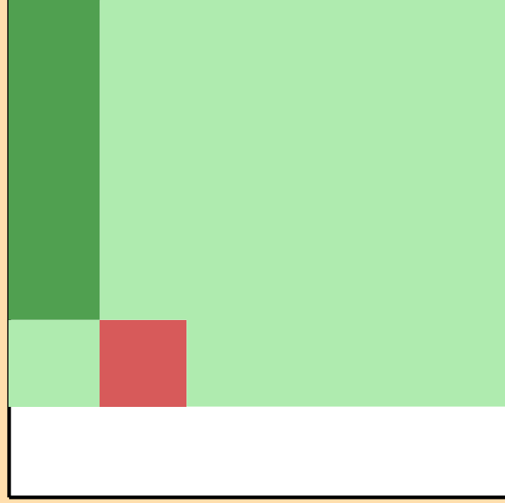
\Delta\sigma/\sigma vs. E for ^{155}\text{Gd}(n,\text{tot.})
