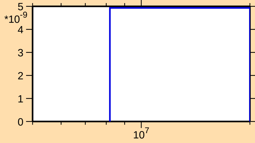
\sigma vs. E for ^{155}\text{Gd}(n,2n\alpha)
