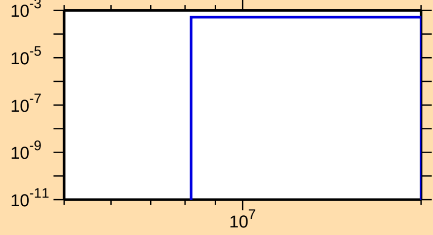
\sigma vs. E for ^{155}\text{Gd}(n,np)
