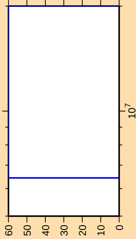
\Delta\sigma/\sigma vs. E for ^{155}\text{Gd}(n,\alpha)
