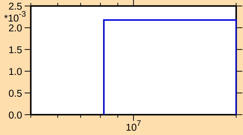
\sigma vs. E for ^{155}\text{Gd}(n,3n)
