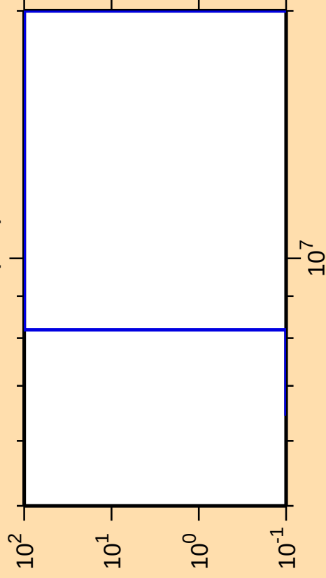
\Delta\sigma/\sigma vs. E for ^{155}\text{Gd}(n,d)
