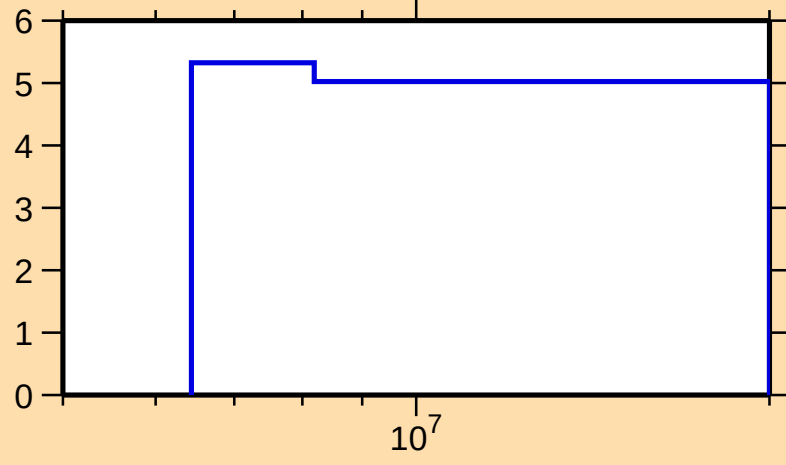
\Delta\sigma/\sigma vs. E for ^{155}\text{Gd}(n,\text{nonel.})
