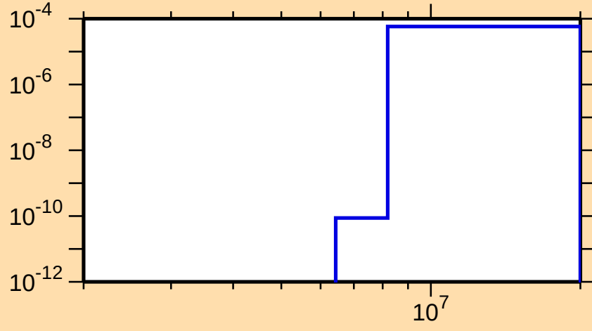
\sigma vs. E for ^{155}\text{Gd}(n,\alpha)
