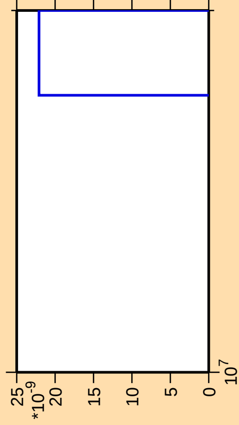
\Delta\sigma/\sigma vs. E for ^{166}\text{Gd}(\text{mt } 11)
