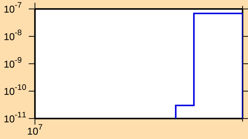
\sigma vs. E for ^{166}\text{Gd}(n,\text{nt})
