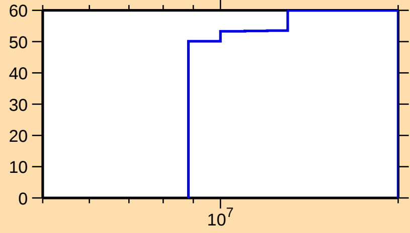
\Delta\sigma/\sigma vs. E for ^{166}\text{Gd}(n,n\text{cont.})
