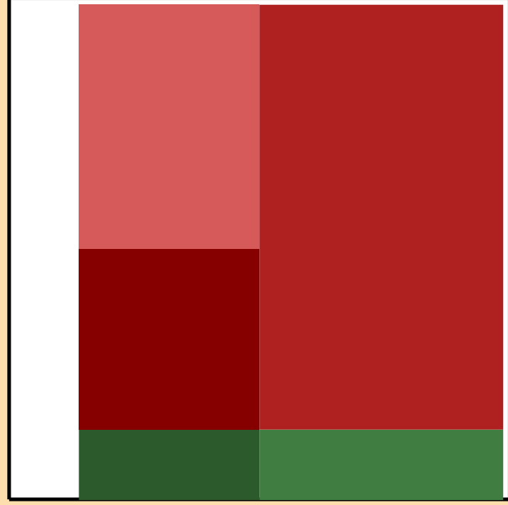
\Delta\sigma/\sigma vs. E for ^{166}\text{Gd}(n,2n)
