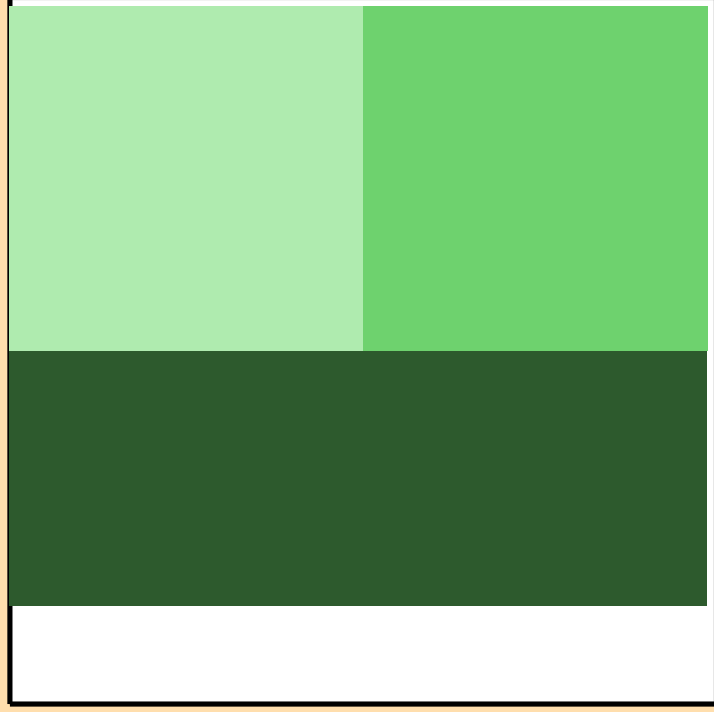
\Delta\sigma/\sigma vs. E for ^{166}\text{Gd}(n,\gamma)
