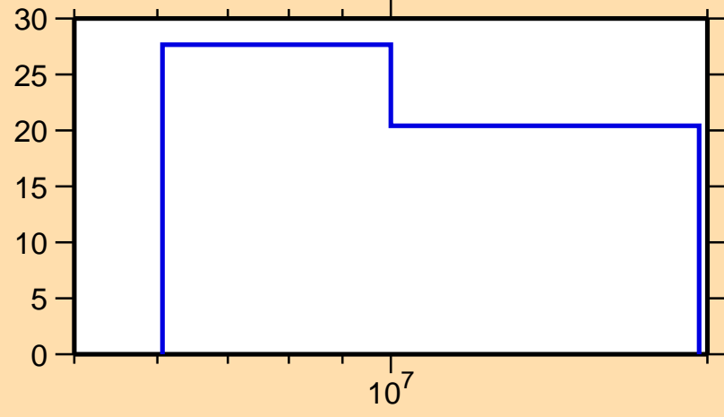
\Delta\sigma/\sigma vs. E for ^{166}\text{Gd}(n,el.)
