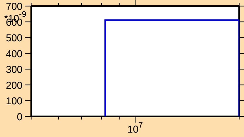
\sigma vs. E for ^{166}\text{Gd}(n,n\alpha)
