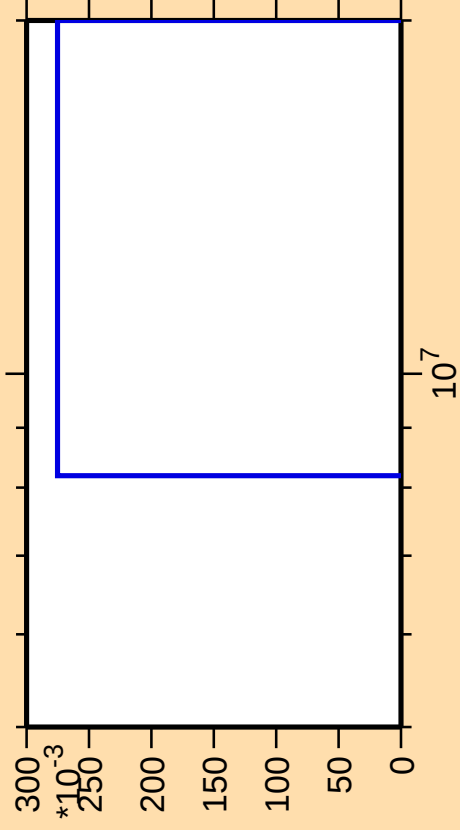
\Delta\sigma/\sigma vs. E for ^{166}\text{Gd}(n,2np)
