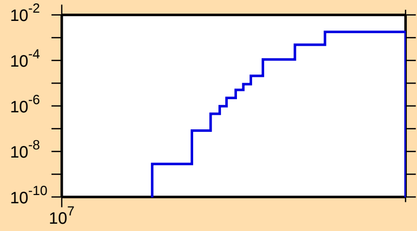
\sigma vs. E for ^{156}\text{Ho}(n,2np)
