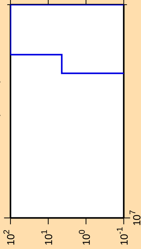
\Delta\sigma/\sigma vs. E for ^{156}\text{Ho}(\text{mt } 34)
