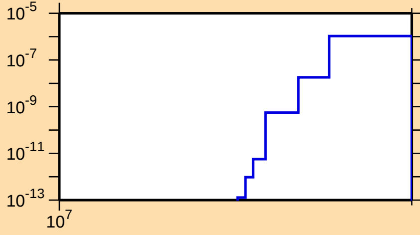
\sigma vs. E for ^{156}\text{Ho}(n,nt)
