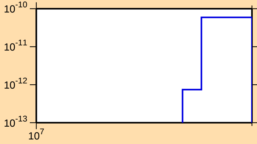
\sigma vs. E for ^{156}\text{Ho}(n,\text{pt})
