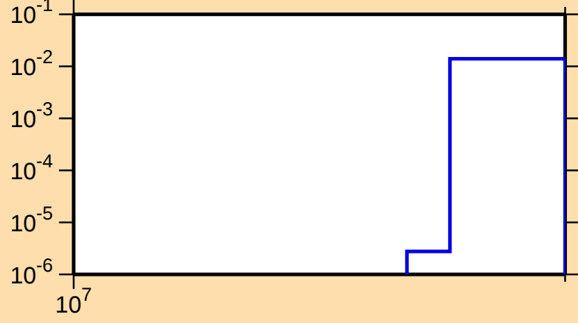
\sigma vs. E for ^{156}\text{Ho}(n,3n)
