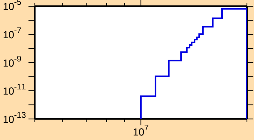
\sigma vs. E for ^{156}\text{Ho}(n,\text{He3})
