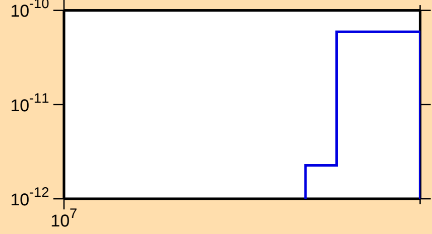
\sigma vs. E for ^{156}\text{Ho}(n,\text{pd})
