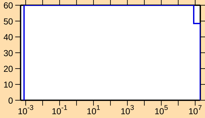
\Delta\sigma/\sigma vs. E for ^{156}\text{Ho}(n,p)
