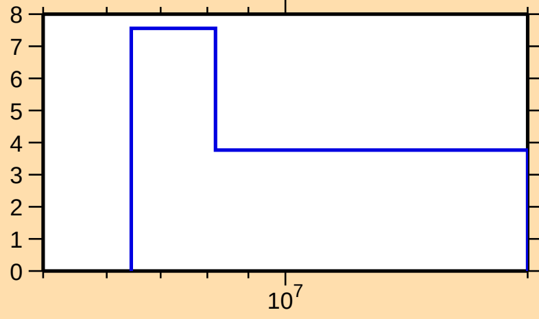
\Delta\sigma/\sigma vs. E for ^{156}\text{Ho}(n,\text{el.})
