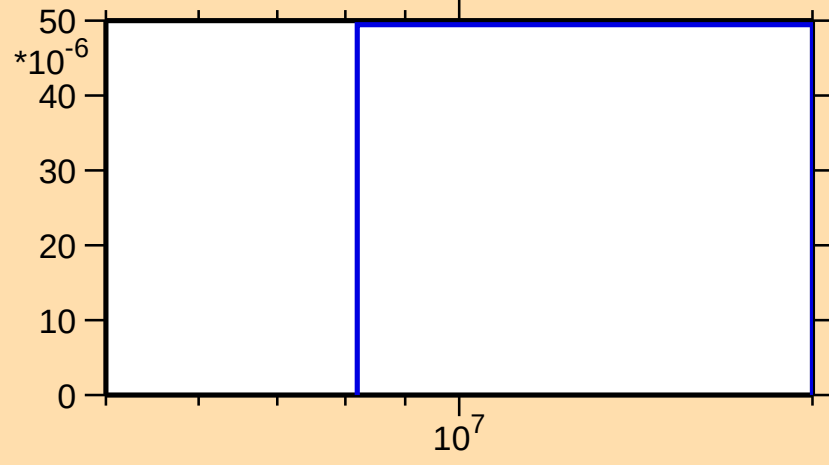
\sigma vs. E for ^{156}\text{Ho}(n,2np)
