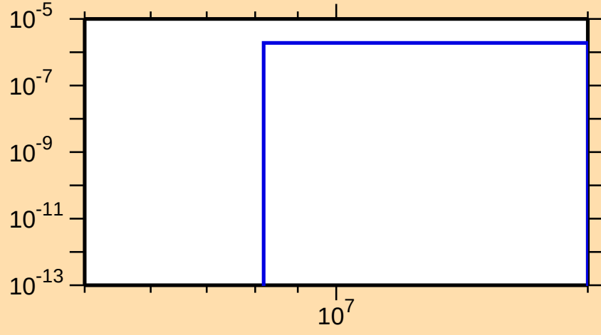
\sigma vs. E for ^{156}\text{Ho}(n,\text{nd})
