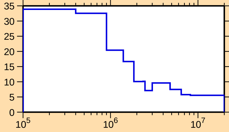
\Delta\sigma/\sigma vs. E for ^{156}\text{Ho}(n,\text{nonel.})
