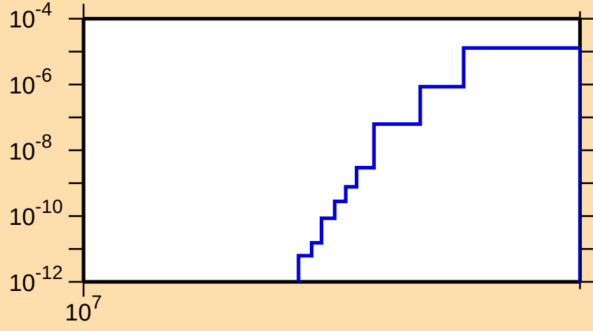
\sigma vs. E for ^{166}\text{Ho}(n,\text{nd})
