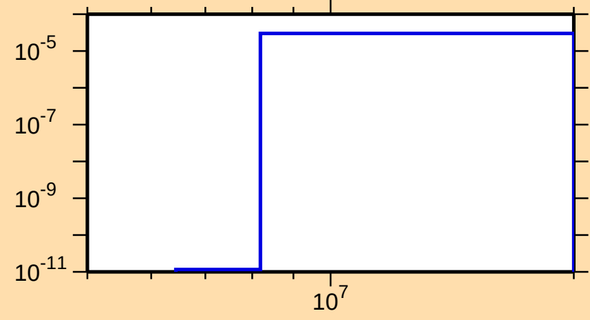
\sigma vs. E for ^{166}\text{Ho}(n,\alpha)
