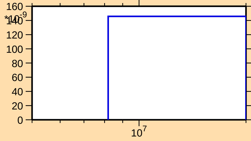
\sigma vs. E for ^{166}\text{Ho}(n,\text{nd})
