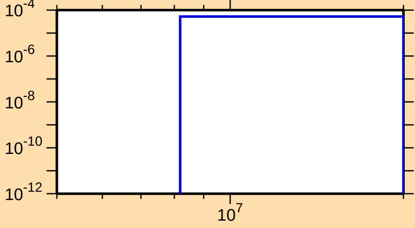
\sigma vs. E for ^{166}\text{Ho}(n,t)
