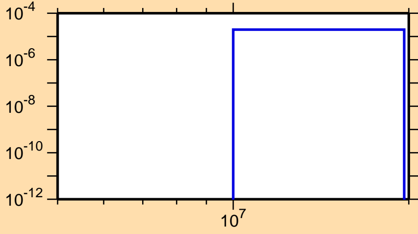
\sigma vs. E for ^{171}\text{Ho}(n,t)
