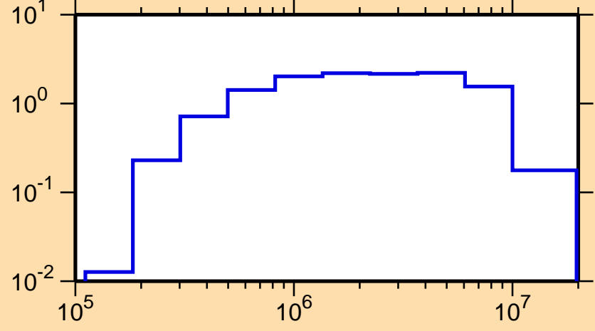
\sigma vs. E for ^{171}\text{Ho}(n,n\text{cont.})
