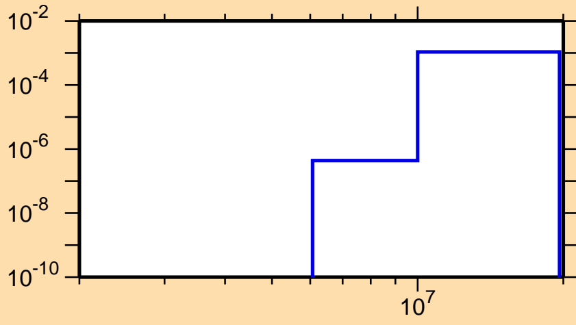
\sigma vs. E for ^{171}\text{Ho}(n,p)
