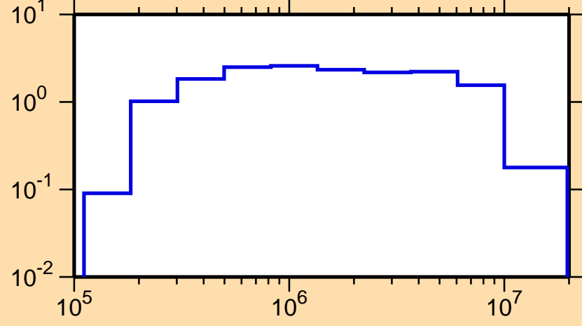
\sigma vs. E for ^{171}\text{Ho}(n,\text{inel.})
