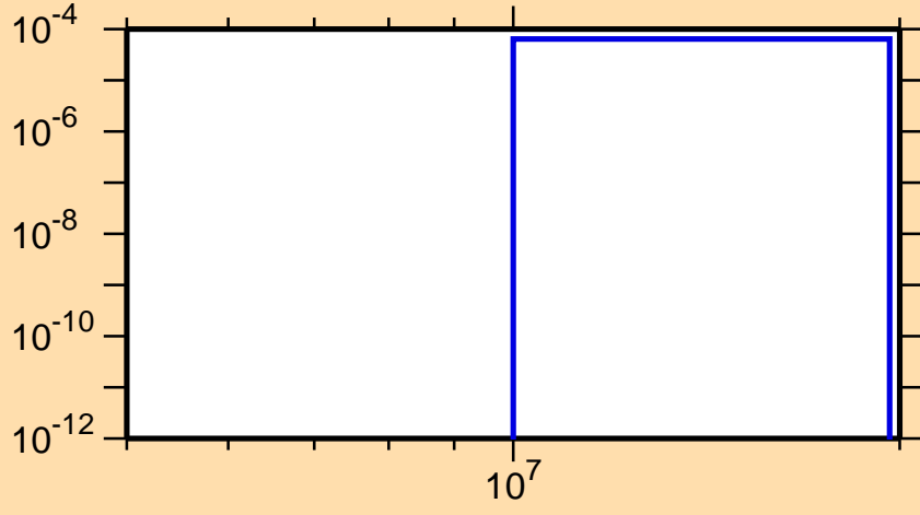
\sigma vs. E for ^{171}\text{Ho}(n,np)
