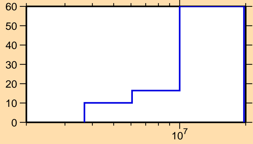
\Delta\sigma/\sigma vs. E for ^{171}\text{Ho}(n,ncont.)
