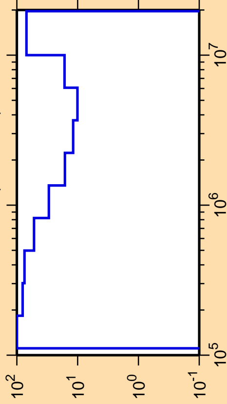
\Delta\sigma/\sigma vs. E for ^{171}\text{Ho}(n,\text{ncont.})
