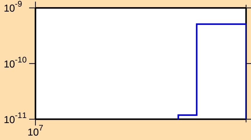
\sigma vs. E for ^{121}\text{La} (mt 34)
