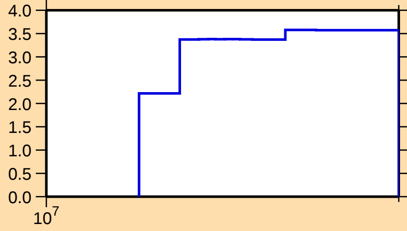
\Delta\sigma/\sigma vs. E for ^{121}\text{La}(n,\text{nonel.})
