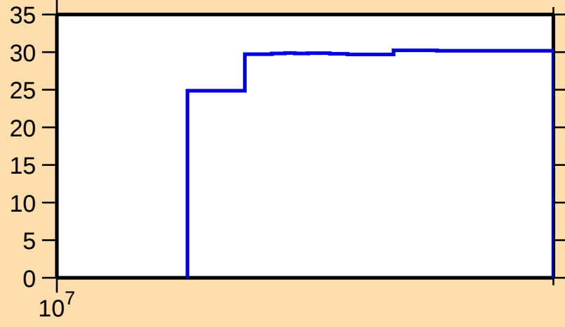
\Delta\sigma/\sigma vs. E for ^{121}\text{La}(n,\text{inel.})
