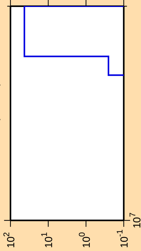
\Delta\sigma/\sigma vs. E for ^{121}\text{La}(n,2n\alpha)
