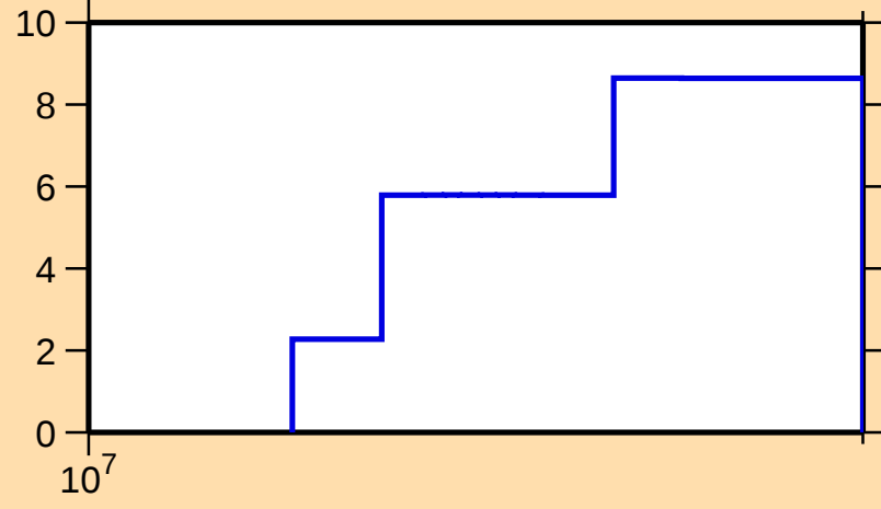
\Delta\sigma/\sigma vs. E for ^{121}\text{La}(n,\text{tot.})
