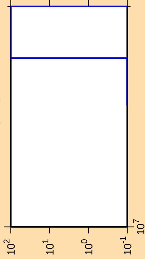
\Delta\sigma/\sigma vs. E for ^{121}\text{La}(n,nt)
