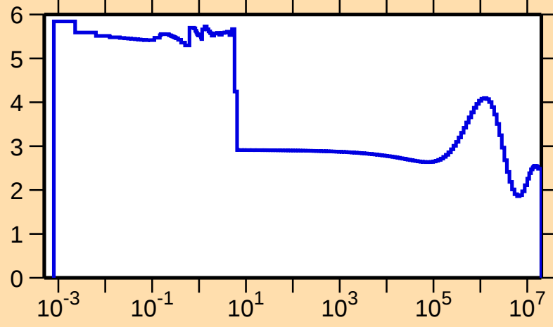
\sigma vs. E for ^{121}\text{La}(n,\text{el.})
