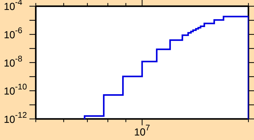
\sigma vs. E for ^{121}\text{La}(\text{mt117})
