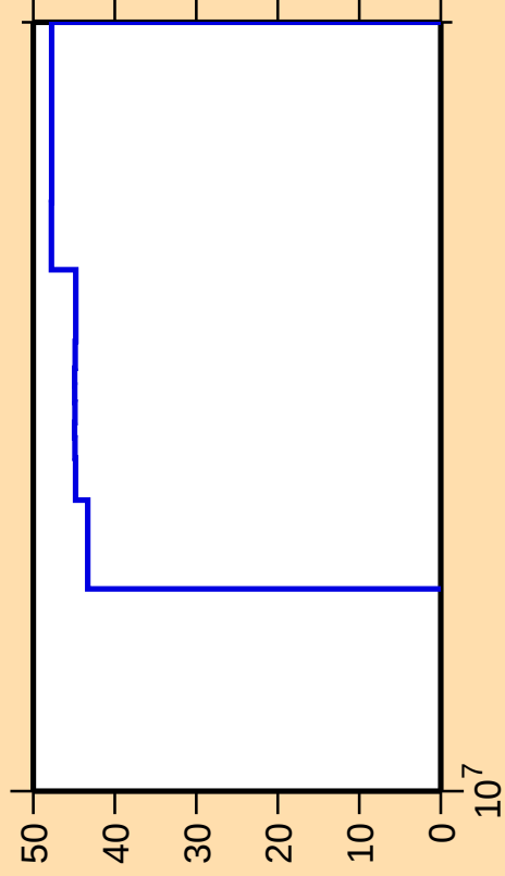
\Delta\sigma/\sigma vs. E for ^{121}\text{La}(n,n_1)
