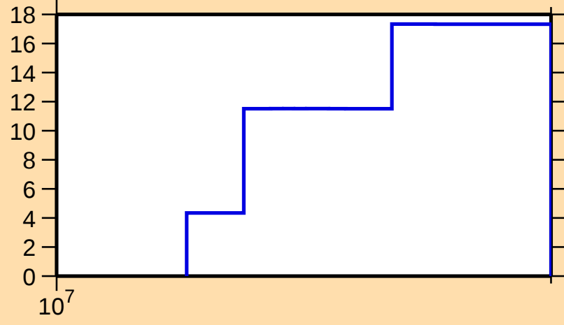
\Delta\sigma/\sigma vs. E for ^{121}\text{La}(n,\text{el.})
