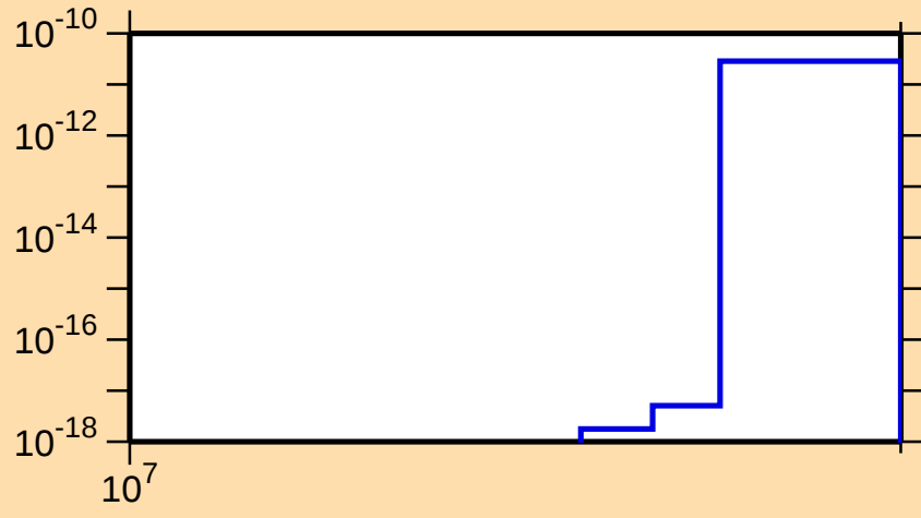
\sigma vs. E for ^{121}\text{La}(n,nt)
