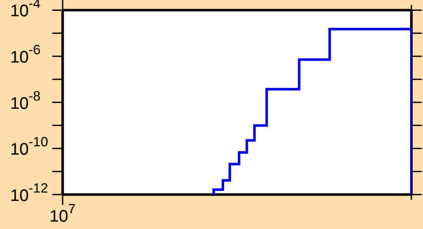
\sigma vs. E for ^{121}\text{La}(n,\text{pt})
