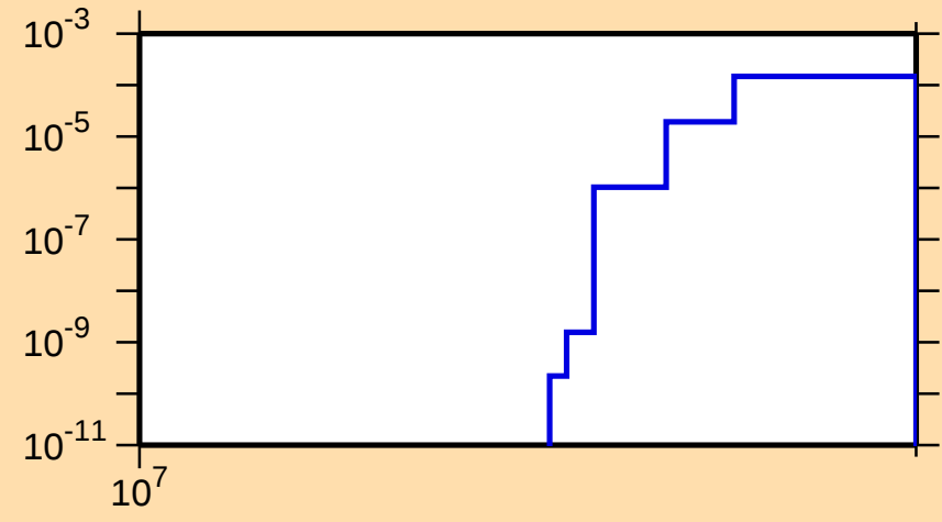
\sigma vs. E for ^{121}\text{La}(n,2np)
