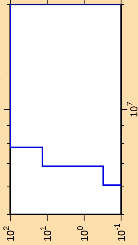
\Delta\sigma/\sigma vs. E for ^{121}\text{La}(\text{mt117})
