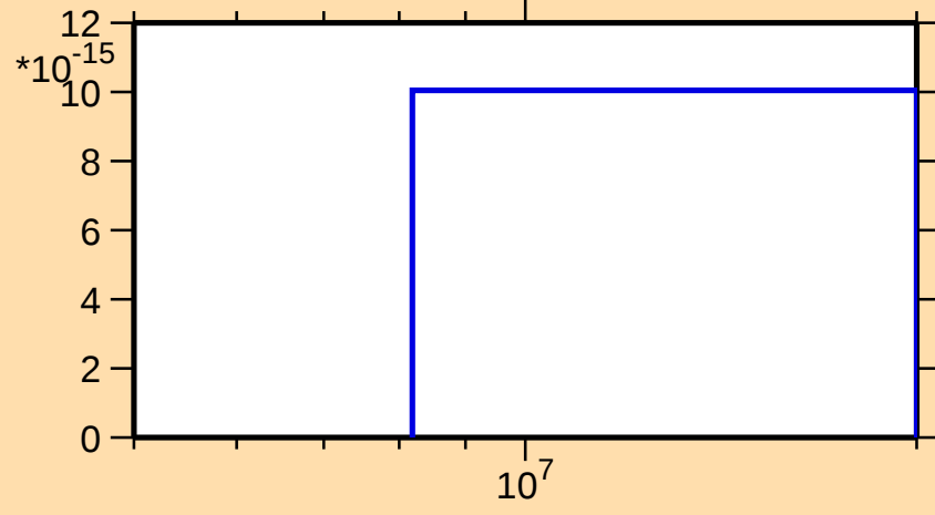
\sigma vs. E for ^{129}\text{La}(\text{mt } 34)
