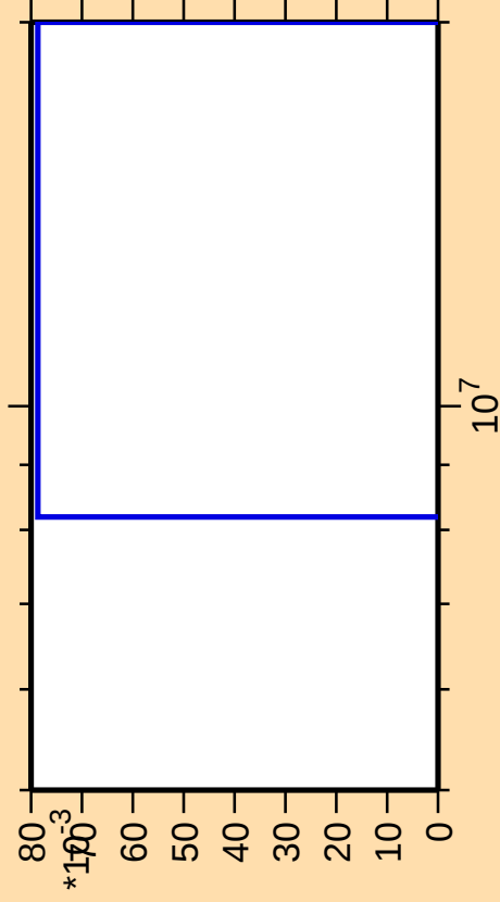
\Delta\sigma/\sigma vs. E for ^{129}\text{La}(\text{mt } 34)
