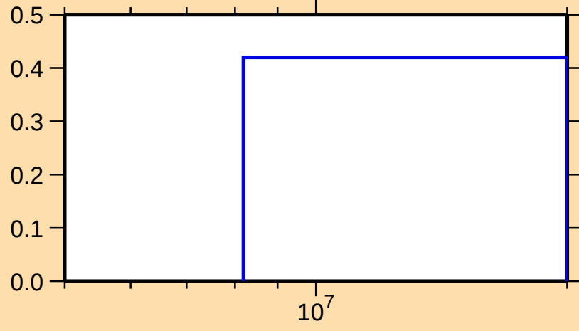
\sigma vs. E for ^{129}\text{La}(n,2n)
