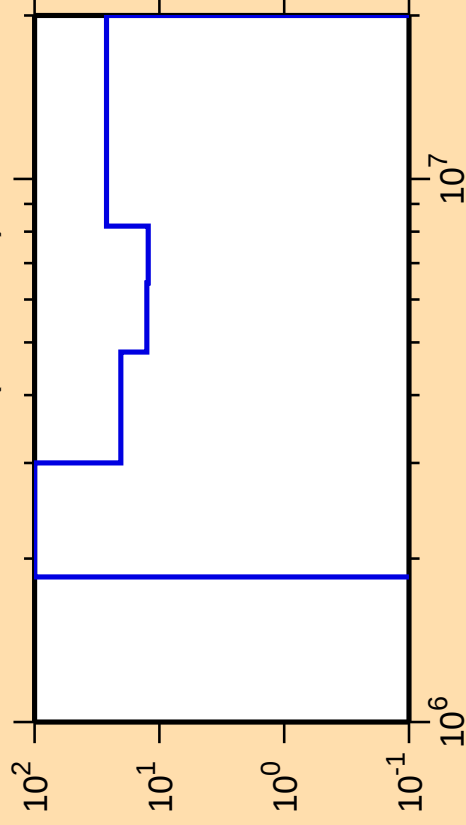
\Delta\sigma/\sigma vs. E for ^{129}\text{La}(n,n\text{cont.})
