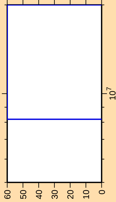
\Delta\sigma/\sigma vs. E for ^{129}\text{La}(\text{mt } 45)
