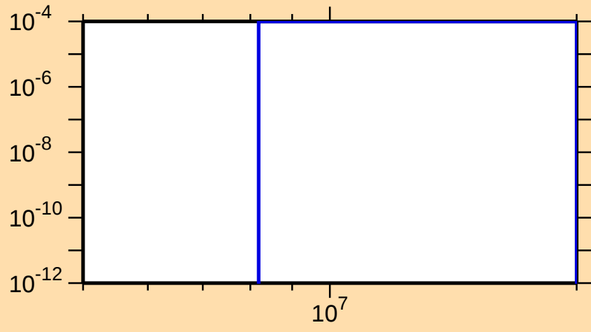
\sigma vs. E for ^{129}\text{La}(n,t)
