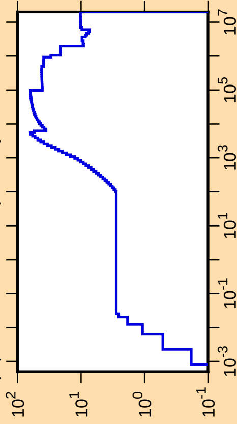
\Delta\mu/\mu vs. E for ^{135}\text{La}(\text{mt251})
