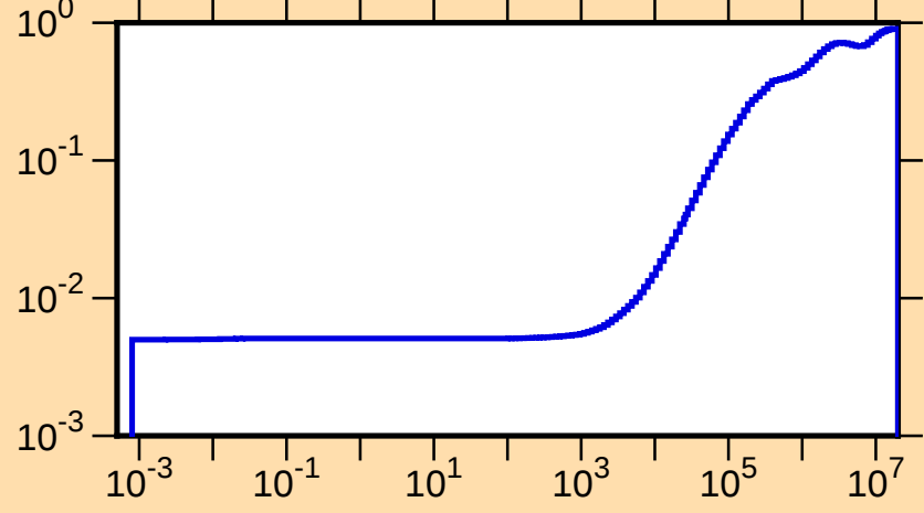
\mu vs. E for ^{135}\text{La}(\text{mt251})
