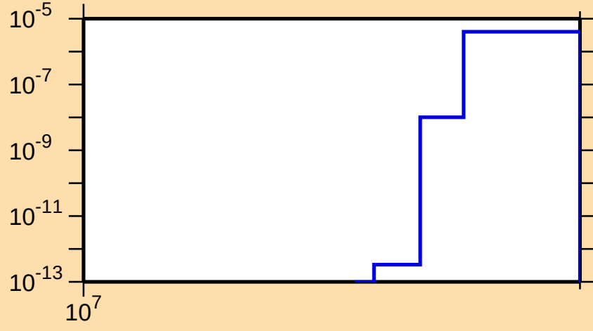
\sigma vs. E for ^{135}\text{La}(n,2np)
