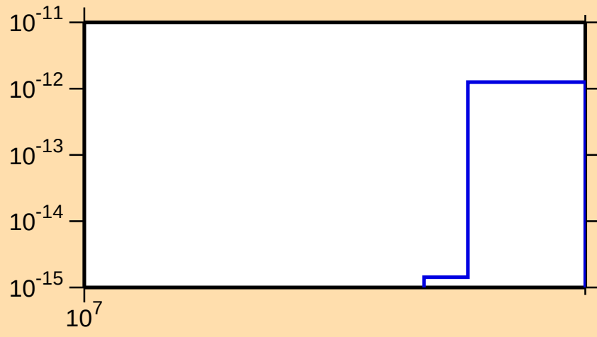
\sigma vs. E for ^{135}\text{La}(n,\text{pd})
