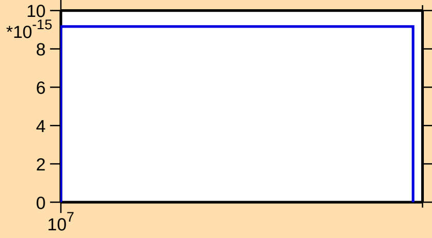
\sigma vs. E for ^{135}\text{La}(n,\text{pd})
