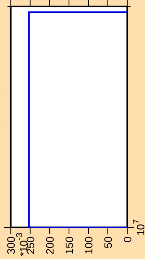
\Delta\sigma/\sigma vs. E for ^{135}\text{La}(\text{mt 45})
