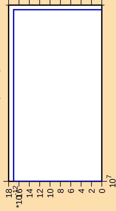
\Delta\sigma/\sigma vs. E for ^{135}\text{La}(\text{mt } 11)
