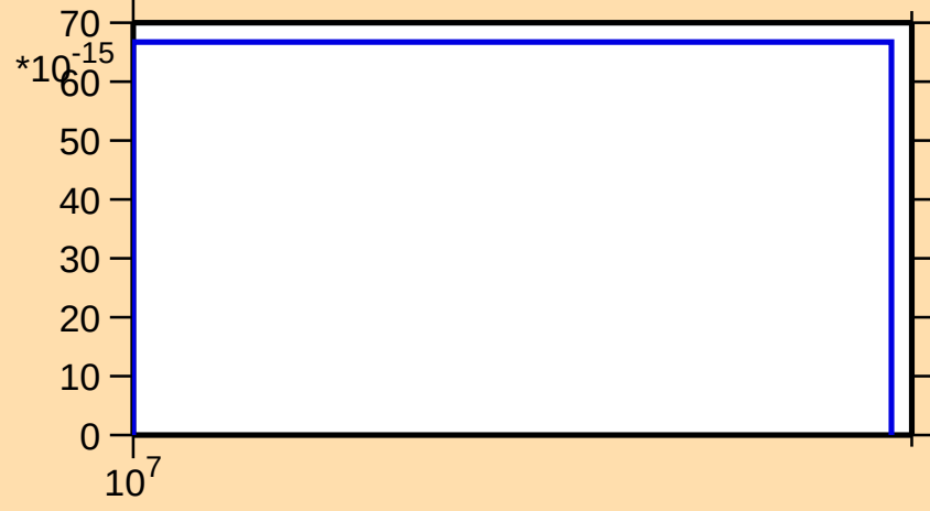
\sigma vs. E for ^{135}\text{La}(\text{mt 45})
