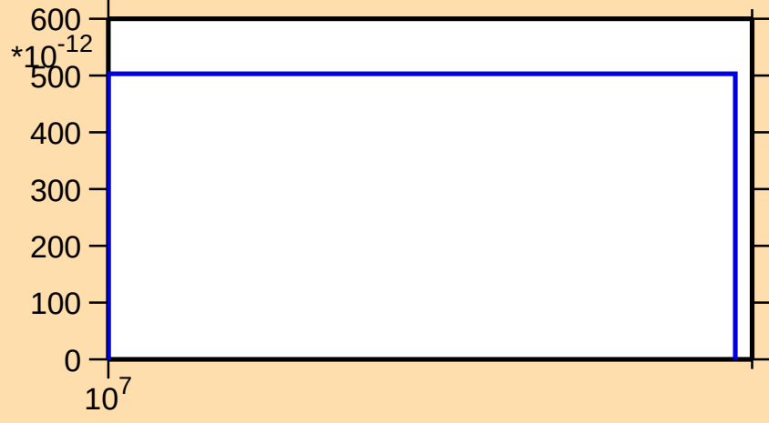
\sigma vs. E for ^{135}\text{La}(n,\text{nt})
