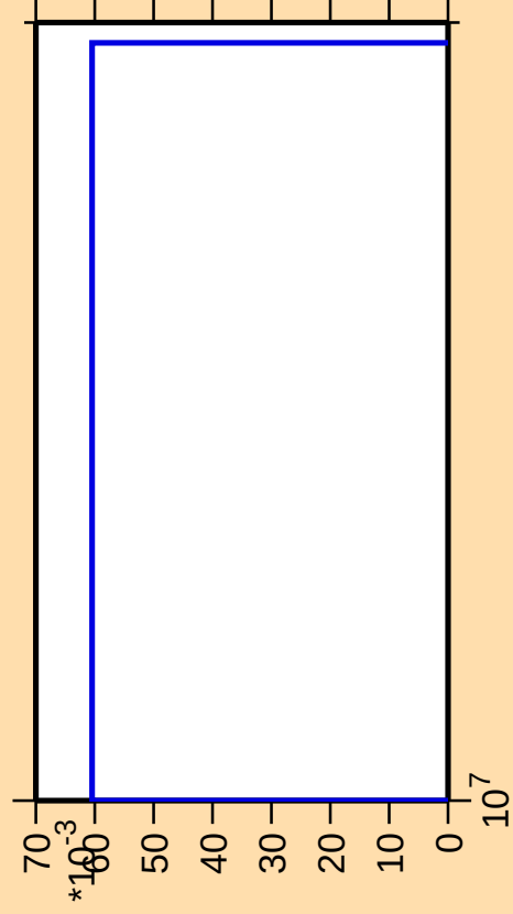
\Delta\sigma/\sigma vs. E for ^{135}\text{La}(n,\text{pd})
