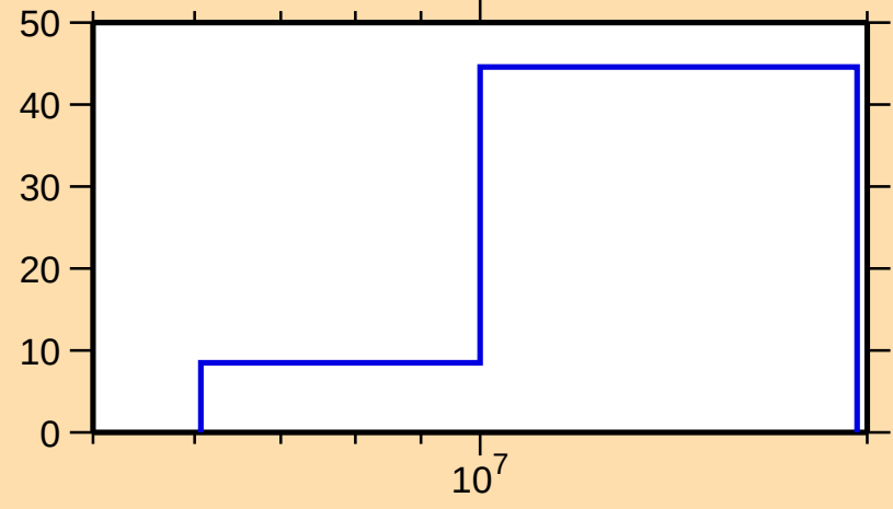
\Delta\sigma/\sigma vs. E for ^{135}\text{La}(n,\text{inel.})
