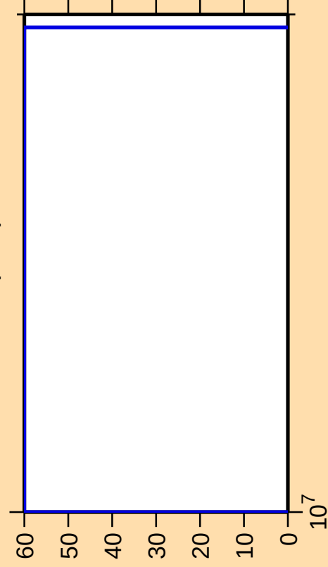
\Delta\sigma/\sigma vs. E for ^{135}\text{La}(n,\text{nt})
