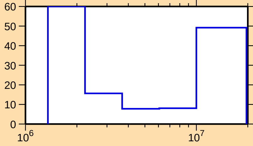
\Delta\sigma/\sigma vs. E for ^{135}\text{La}(n,n\text{cont.})
