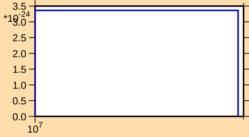
\sigma vs. E for ^{135}\text{La}(\text{mt } 11)
