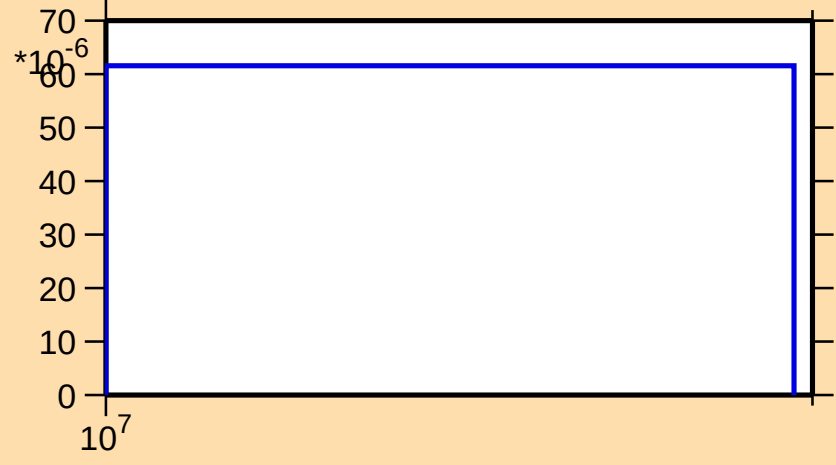
\sigma vs. E for ^{135}\text{La}(n,3n)
