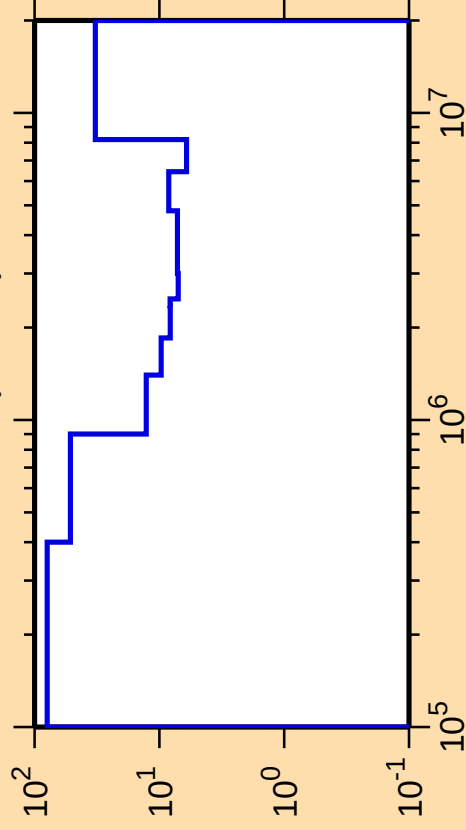
\Delta\sigma/\sigma vs. E for ^{135}\text{La}(n,\text{inel.})
