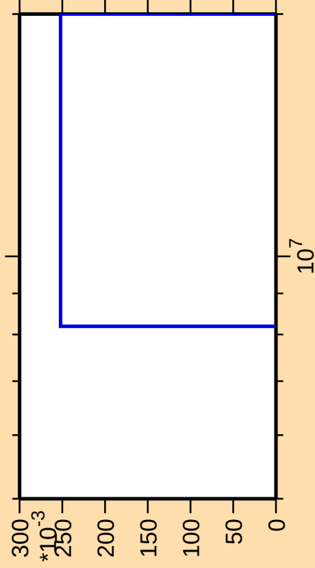
\Delta\sigma/\sigma vs. E for ^{135}\text{La}(\text{mt } 45)
