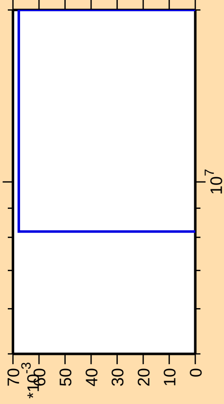
\Delta\sigma/\sigma vs. E for ^{135}\text{La}(n,\text{pd})
