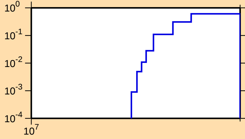
\sigma vs. E for ^{140}\text{La}(n,3n)
