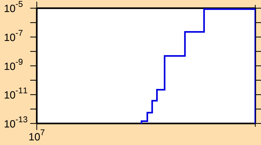
\sigma vs. E for ^{140}\text{La}(n,nt)
