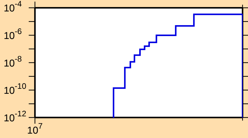
\sigma vs. E for ^{140}\text{La}(n,2np)
