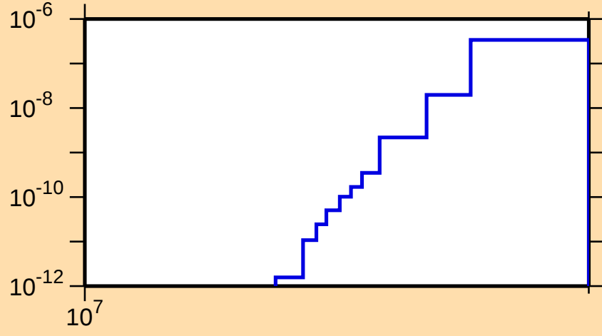
\sigma vs. E for ^{140}\text{La}(n,2n\alpha)
