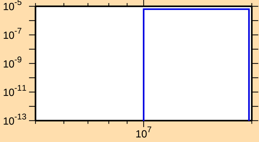
\sigma vs. E for ^{140}\text{La}(n,\text{nd})
