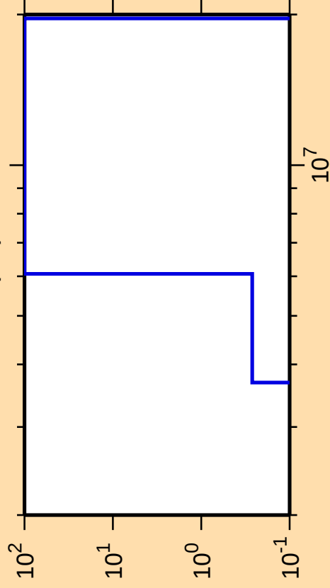
\Delta\sigma/\sigma vs. E for ^{140}\text{La}(n,t)
