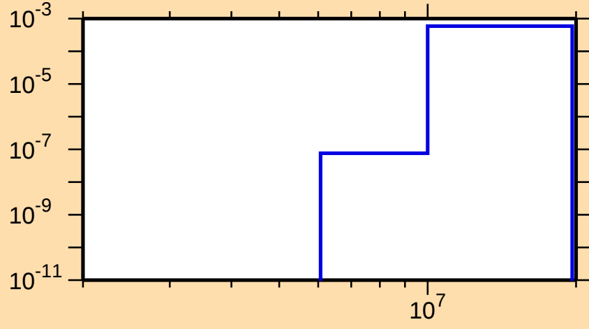
\sigma vs. E for ^{140}\text{La}(n,t)
