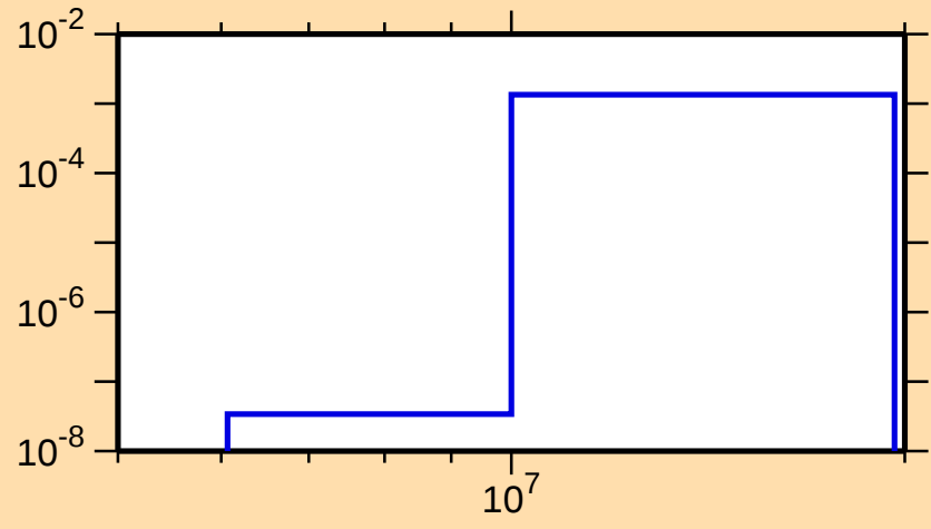
\sigma vs. E for ^{140}\text{La}(n,d)
