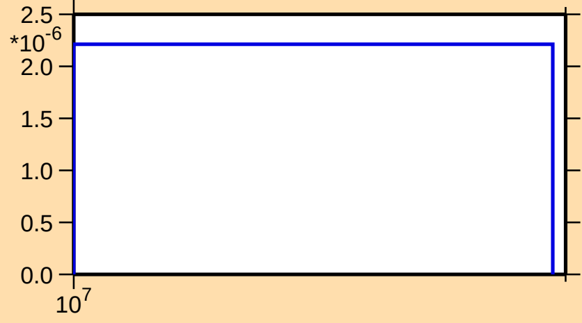
\sigma vs. E for ^{142}\text{La}(n,\text{nd})
