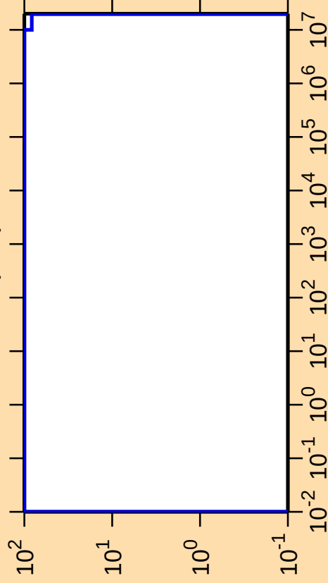
\Delta\sigma/\sigma vs. E for ^{142}\text{La}(n,\alpha)
