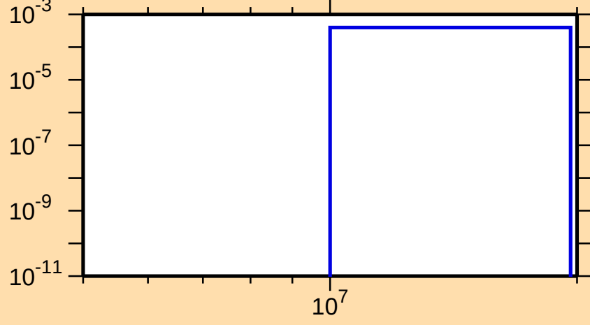
\sigma vs. E for ^{142}\text{La}(n,np)
