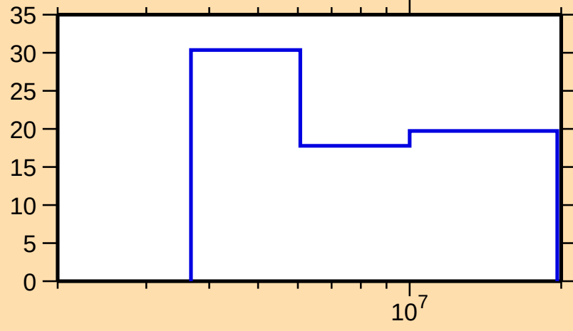
\Delta\sigma/\sigma vs. E for ^{142}\text{La}(n,2n)
