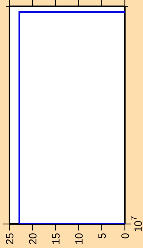
\Delta\sigma/\sigma vs. E for ^{142}\text{La}(n,3n)
