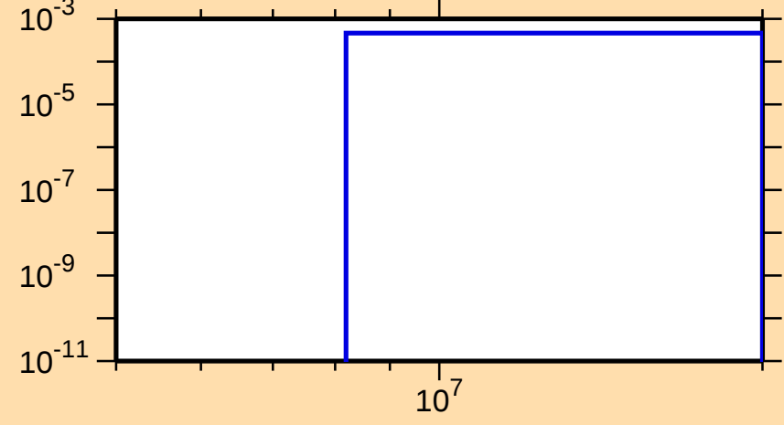
\sigma vs. E for ^{142}\text{La}(n,d)
