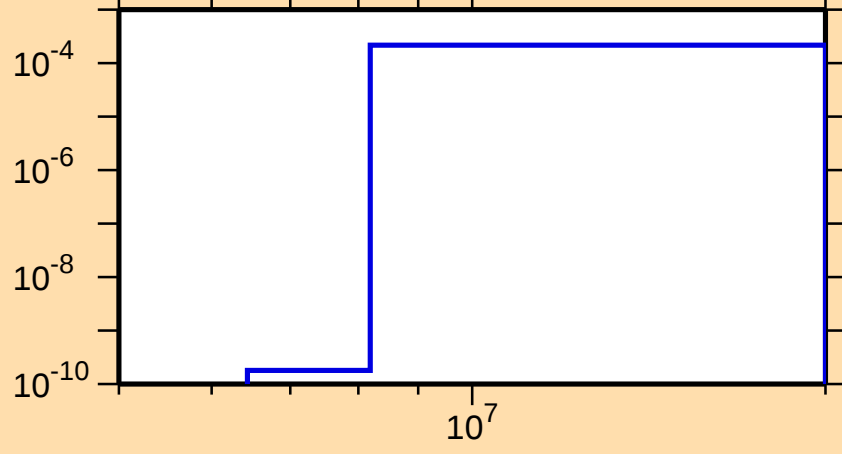
\sigma vs. E for ^{142}\text{La}(n,t)
