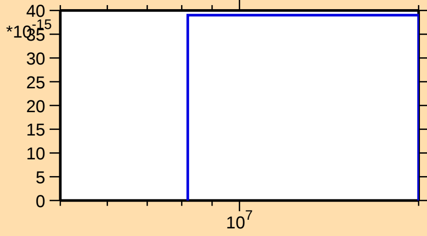
\sigma vs. E for ^{142}\text{La}(\text{mt 11})
