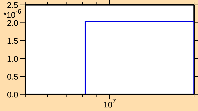
\sigma vs. E for ^{142}\text{La}(n,2n\alpha)
