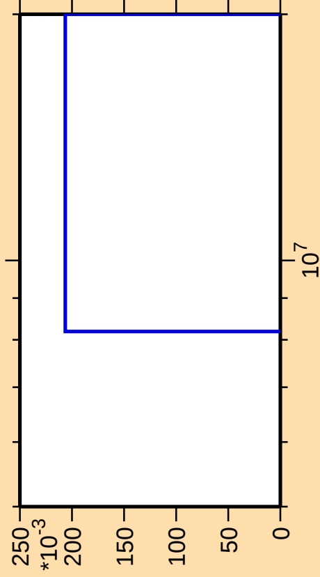
\Delta\sigma/\sigma vs. E for ^{142}\text{La}(\text{mt 11})
