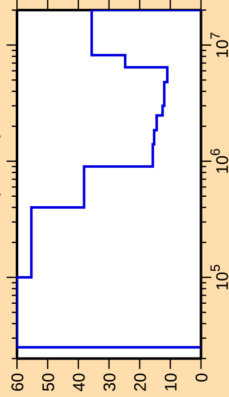
\Delta\sigma/\sigma vs. E for ^{142}\text{La}(n,\text{inel.})
