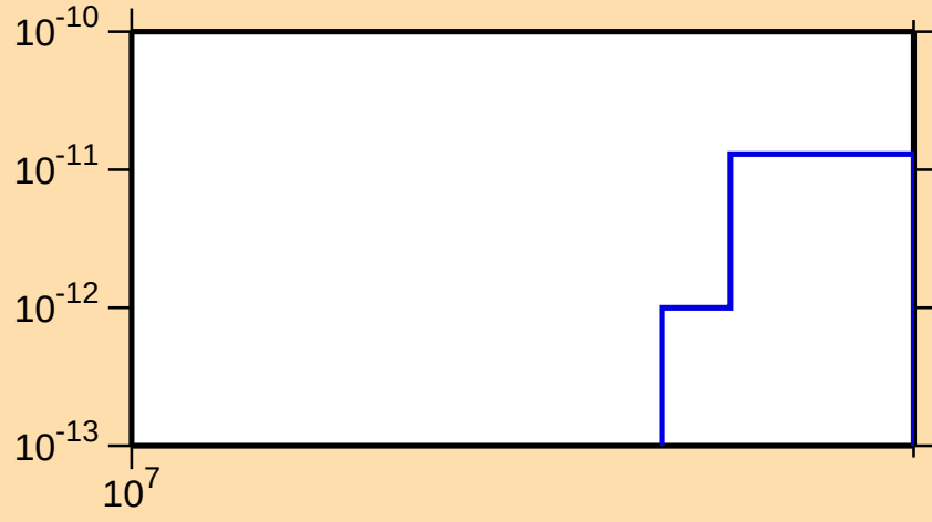
\sigma vs. E for ^{254}\text{Lw}(n,\text{pt})
