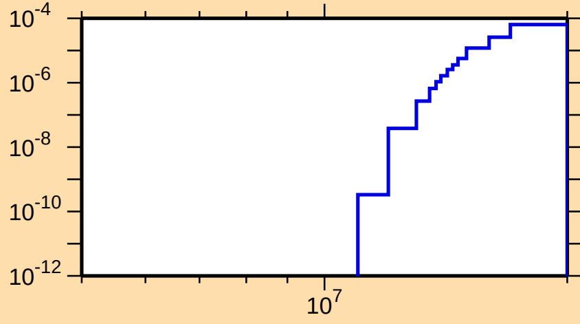
\sigma vs. E for ^{254}\text{Lw}(n,2np)
