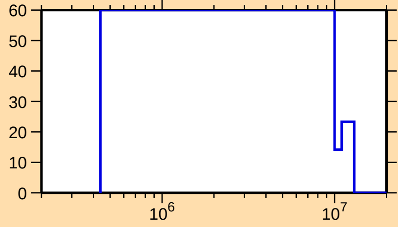
\Delta\sigma/\sigma vs. E for ^{254}\text{Lw}(n, n_1)
