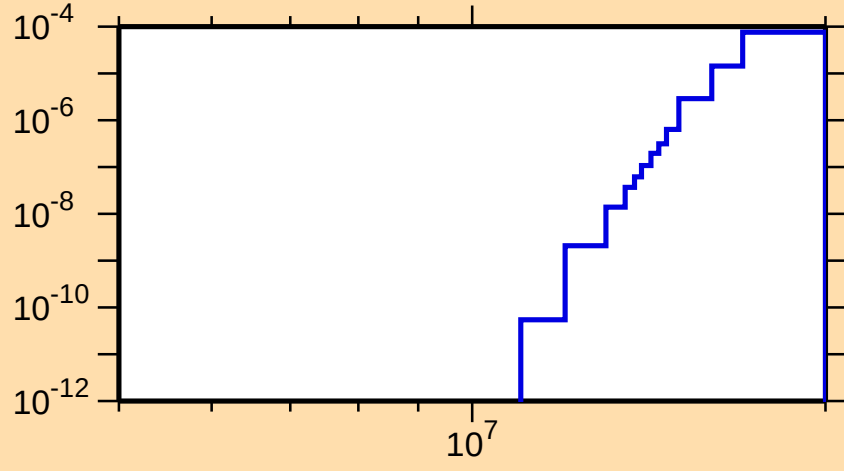
\sigma vs. E for ^{254}\text{Lw}(n,nd)
