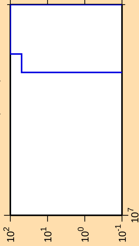
\Delta\sigma/\sigma vs. E for ^{254}\text{Lw}(\text{mt } 34)
