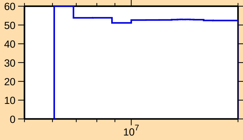
\Delta\sigma/\sigma vs. E for ^{254}\text{Lw}(n,\text{inel.})
