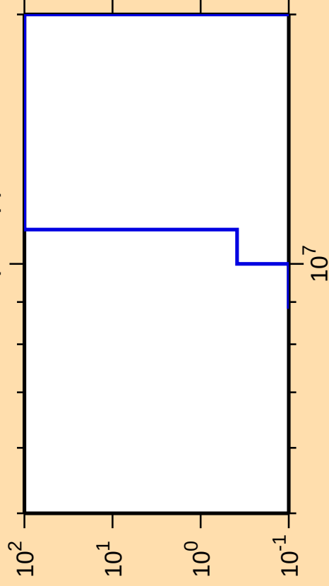
\Delta\sigma/\sigma vs. E for ^{254}\text{Lw}(n,2np)
