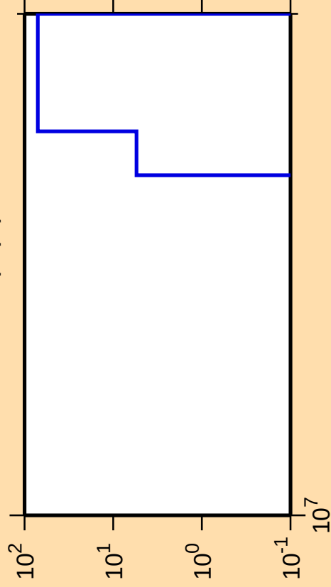
\Delta\sigma/\sigma vs. E for ^{254}\text{Lw}(n,\text{pt})
