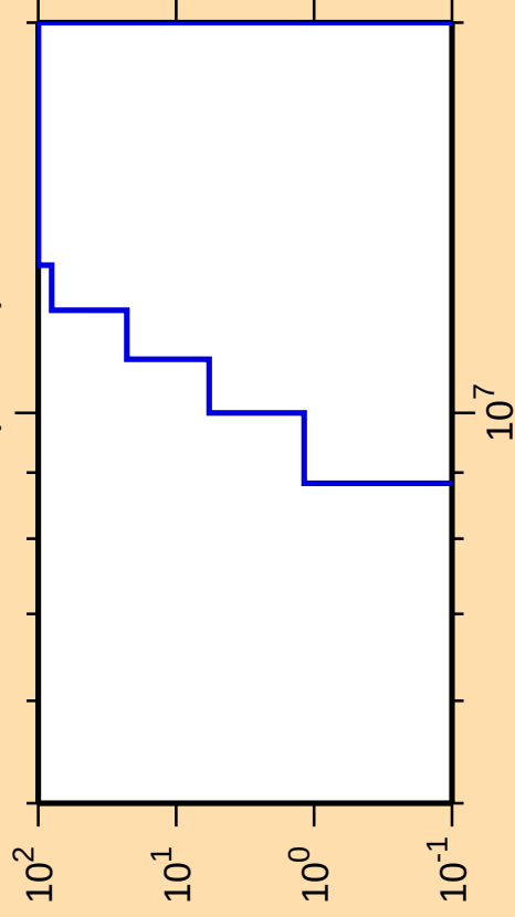
\Delta\sigma/\sigma vs. E for ^{254}\text{Lw(mt 45)}
