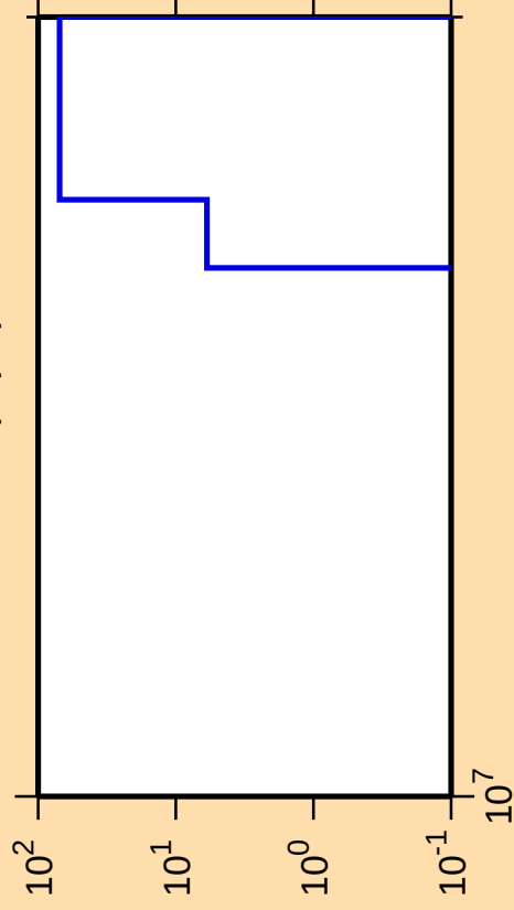
\Delta\sigma/\sigma vs. E for ^{254}\text{Lw}(n,\text{pd})
