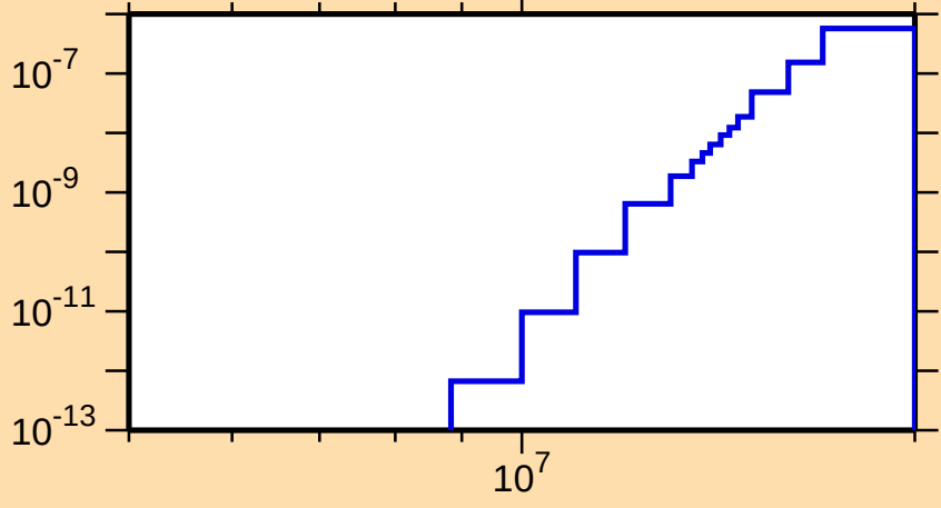
\sigma vs. E for ^{254}\text{Lw}(n,\text{He3})
