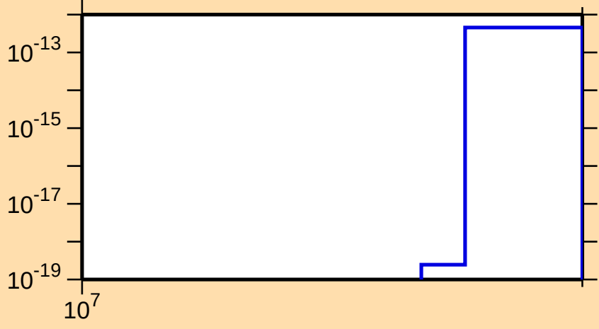
\sigma vs. E for ^{254}\text{Lw(mt 11)}
