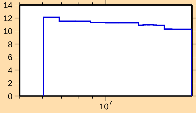
\Delta\sigma/\sigma vs. E for ^{254}\text{Lw}(n,\text{nonel.})
