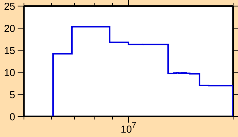
\Delta\sigma/\sigma vs. E for ^{254}\text{Lw}(n,\text{tot.})
