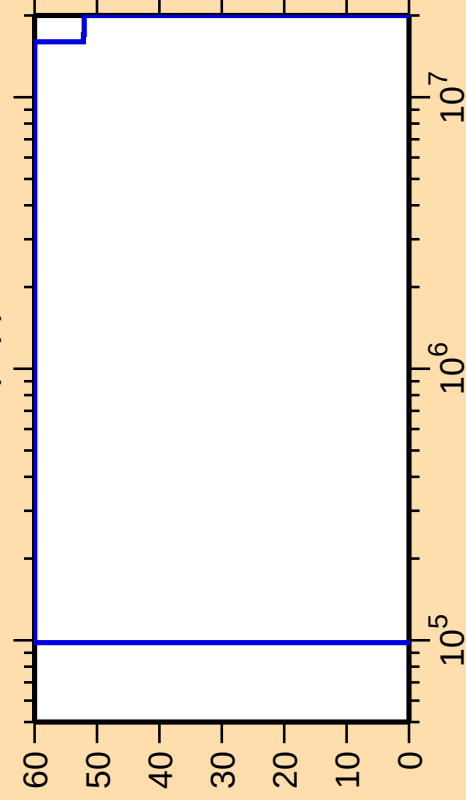
\Delta\sigma/\sigma vs. E for ^{254}\text{Lw}(n,p)
