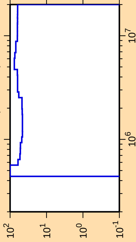
\Delta\sigma/\sigma vs. E for ^{254}\text{Lw}(n, n_{\text{cont}})
