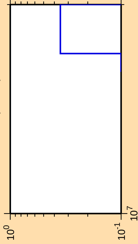
\Delta\sigma/\sigma vs. E for ^{254}\text{Lw}(\text{mt } 42)
