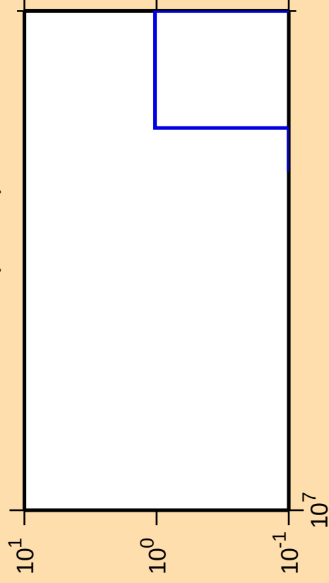
\Delta\sigma/\sigma vs. E for ^{254}\text{Lw(mt 11)}
