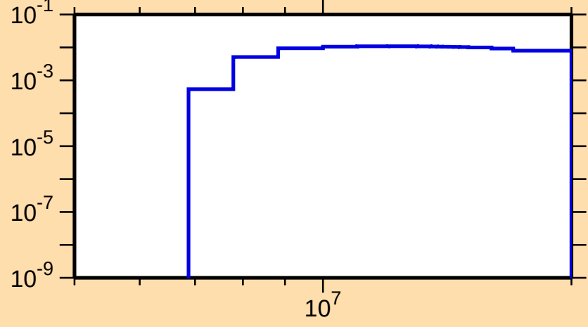
\sigma vs. E for ^{254}\text{Lw}(n,2n\alpha)
