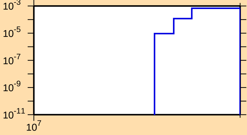
\sigma vs. E for ^{254}\text{Lw}(n,3n\alpha)
