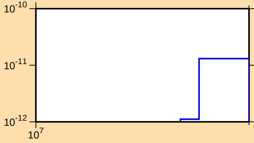
\sigma vs. E for ^{254}\text{Lw}(n,\text{pd})
