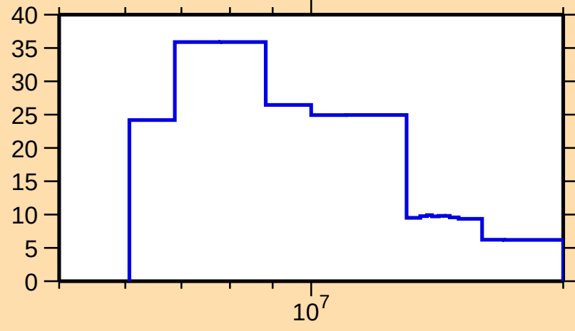
\Delta\sigma/\sigma vs. E for ^{254}\text{Lw}(n,\text{el.})
