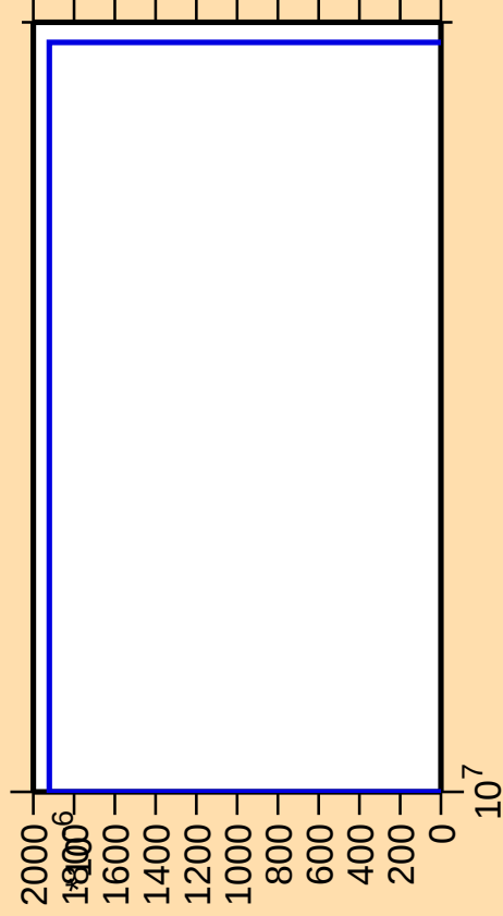
\Delta\sigma/\sigma vs. E for ^{254}\text{Lw(mt 42)}
