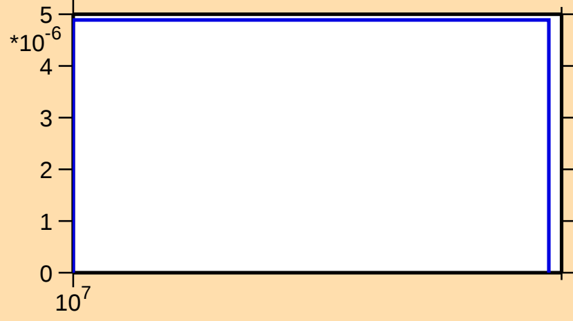
\sigma vs. E for ^{254}\text{Lw}(n,2np)
