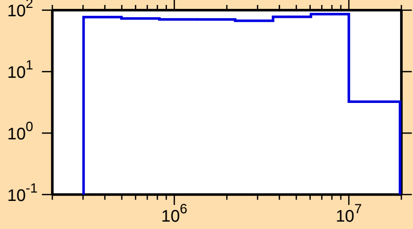
\Delta\sigma/\sigma vs. E for ^{254}\text{Lw}(n,n_1)
