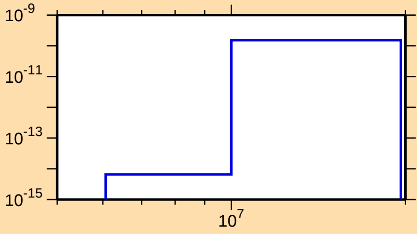
\sigma vs. E for ^{254}\text{Lw}(\text{mt117})
