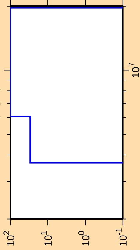
\Delta\sigma/\sigma vs. E for ^{254}\text{Lw}(n,p\alpha)
