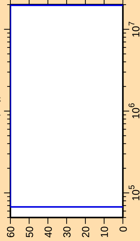
\Delta\sigma/\sigma vs. E for ^{254}\text{Lw}(n,\gamma)
