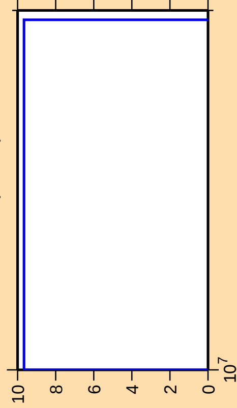
\Delta\sigma/\sigma vs. E for ^{254}\text{Lw(mt 34)}
