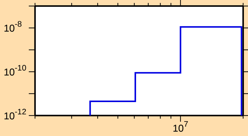
\sigma vs. E for ^{254}\text{Lw}(n,p\alpha)
