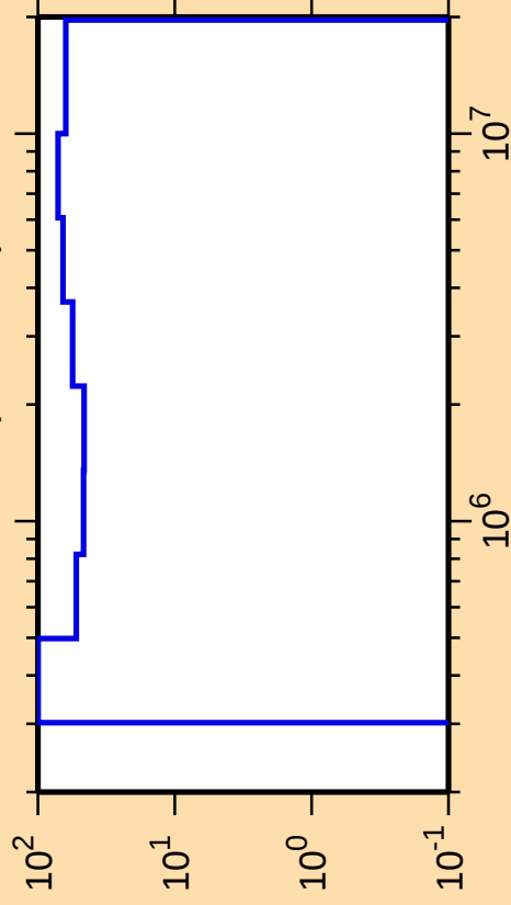
\Delta\sigma/\sigma vs. E for ^{254}\text{Lw}(n,\text{ncont.})
