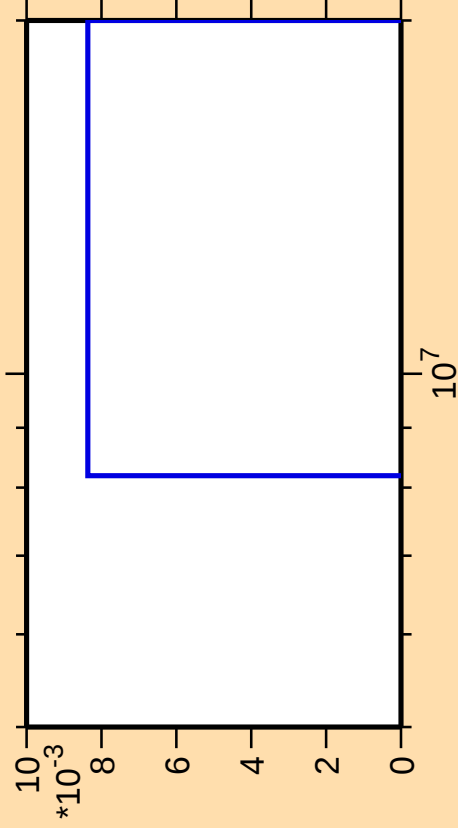
\Delta\sigma/\sigma vs. E for ^{254}\text{Lw(mt 11)}
