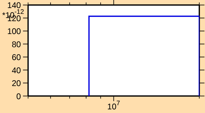
\sigma vs. E for ^{254}\text{Lw(mt117)}
