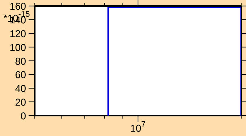
\sigma vs. E for ^{254}\text{Lw}(n,\text{pt})
