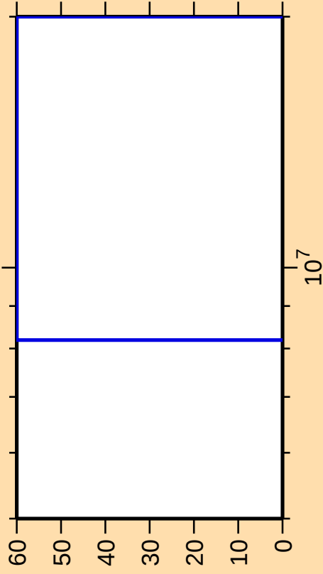
\Delta\sigma/\sigma vs. E for ^{254}\text{Lw(mt117)}
