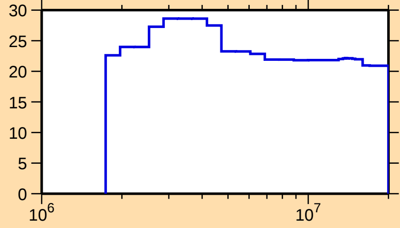
\Delta\sigma/\sigma vs. E for ^{255}\text{Lw}(n,n\text{onel.})
