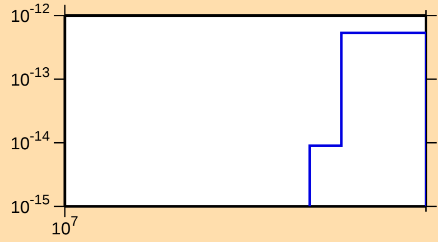
\sigma vs. E for ^{255}\text{Lw}(n,\text{pt})
