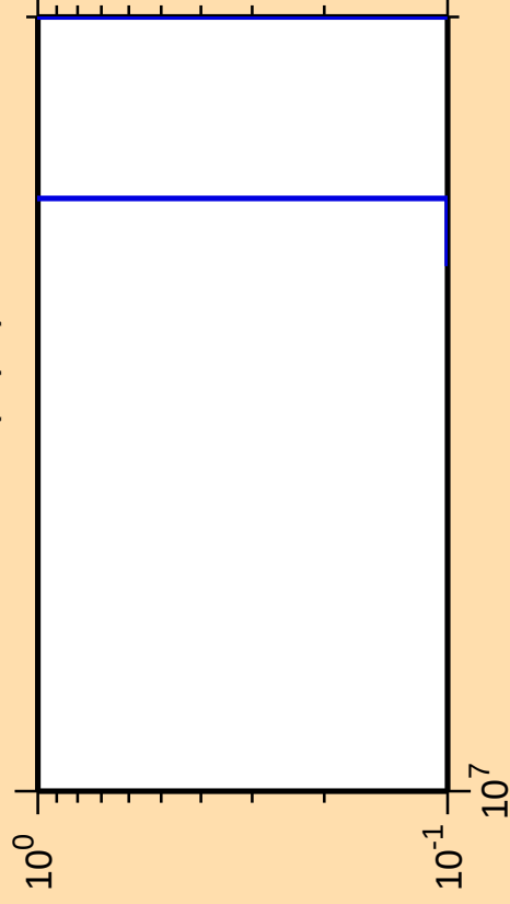
\Delta\sigma/\sigma vs. E for ^{255}\text{Lw}(n,\text{pd})
