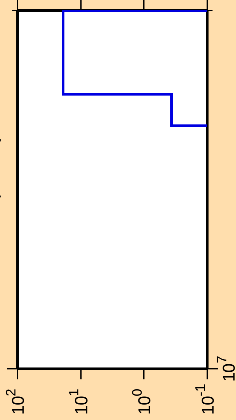
\Delta\sigma/\sigma vs. E for ^{255}\text{Lw(mt 34)}
