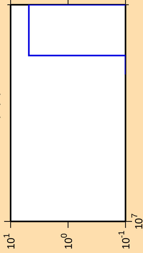
\Delta\sigma/\sigma vs. E for ^{255}\text{Lw}(n,\text{pt})
