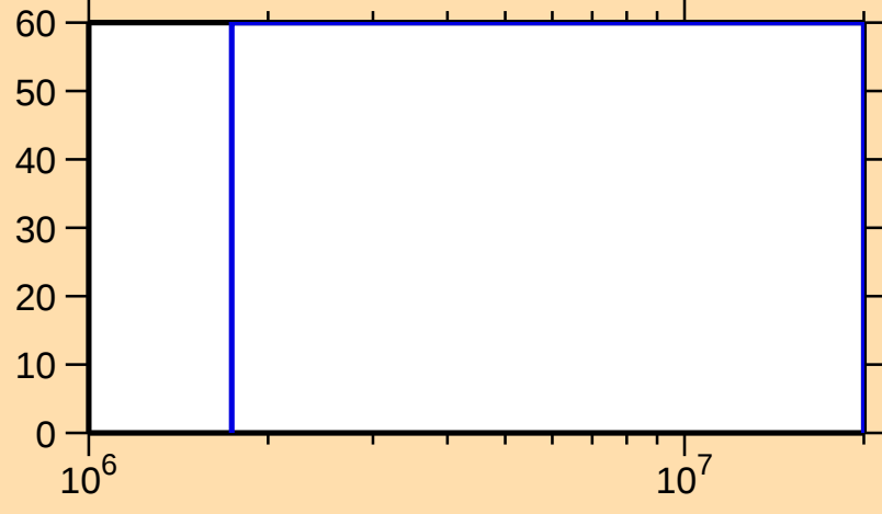
\Delta\sigma/\sigma vs. E for ^{255}\text{Lw}(n,\text{ncont.})
