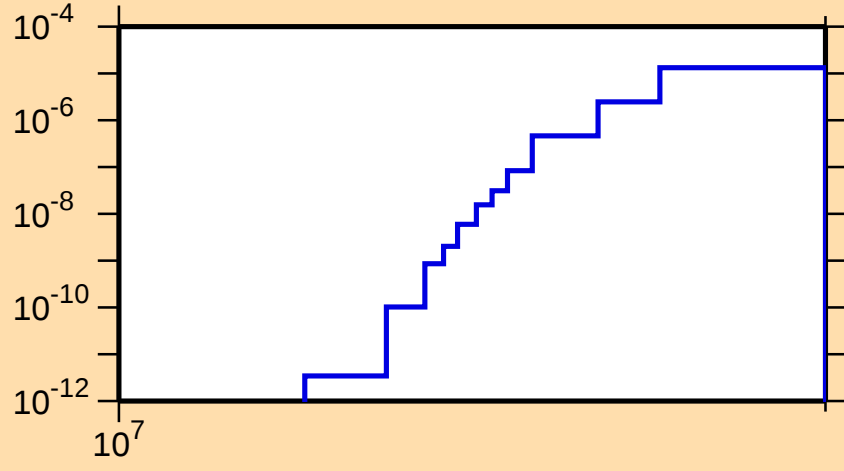
\sigma vs. E for ^{255}\text{Lw}(n,2np)
