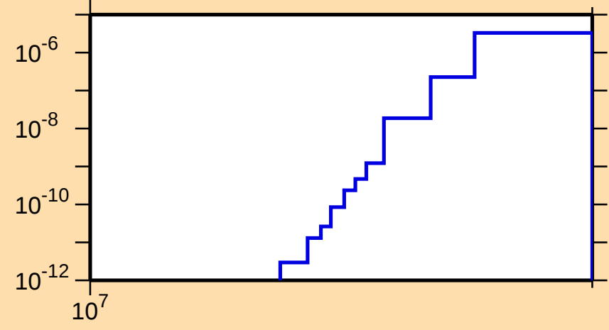
\sigma vs. E for ^{255}\text{Lw}(n,nt)
