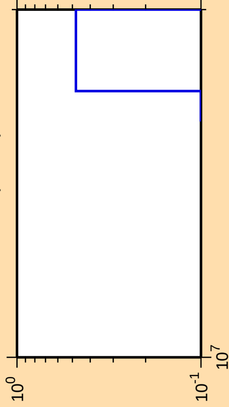
\Delta\sigma/\sigma vs. E for ^{255}\text{Lw(mt 11)}
