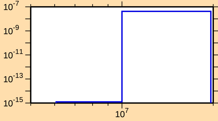
\sigma vs. E for ^{255}\text{Lw(mt 45)}
