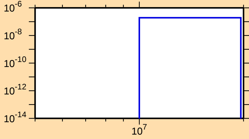
\sigma vs. E for ^{255}\text{Lw}(n,nd)
