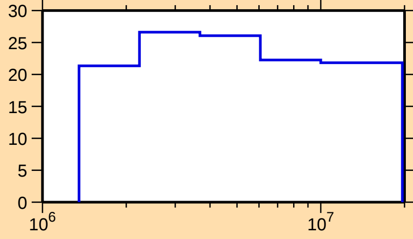
\Delta\sigma/\sigma vs. E for ^{255}\text{Lw}(n,n\text{oncl.})
