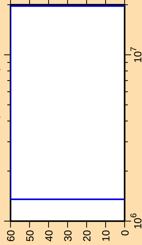
\Delta\sigma/\sigma vs. E for ^{255}\text{Lw}(n,\text{ncont.})
