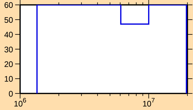
\Delta\sigma/\sigma vs. E for ^{255}\text{Lw}(n,n_1)
