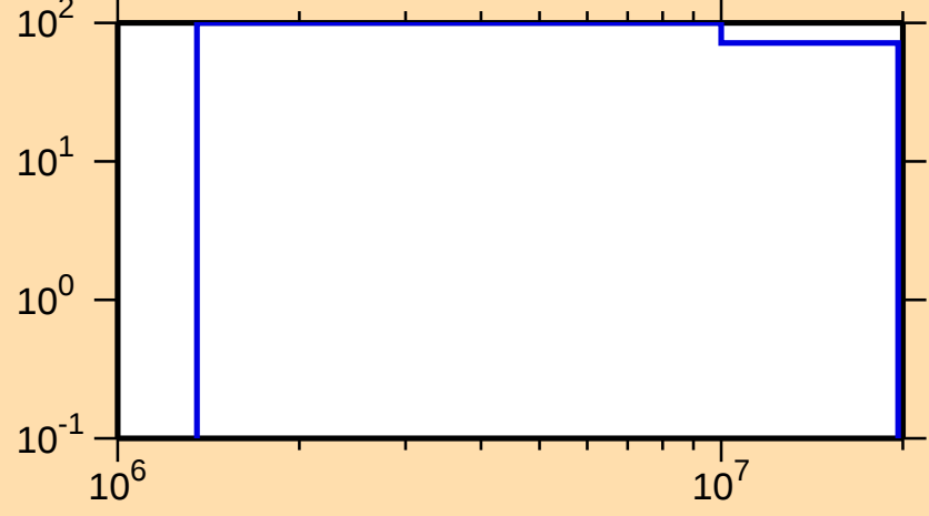
\Delta\sigma/\sigma vs. E for ^{255}\text{Lw}(n,\text{f})
