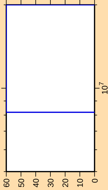
\Delta\sigma/\sigma vs. E for ^{255}\text{Lw(mt 45)}
