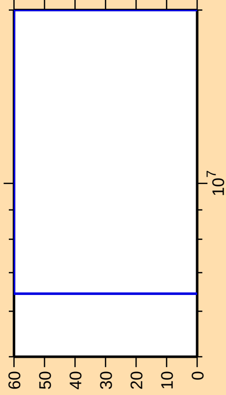
\Delta\sigma/\sigma vs. E for ^{255}\text{Lw}(n,\gamma)
