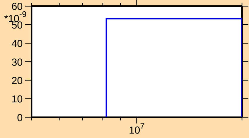
\sigma vs. E for ^{255}\text{Lw(mt117)}
