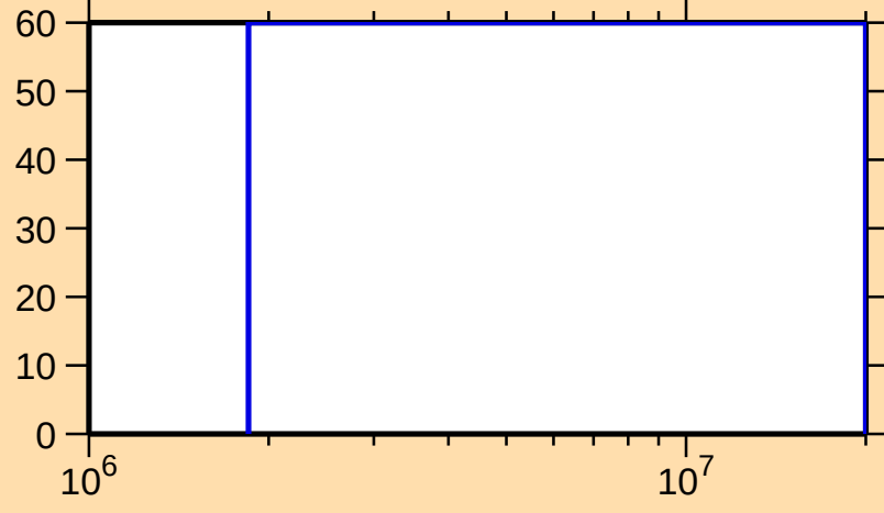
\Delta\sigma/\sigma vs. E for ^{255}\text{Lw}(n,\text{ncont.})
