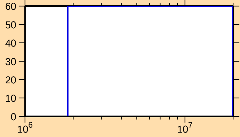
\Delta\sigma/\sigma vs. E for ^{255}\text{Lw}(n,ncont.)
