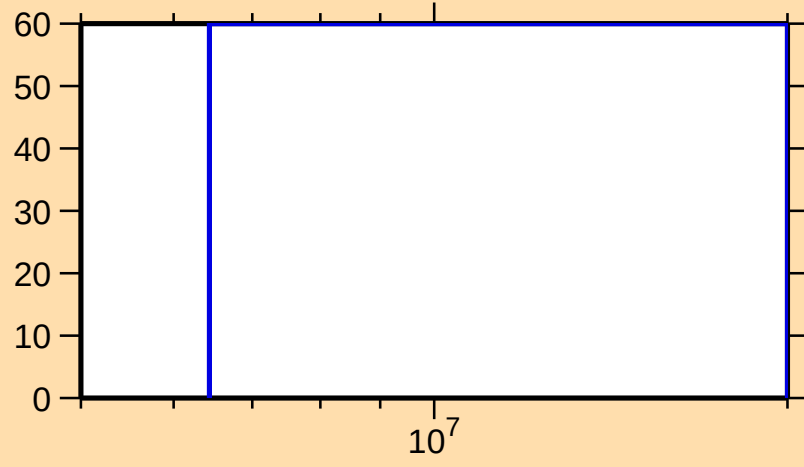
\Delta\sigma/\sigma vs. E for ^{255}\text{Lw}(n,2n)
