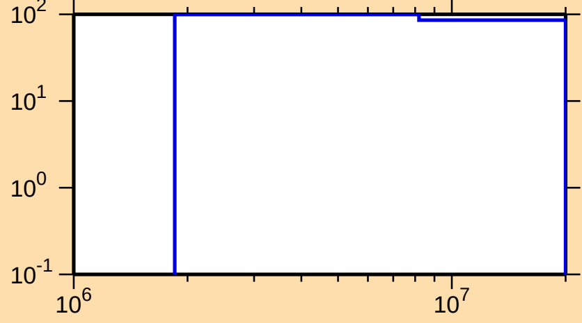
\Delta\sigma/\sigma vs. E for ^{255}\text{Lw}(n,f)
