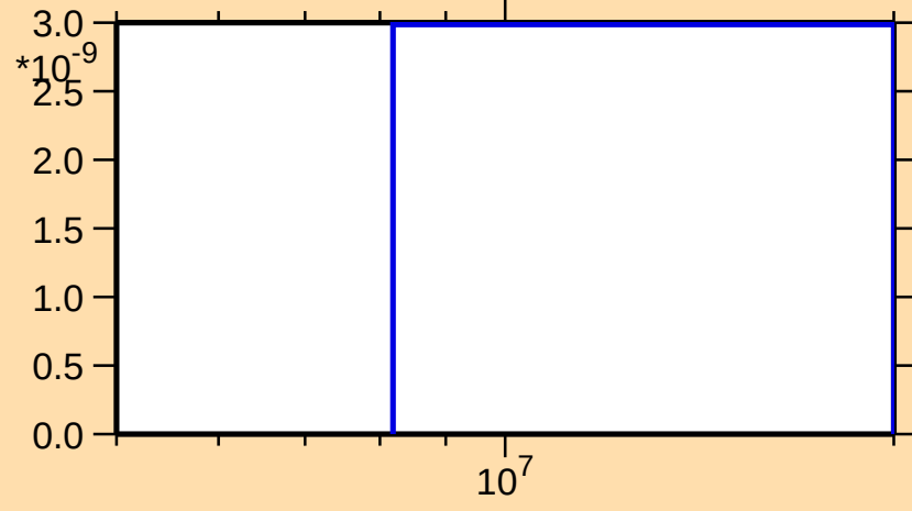
\sigma vs. E for ^{255}\text{Lw}(n,\text{He3})
