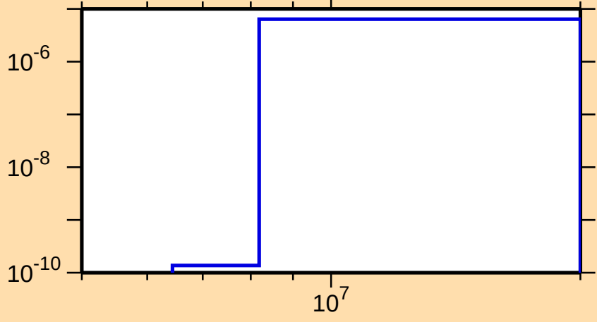
\sigma vs. E for ^{255}\text{Lw}(n,2n\alpha)
