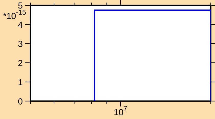
\sigma vs. E for ^{255}\text{Lw}(n,pt)
