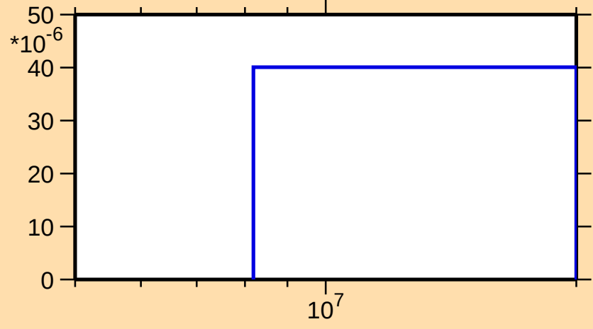
\sigma vs. E for ^{255}\text{Lw}(n,3n\alpha)
