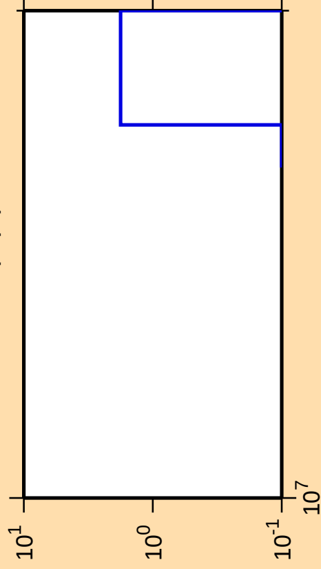
\Delta\sigma/\sigma vs. E for ^{255}\text{Lw}(n,pt)
