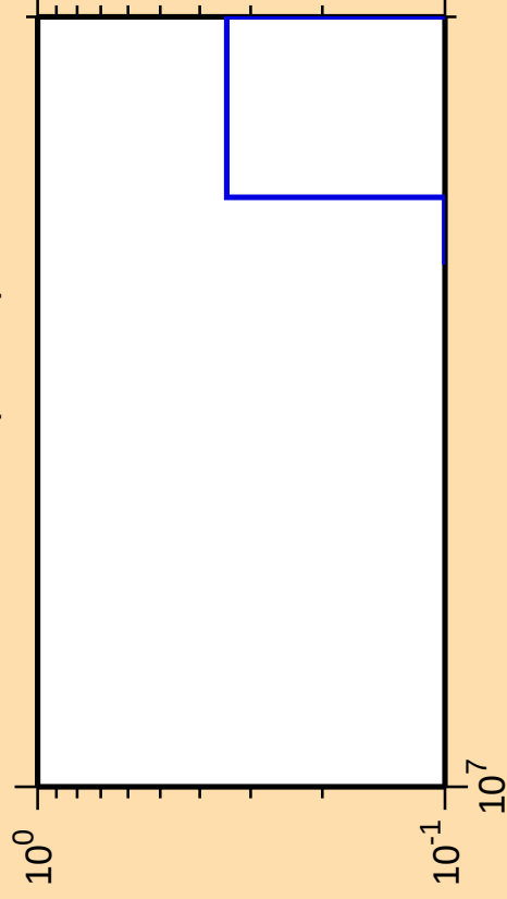
\Delta\sigma/\sigma vs. E for ^{255}\text{Lw(mt 42)}
