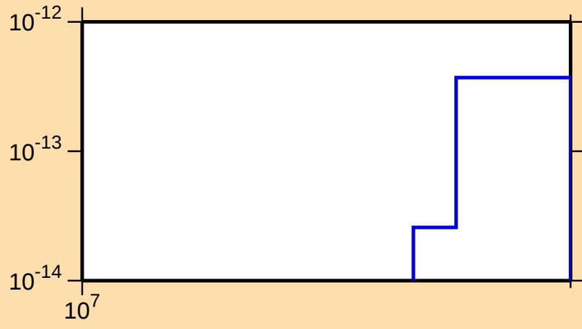
\sigma vs. E for ^{255}\text{Lw}(n,\text{pd})
