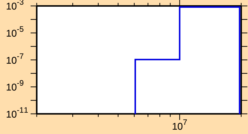
\sigma vs. E for ^{255}\text{Lw}(n,d)
