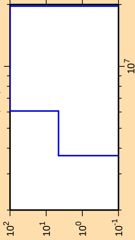
\Delta\sigma/\sigma vs. E for ^{255}\text{Lw}(n,d)
