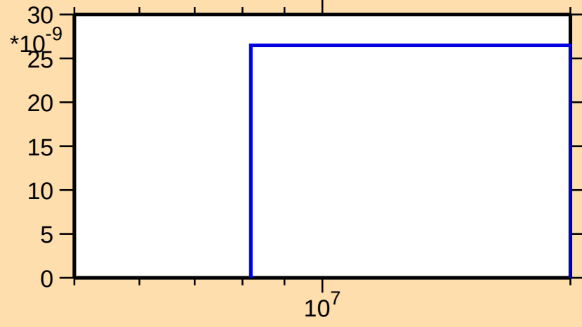
\sigma vs. E for ^{255}\text{Lw(mt 45)}
