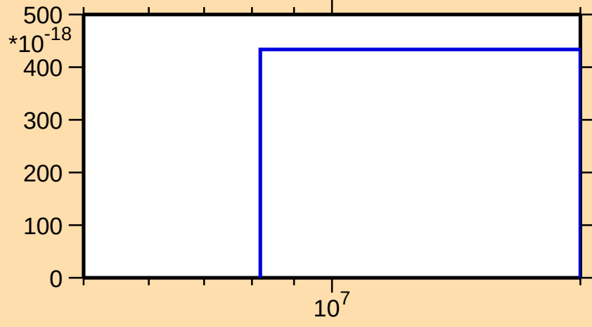
\sigma vs. E for ^{255}\text{Lw(mt 42)}
