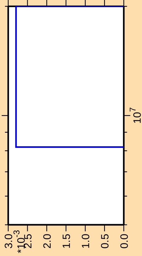
\Delta\sigma/\sigma vs. E for ^{255}\text{Lw(mt 42)}
