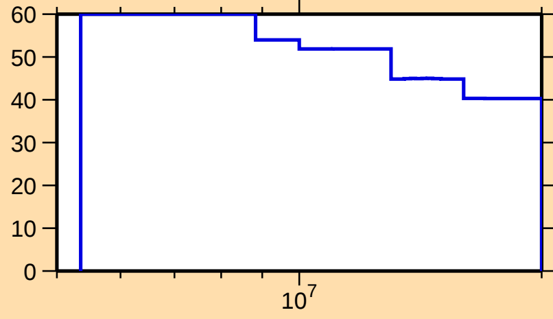
\Delta\sigma/\sigma vs. E for ^{258}\text{Lw}(n,2n)
