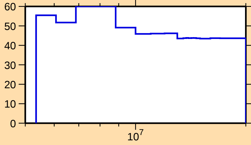
\Delta\sigma/\sigma vs. E for ^{258}\text{Lw}(n,\text{inel.})
