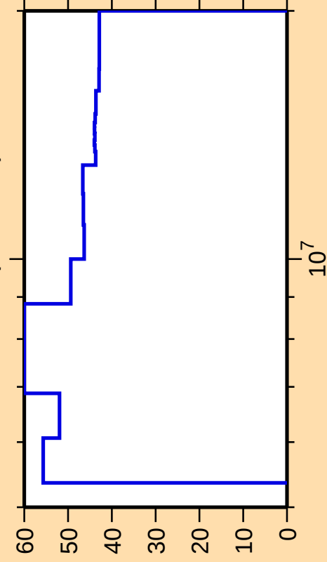
\Delta\sigma/\sigma vs. E for ^{258}\text{Lw}(n,n\text{cont.})
