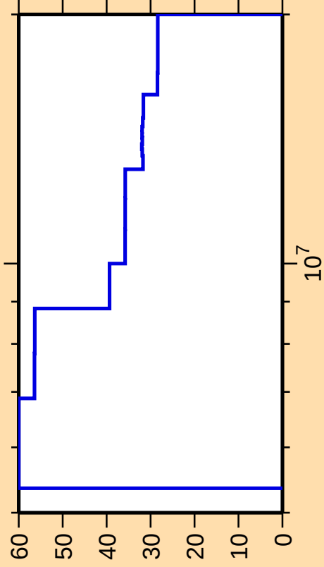
\Delta\sigma/\sigma vs. E for ^{258}\text{Lw}(n,f)
