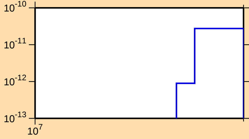
\sigma vs. E for ^{258}\text{Lw(mt 34)}
