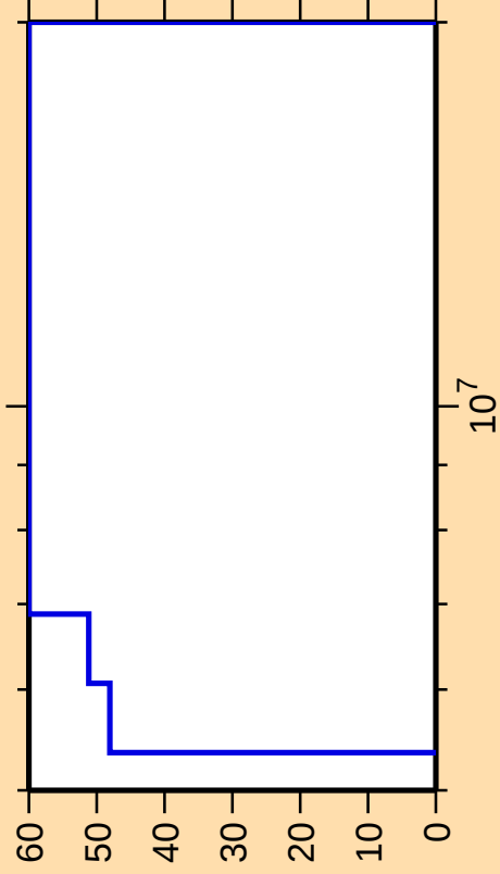
\Delta\sigma/\sigma vs. E for ^{258}\text{Lw}(n,\gamma)
