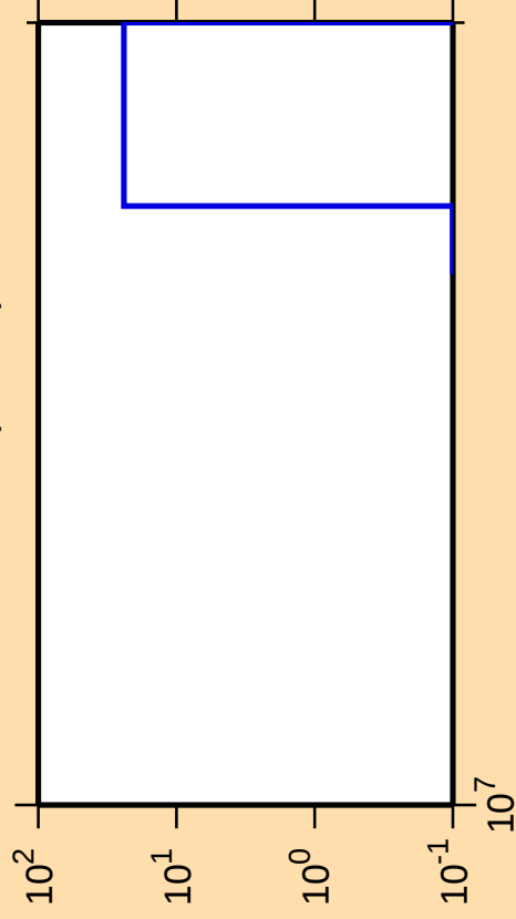
\Delta\sigma/\sigma vs. E for ^{258}\text{Lw(mt 11)}
