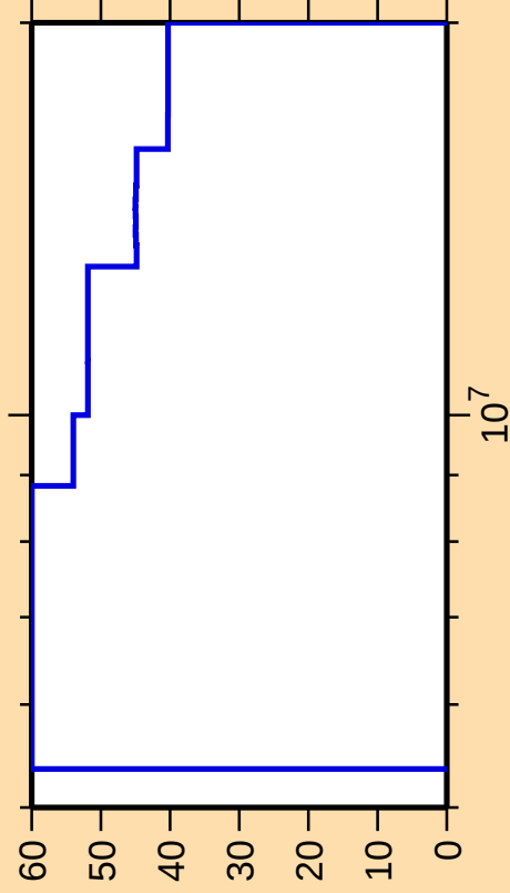
\Delta\sigma/\sigma vs. E for ^{258}\text{Lw}(n,2n)
