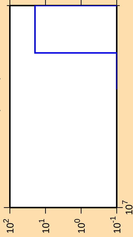
\Delta\sigma/\sigma vs. E for ^{258}\text{Lw(mt 42)}
