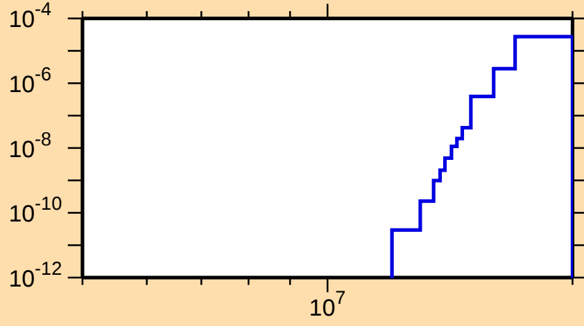
\sigma vs. E for ^{258}\text{Lw}(n,nt)
