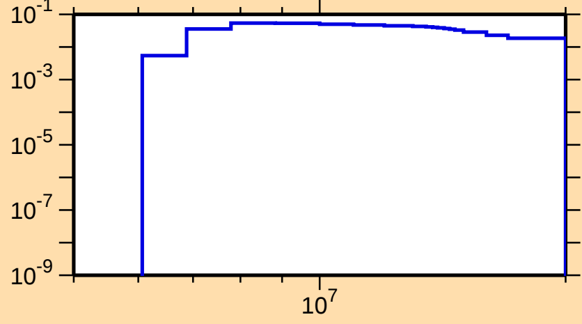
\sigma vs. E for ^{258}\text{Lw}(n,2n\alpha)
