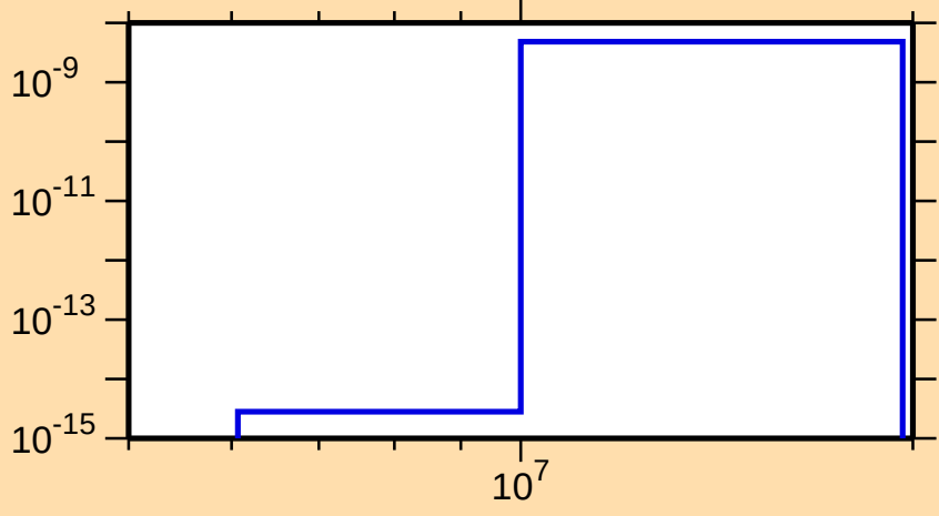
\sigma vs. E for ^{258}\text{Lw}(\text{mt117})
