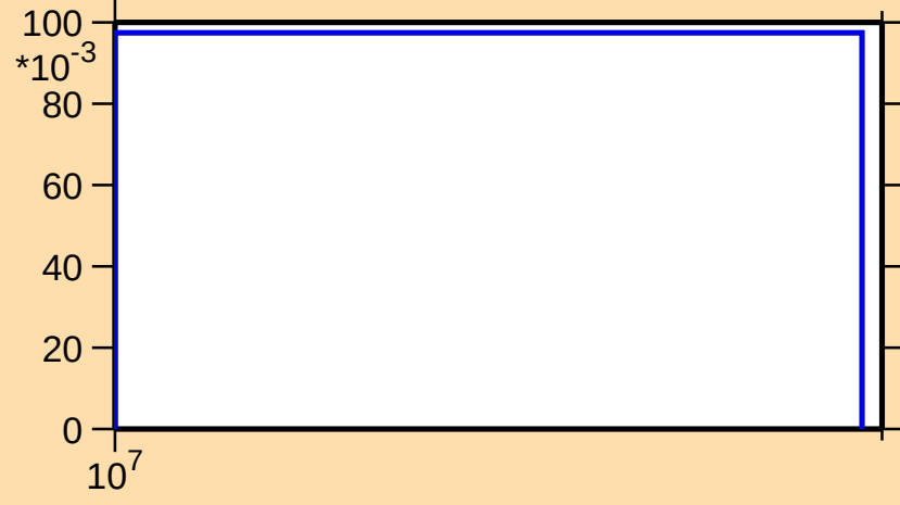
\sigma vs. E for ^{258}\text{Lw}(n,3n)
