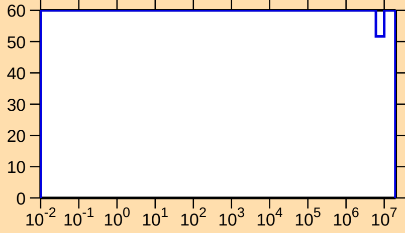
\Delta\sigma/\sigma vs. E for ^{258}\text{Lw}(n,p)
