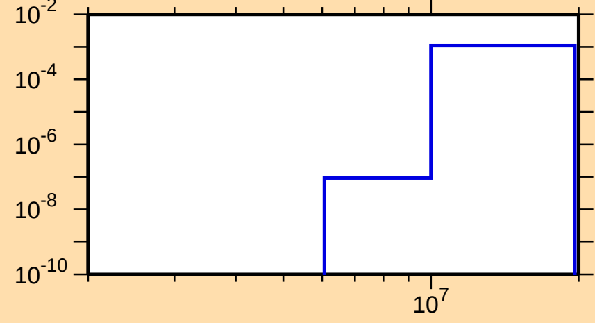
\sigma vs. E for ^{258}\text{Lw}(n,d)
