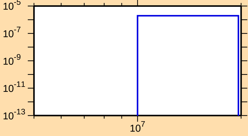
\sigma vs. E for ^{258}\text{Lw}(n,nd)
