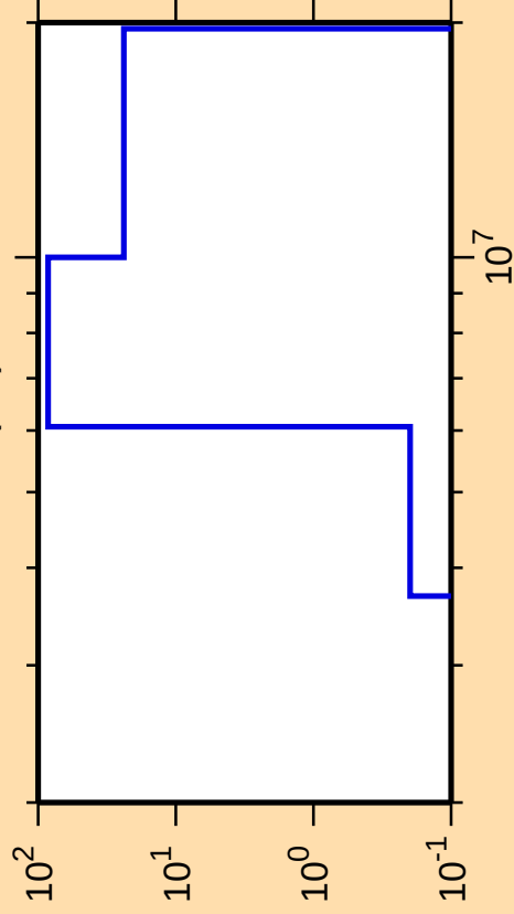
\Delta\sigma/\sigma vs. E for ^{258}\text{Lw}(n,t)
