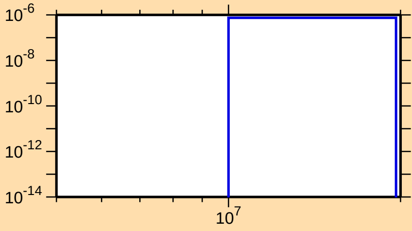
\sigma vs. E for ^{258}\text{Lw}(n,2np)
