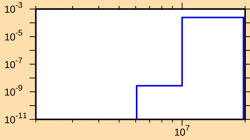
\sigma vs. E for ^{258}\text{Lw}(n,t)
