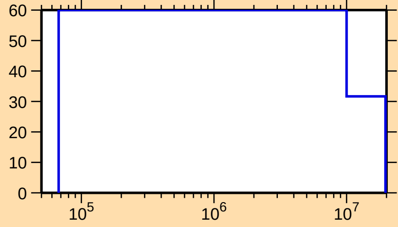
\Delta\sigma/\sigma vs. E for ^{258}\text{Lw}(n,f)
