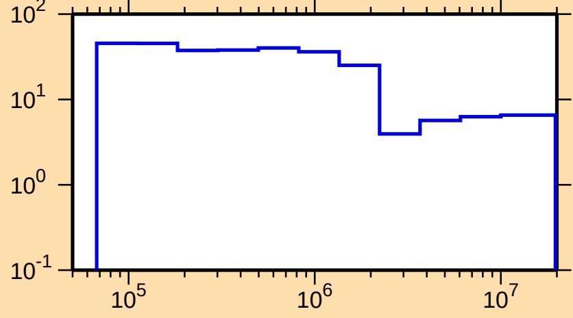
\Delta\sigma/\sigma vs. E for ^{258}\text{Lw}(n,n\text{onel.})
