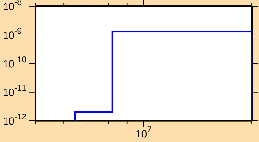
\sigma vs. E for ^{258}\text{Lw}(n,p\alpha)
