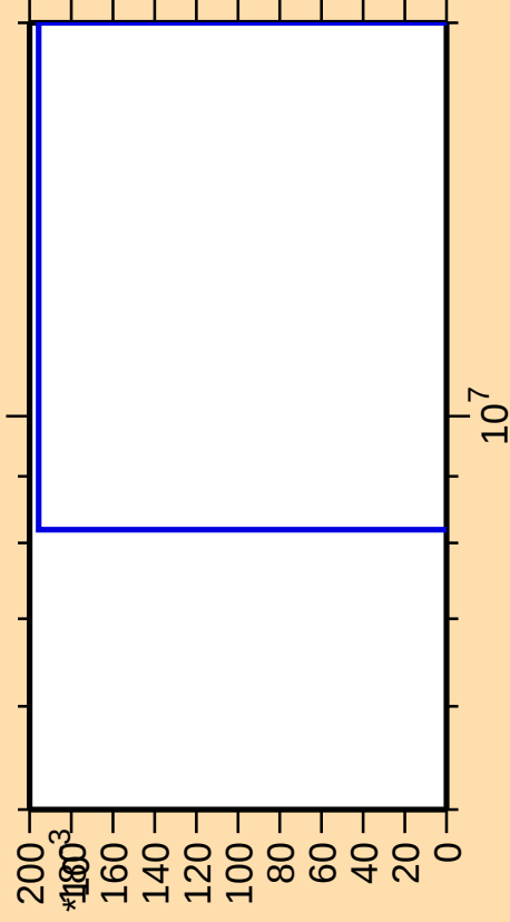
\Delta\sigma/\sigma vs. E for ^{258}\text{Lw(mt 11)}
