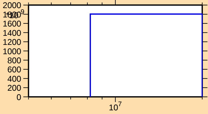
\sigma vs. E for ^{258}\text{Lw}(n,3n\alpha)
