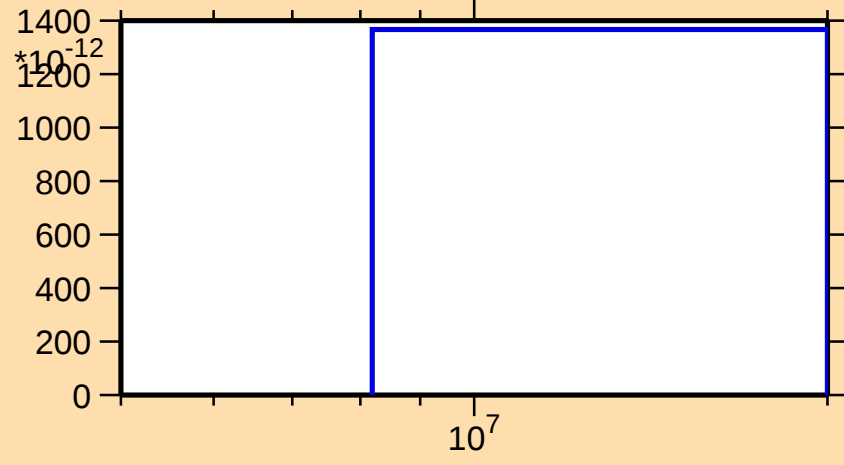
\sigma vs. E for ^{258}\text{Lw(mt 45)}
