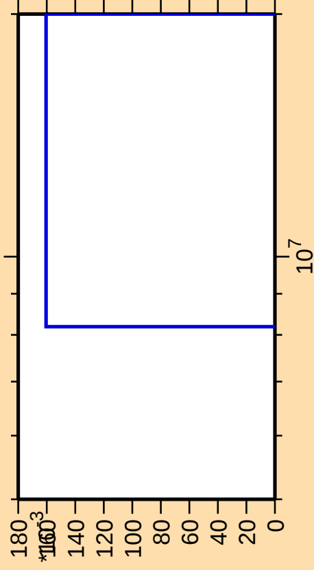
\Delta\sigma/\sigma vs. E for ^{258}\text{Lw(mt 42)}
