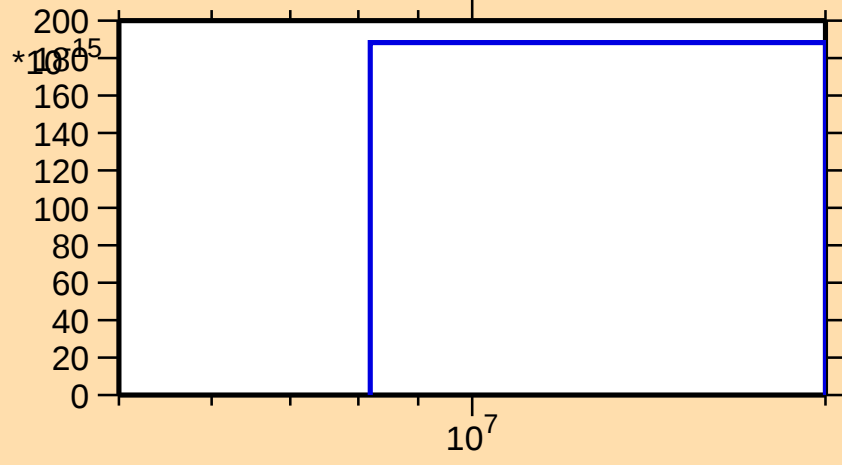
\sigma vs. E for ^{258}\text{Lw(mt 42)}
