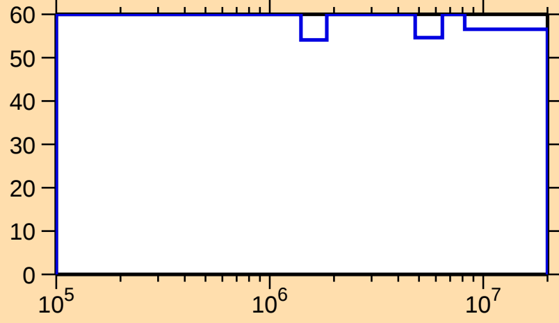
\Delta\sigma/\sigma vs. E for ^{258}\text{Lw}(n,n_1)
