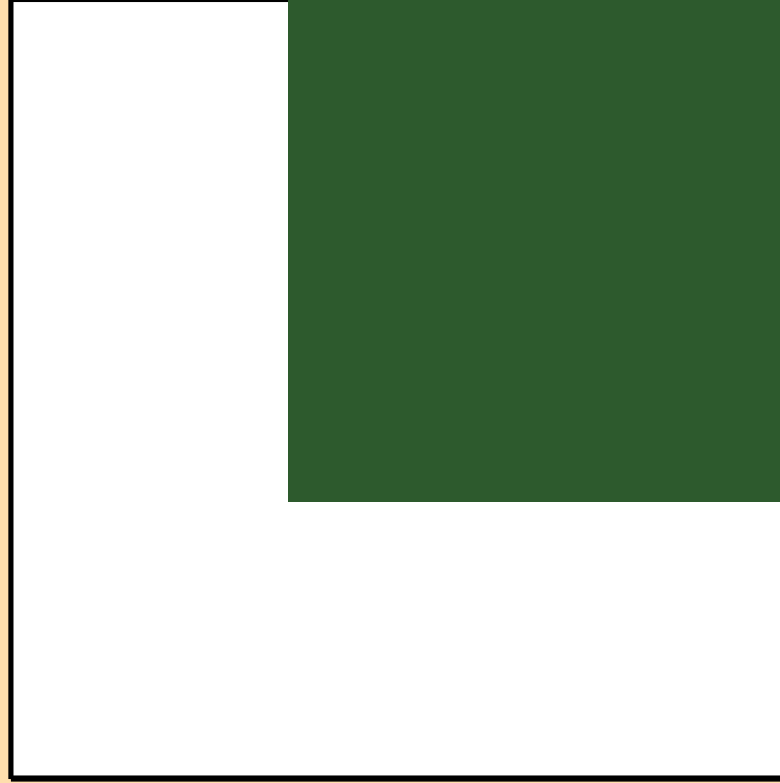
\sigma vs. E for ^{258}\text{Lw}(n,2np)
