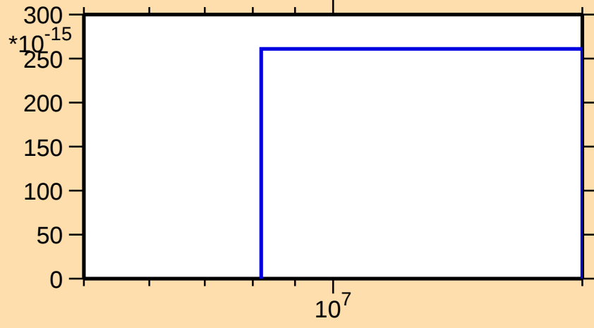
\sigma vs. E for ^{258}\text{Lw(mt 11)}
