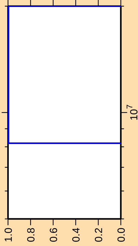
\Delta\sigma/\sigma vs. E for ^{258}\text{Lw(mt 34)}
