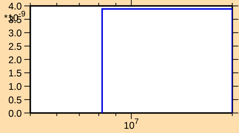
\sigma vs. E for ^{258}\text{Lw(mt117)}
