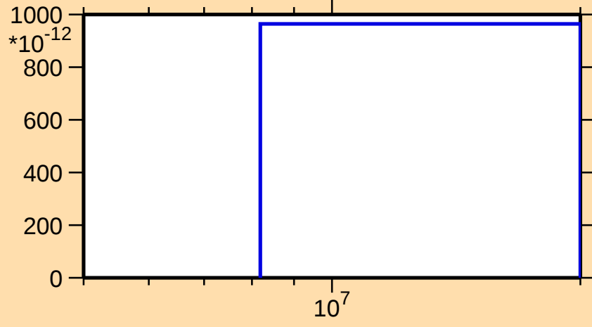
\sigma vs. E for ^{258}\text{Lw}(n,\text{He3})
