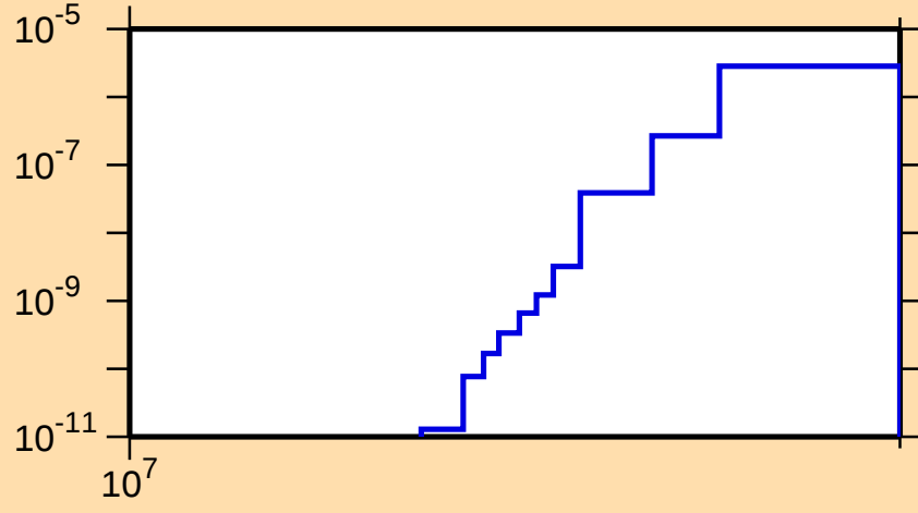
\sigma vs. E for ^{259}\text{Lw}(n,2np)
