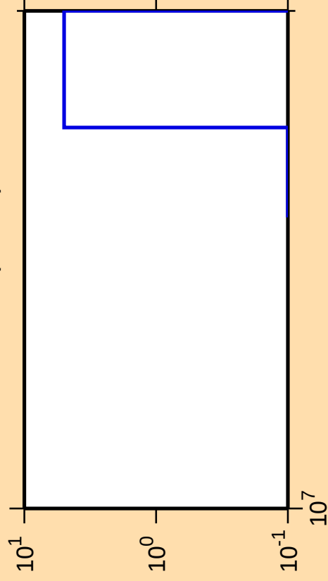
\Delta\sigma/\sigma vs. E for ^{259}\text{Lw(mt 42)}
