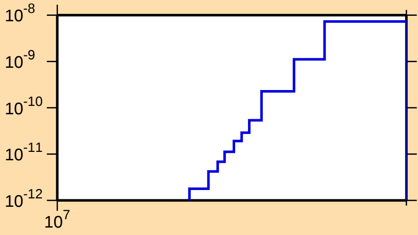
\sigma vs. E for ^{259}\text{Lw}(n,\text{He3})
