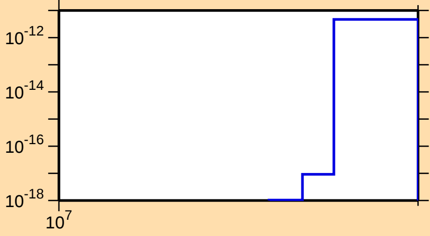
\sigma vs. E for ^{259}\text{Lw(mt 42)}
