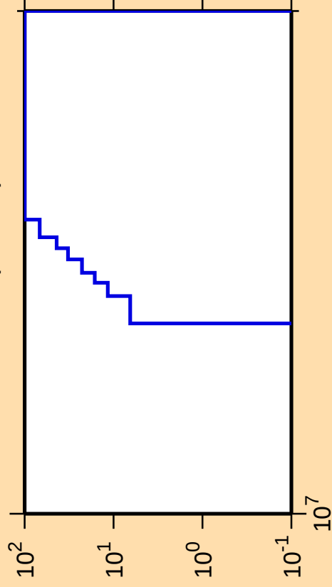
\Delta\sigma/\sigma vs. E for ^{259}\text{Lw(mt117)}
