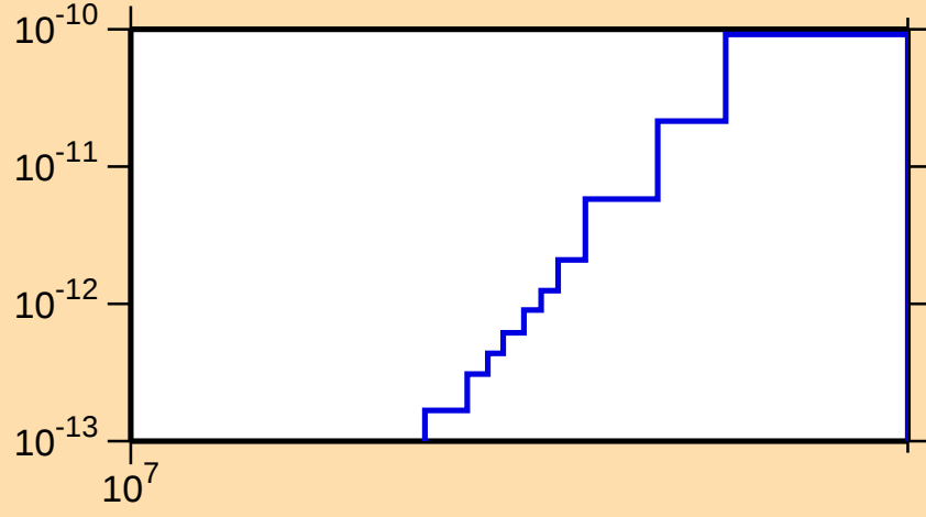
\sigma vs. E for ^{259}\text{Lw(mt 45)}
