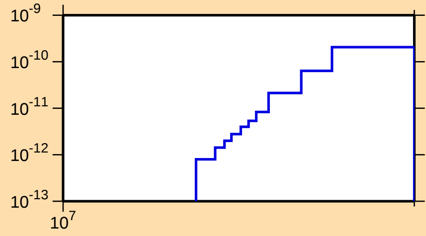
\sigma vs. E for ^{259}\text{Lw(mt117)}
