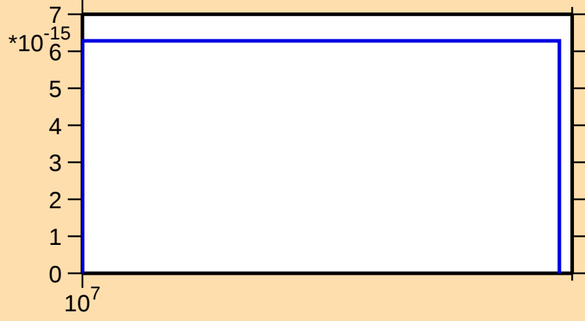
\sigma vs. E for ^{259}\text{Lw}(\text{mt } 34)
