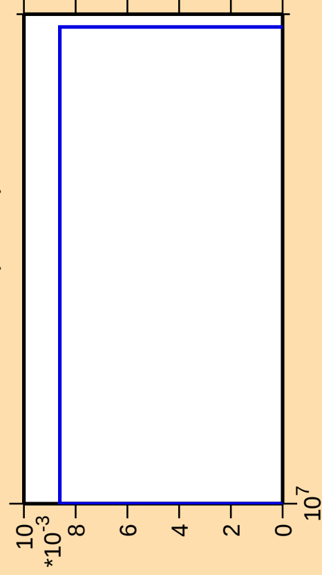
\Delta\sigma/\sigma vs. E for ^{259}\text{Lw}(\text{mt } 34)
