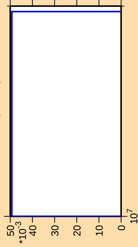
\Delta\sigma/\sigma vs. E for ^{259}\text{Lw(mt 11)}
