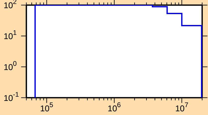
\Delta\sigma/\sigma vs. E for ^{259}\text{Lw}(n,f)
