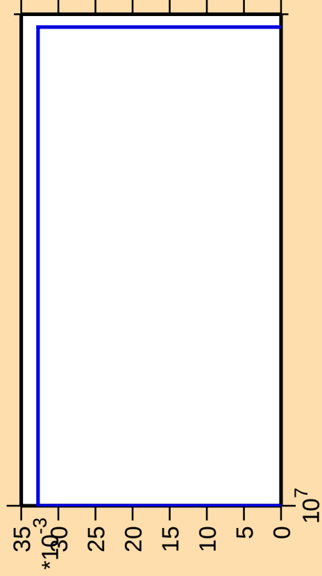
\Delta\sigma/\sigma vs. E for ^{259}\text{Lw}(\text{mt } 42)
