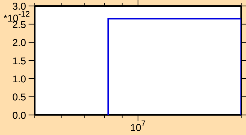
\sigma vs. E for ^{259}\text{Lw}(\text{mt } 45)
