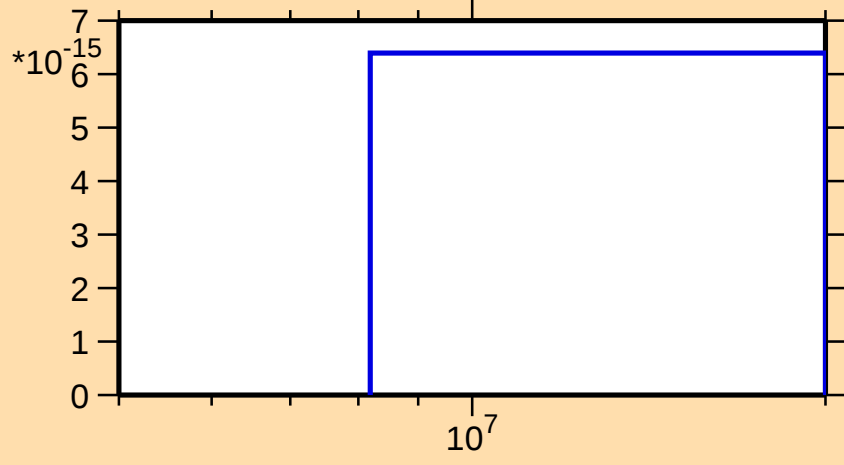
\sigma vs. E for ^{259}\text{Lw(mt 34)}
