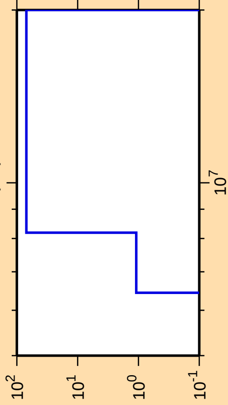
\Delta\sigma/\sigma vs. E for ^{259}\text{Lw}(n,t)
