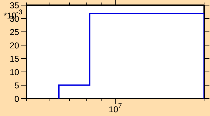
\sigma vs. E for ^{259}\text{Lw}(n,2n\alpha)
