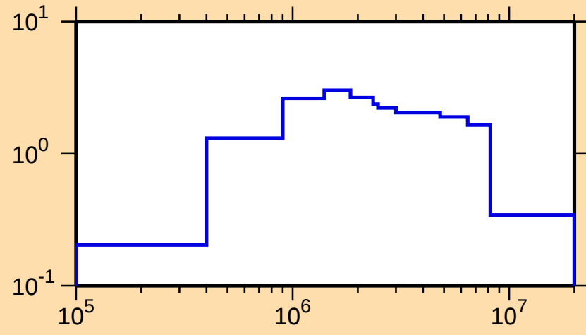
\sigma vs. E for ^{259}\text{Lw}(n,\text{inel.})
