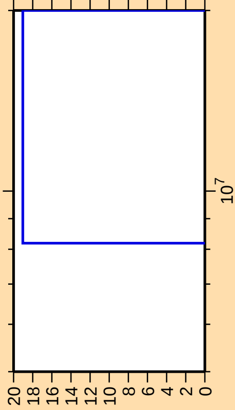
\Delta\sigma/\sigma vs. E for ^{259}\text{Lw}(\text{mt } 45)
