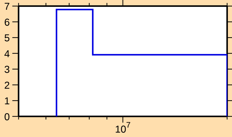
\Delta\sigma/\sigma vs. E for ^{259}\text{Lw}(n,\text{tot.})
