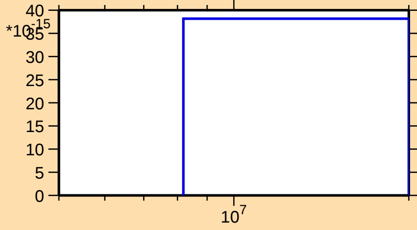
\sigma vs. E for ^{259}\text{Lw}(\text{mt } 42)
