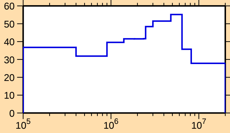
\Delta\sigma/\sigma vs. E for ^{259}\text{Lw}(n,n\text{cont.})
