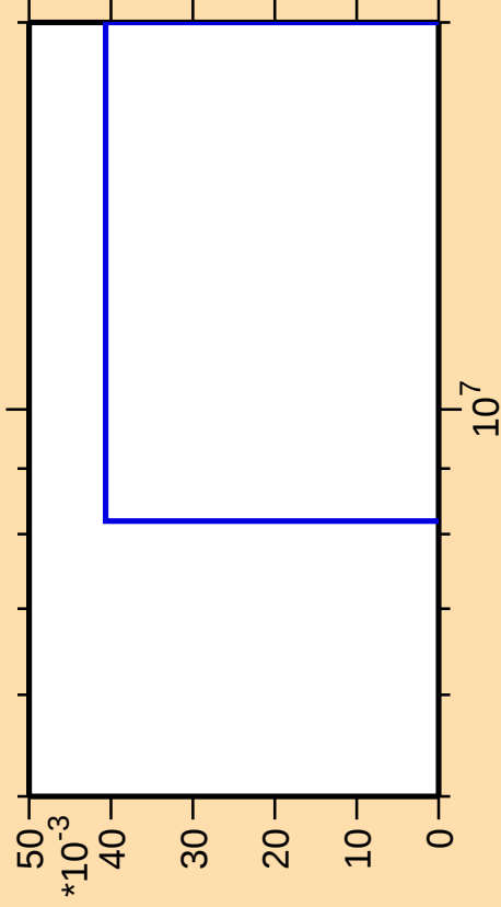
\Delta\sigma/\sigma vs. E for ^{259}\text{Lw}(\text{mt } 42)
