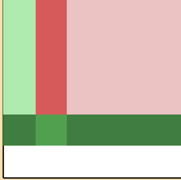
\Delta\sigma/\sigma vs. E for ^{259}\text{Lw}(n,\text{nonel.})
