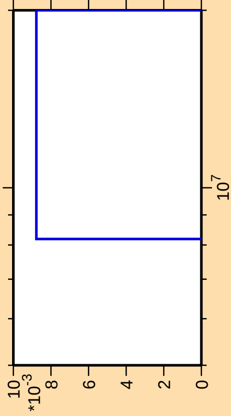
\Delta\sigma/\sigma vs. E for ^{259}\text{Lw(mt 34)}
