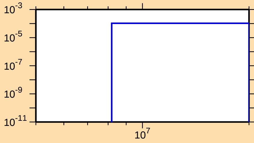
\sigma vs. E for ^{259}\text{Lw}(n,t)
