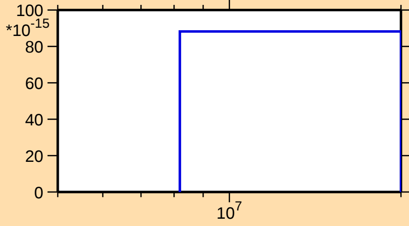
\sigma vs. E for ^{259}\text{Lw(mt 11)}
