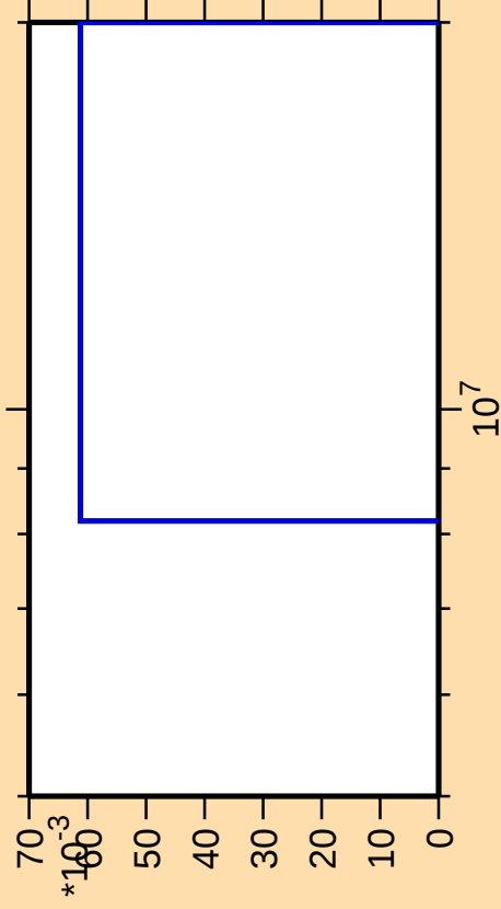
\Delta\sigma/\sigma vs. E for ^{259}\text{Lw(mt 11)}
