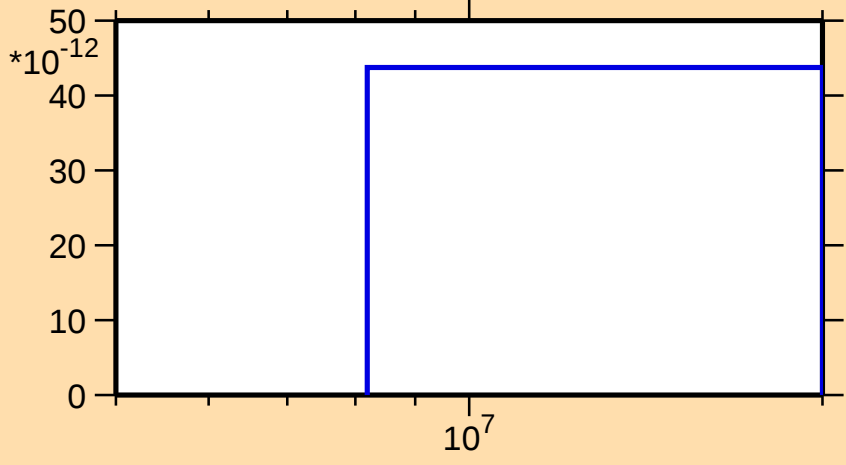
\sigma vs. E for ^{259}\text{Lw}(n,p\alpha)
