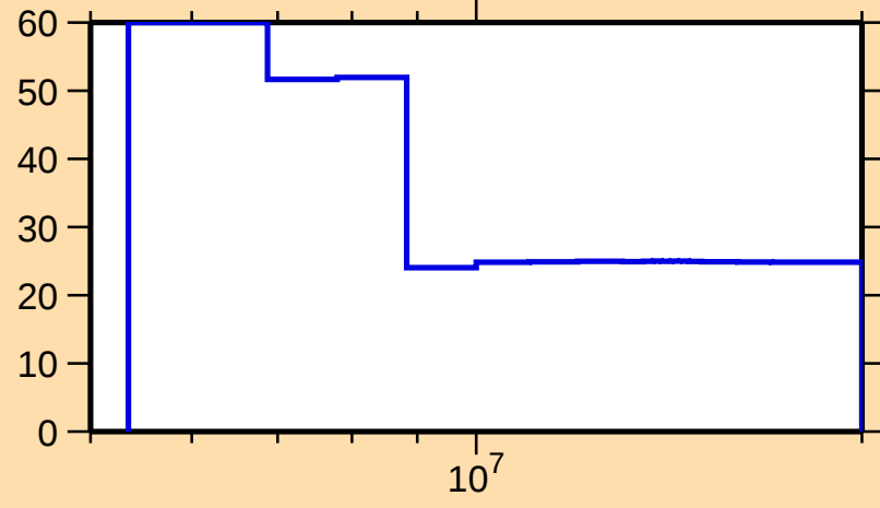
\Delta\sigma/\sigma vs. E for ^{260}\text{Lw}(n,\text{inel.})
