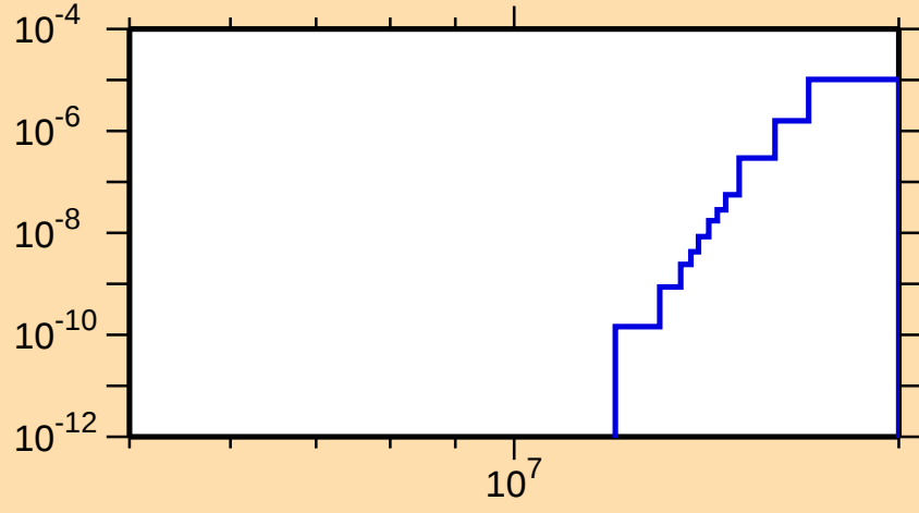
\sigma vs. E for ^{260}\text{Lw}(n,2np)
