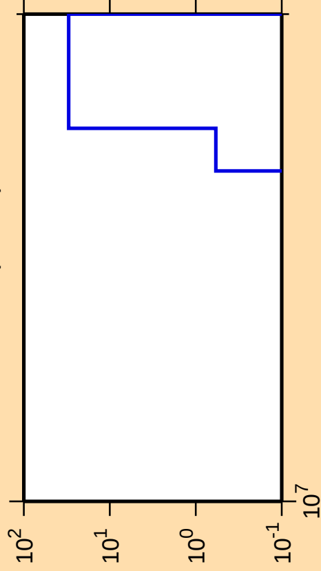
\Delta\sigma/\sigma vs. E for ^{260}\text{Lw(mt 34)}
