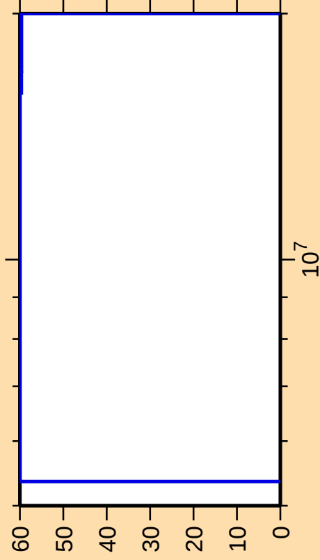
\Delta\sigma/\sigma vs. E for ^{260}\text{Lw}(n,2n)
