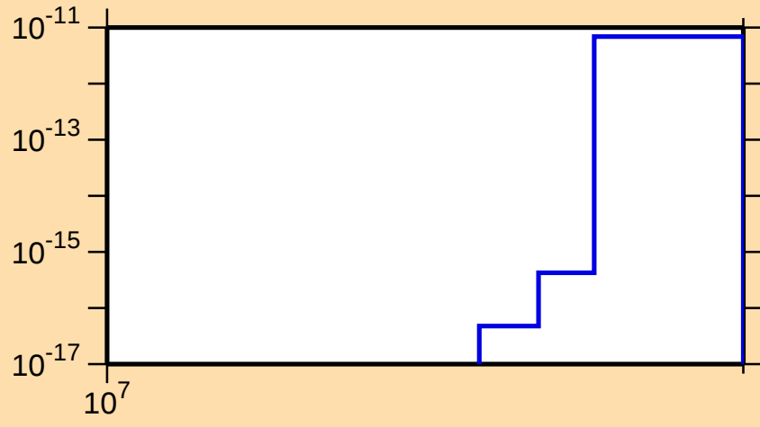
\sigma vs. E for ^{260}\text{Lw(mt 42)}
