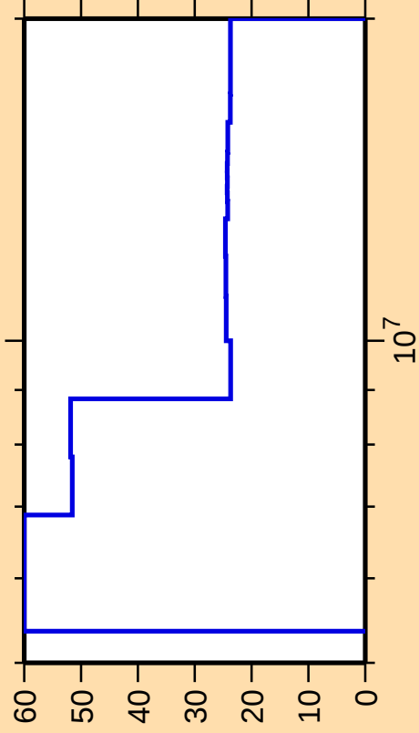
\Delta\sigma/\sigma vs. E for ^{260}\text{Lw}(n,n\text{cont.})
