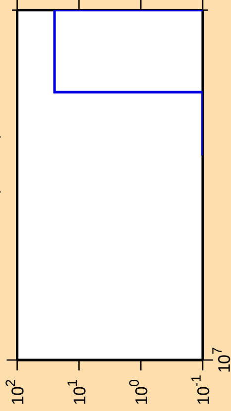
\Delta\sigma/\sigma vs. E for ^{260}\text{Lw(mt 42)}
