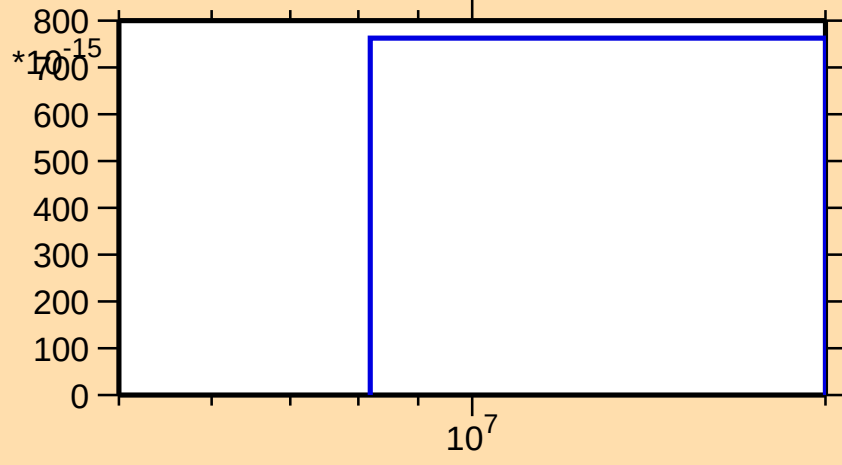
\sigma vs. E for ^{260}\text{Lw(mt117)}
