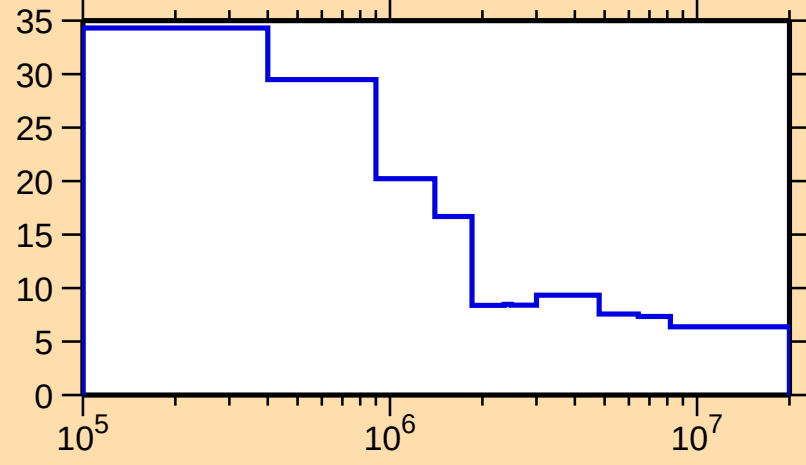
\Delta\sigma/\sigma vs. E for ^{260}\text{Lw}(n,\text{nonel.})
