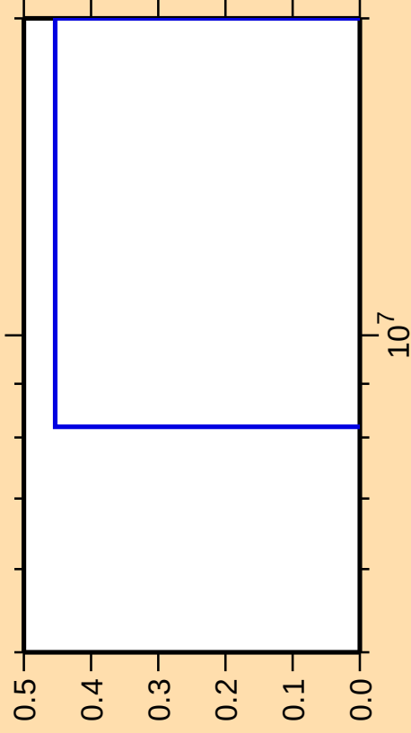
\Delta\sigma/\sigma vs. E for ^{260}\text{Lw(mt 11)}
