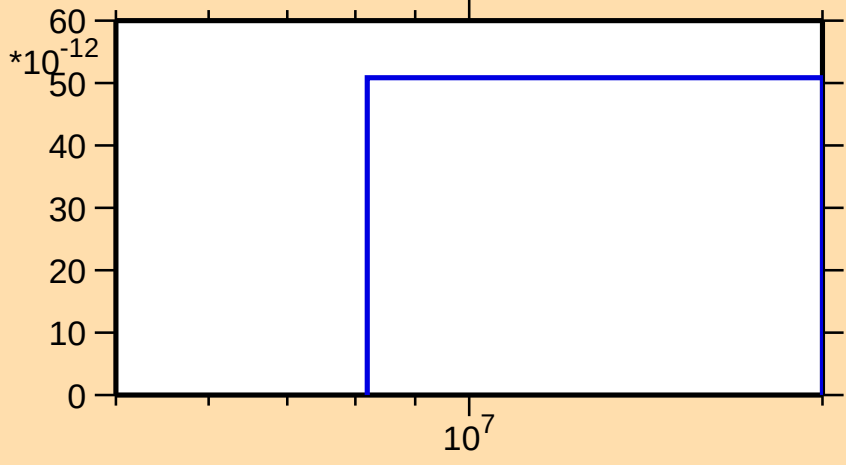
\sigma vs. E for ^{260}\text{Lw}(n,p\alpha)
