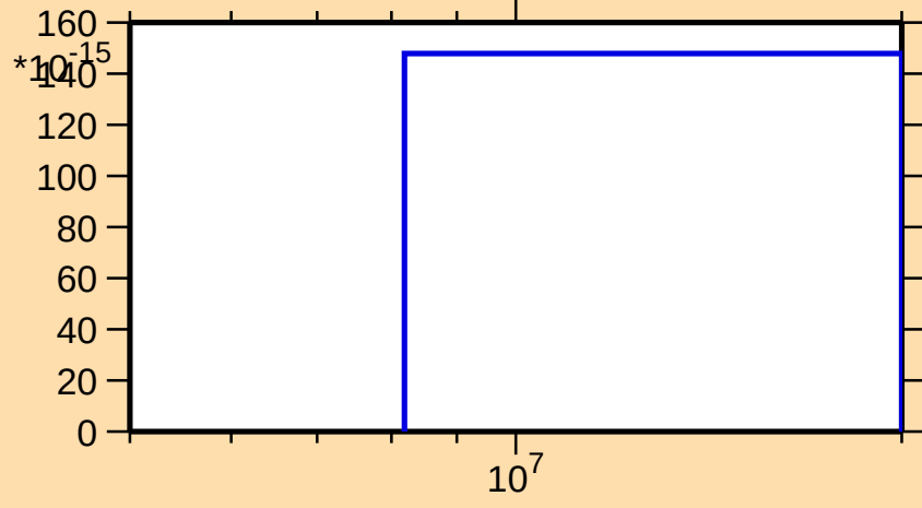
\sigma vs. E for ^{260}\text{Lw(mt 11)}
