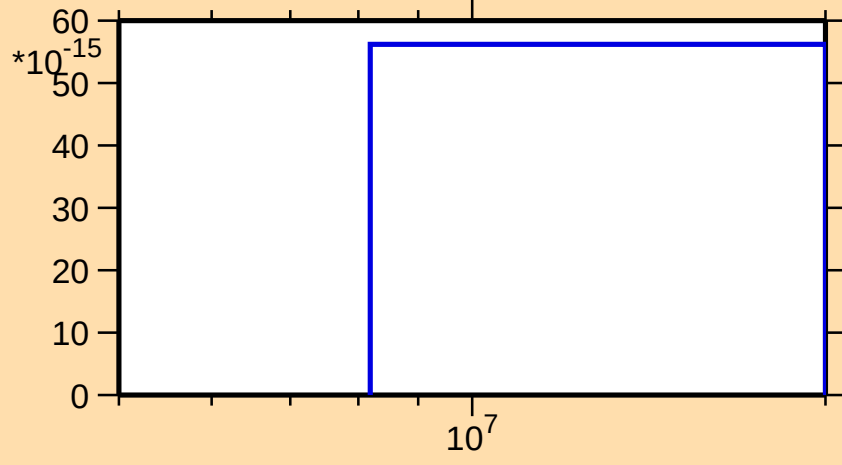
\sigma vs. E for ^{260}\text{Lw(mt 42)}
