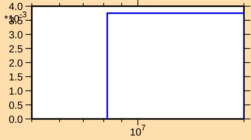
\sigma vs. E for ^{260}\text{Lw}(n,3n\alpha)
