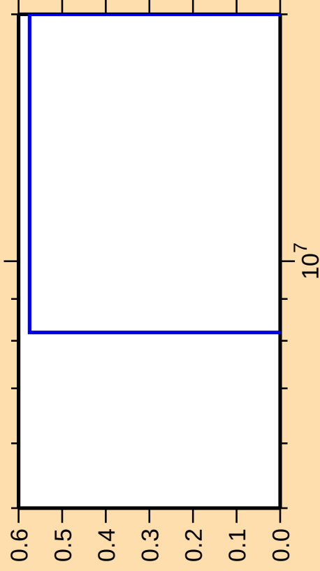
\Delta\sigma/\sigma vs. E for ^{260}\text{Lw(mt 45)}
