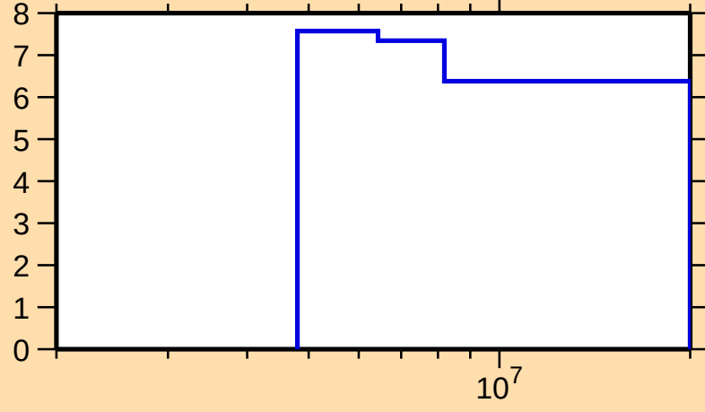
\Delta\sigma/\sigma vs. E for ^{260}\text{Lw}(n,\text{nonel.})
