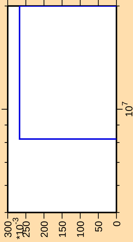
\Delta\sigma/\sigma vs. E for ^{260}\text{Lw(mt 34)}
