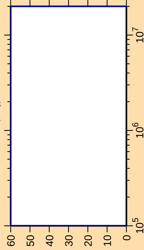
\Delta\sigma/\sigma vs. E for ^{260}\text{Lw}(n,\gamma)
