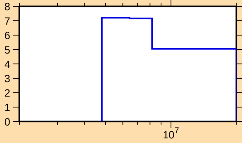
\Delta\sigma/\sigma vs. E for ^{260}\text{Lw}(n,\text{el.})
