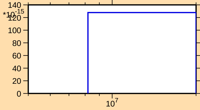
\sigma vs. E for ^{260}\text{Lw(mt 45)}
