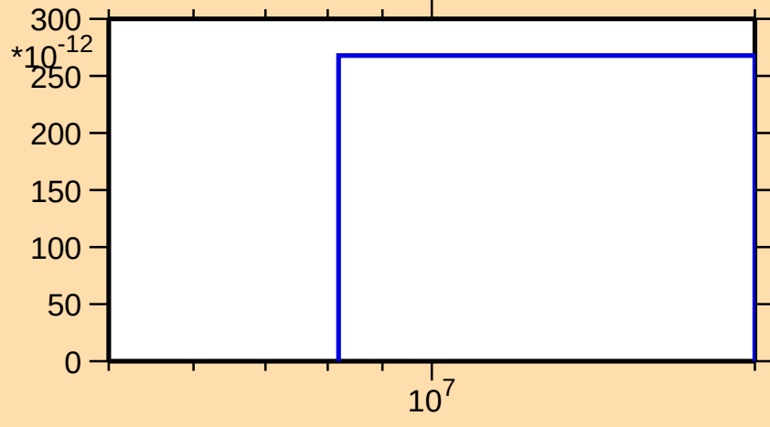
\sigma vs. E for ^{260}\text{Lw}(n,\text{He3})
