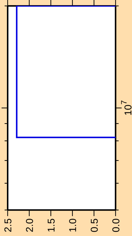
\Delta\sigma/\sigma vs. E for ^{260}\text{Lw(mt117)}
