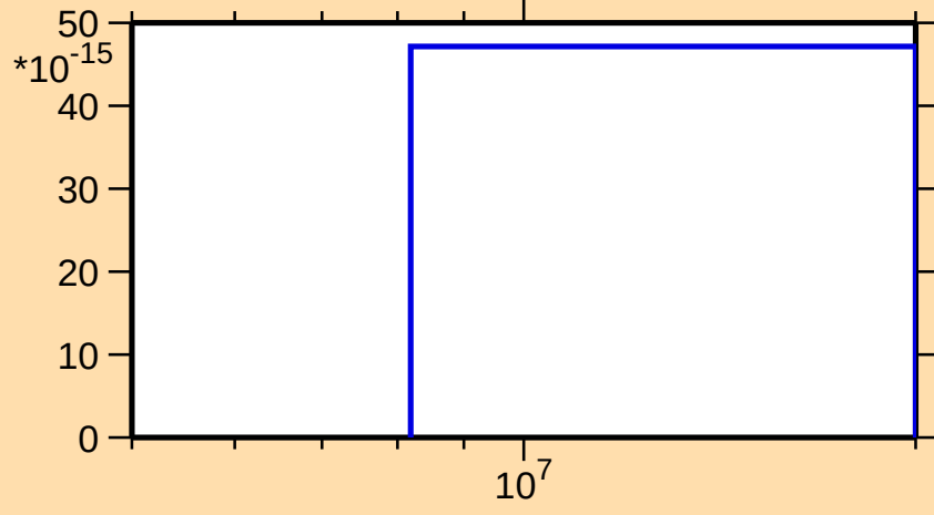
\sigma vs. E for ^{260}\text{Lw(mt 34)}
