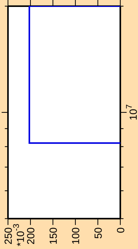
\Delta\sigma/\sigma vs. E for ^{260}\text{Lw(mt 42)}
