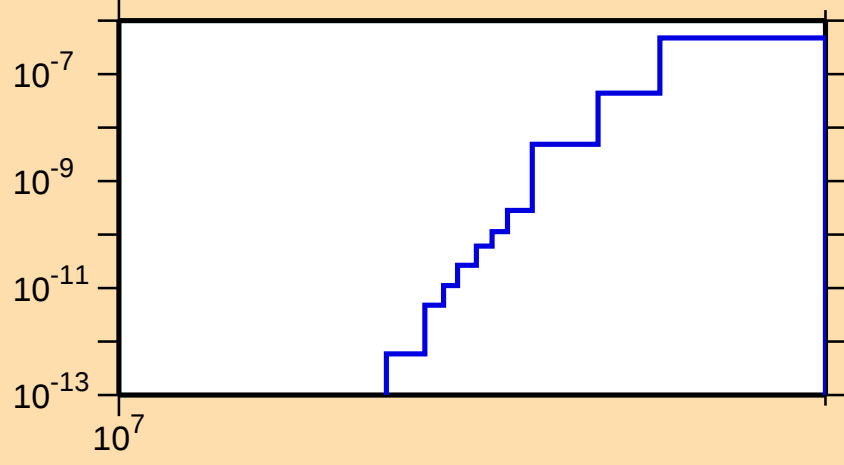
\sigma vs. E for ^{261}\text{Lw}(n,2np)
