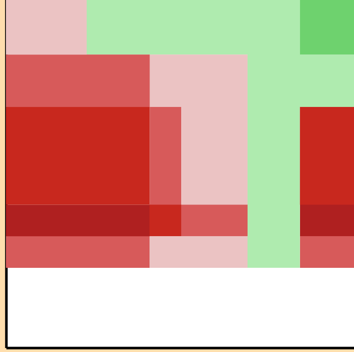
\Delta\sigma/\sigma vs. E for ^{261}\text{Lw}(n,\text{el.})
