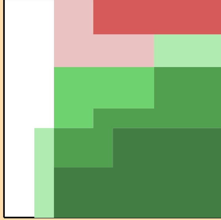
\Delta\sigma/\sigma vs. E for ^{261}\text{Lw}(n,2n)
