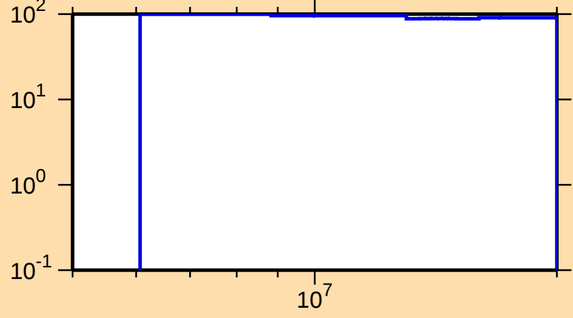
\Delta\sigma/\sigma vs. E for ^{261}\text{Lw}(n,2n)
