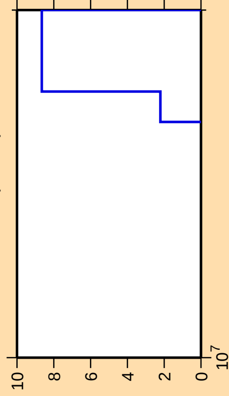
\Delta\sigma/\sigma vs. E for ^{261}\text{Lw(mt 45)}
