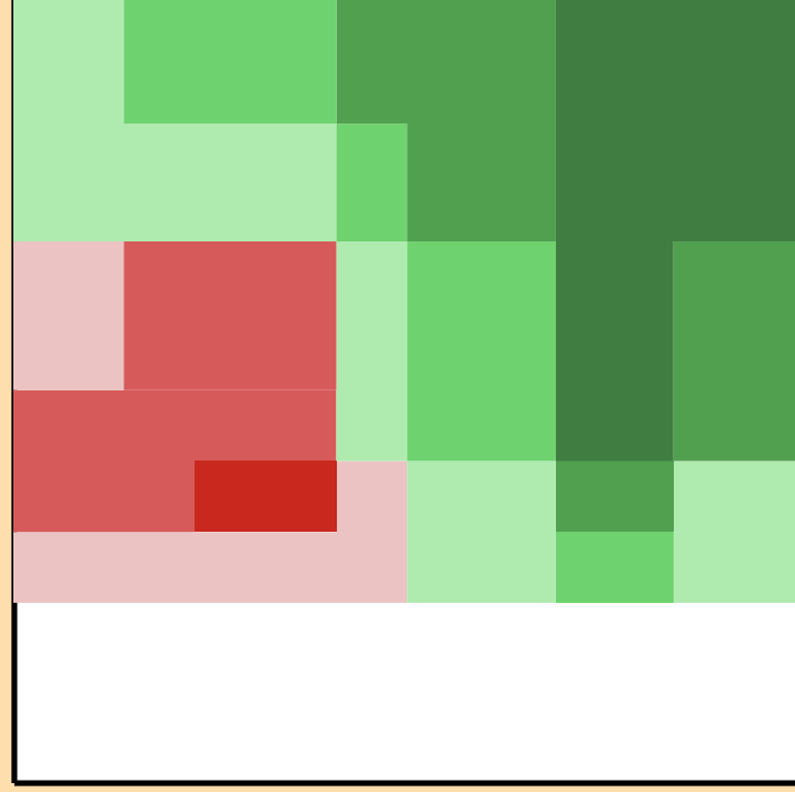
\Delta\sigma/\sigma vs. E for ^{261}\text{Lw}(n,\text{tot.})
