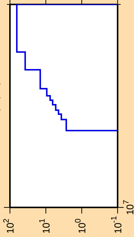
\Delta\sigma/\sigma vs. E for ^{261}\text{Lw}(n,p\alpha)
