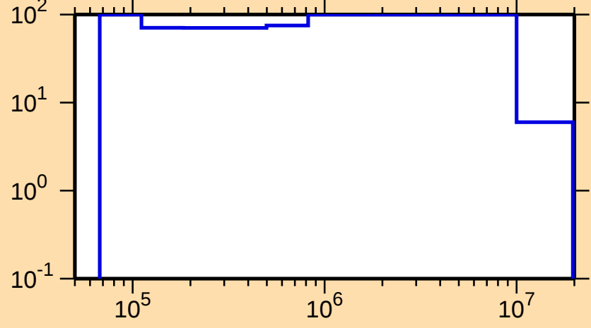
\Delta\sigma/\sigma vs. E for ^{261}\text{Lw}(n,n_1)
