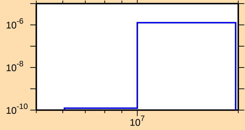
\sigma vs. E for ^{261}\text{Lw}(n,2n\alpha)
