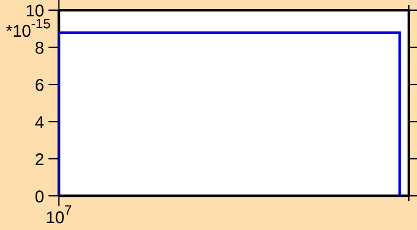
\sigma vs. E for ^{261}\text{Lw(mt 42)}
