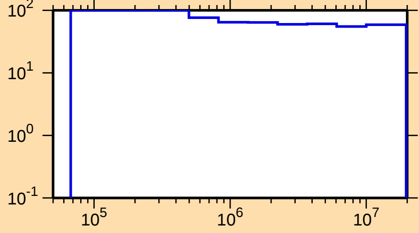
\Delta\sigma/\sigma vs. E for ^{261}\text{Lw}(n,\text{inel.})
