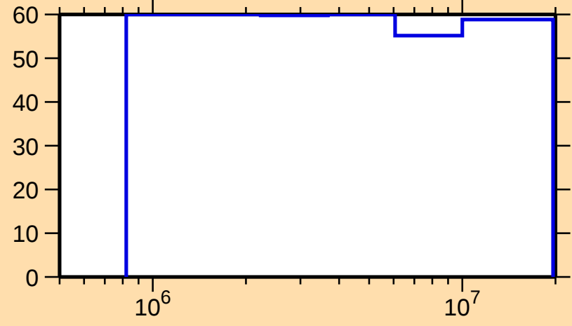
\Delta\sigma/\sigma vs. E for ^{261}\text{Lw}(n,\text{ncont.})
