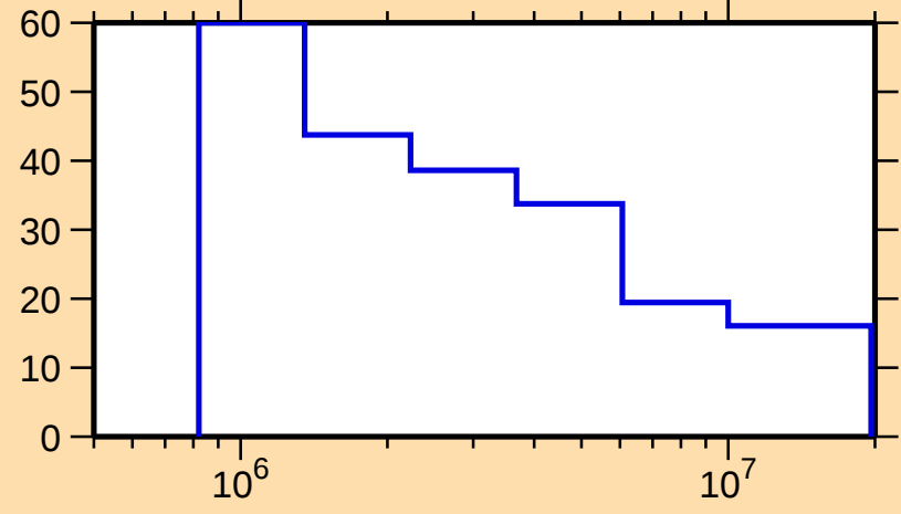
\Delta\sigma/\sigma vs. E for ^{261}\text{Lw}(n,f)
