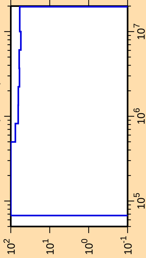
\Delta\sigma/\sigma vs. E for ^{261}\text{Lw}(n,\text{inel.})
