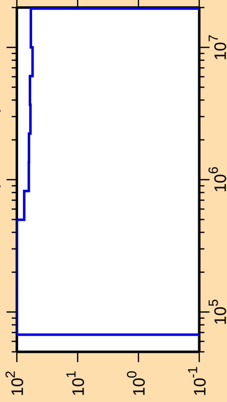
\Delta\sigma/\sigma vs. E for ^{261}\text{Lw}(n,\text{ncont.})
