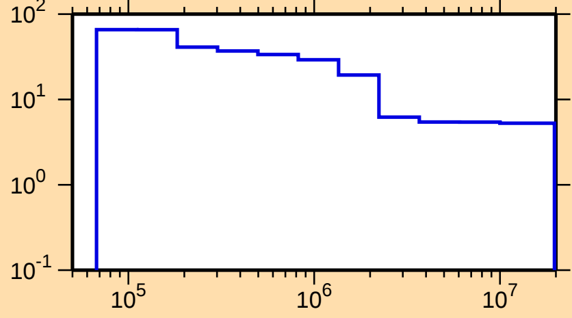
\Delta\sigma/\sigma vs. E for ^{261}\text{Lw}(n,\text{nonel.})
