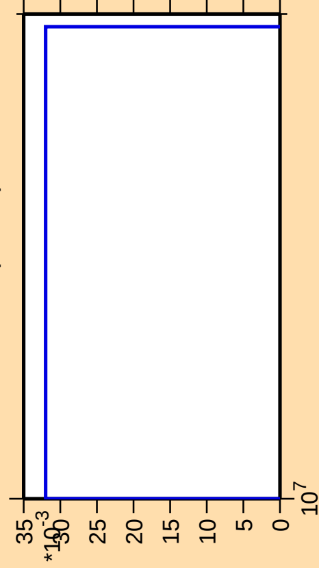
\Delta\sigma/\sigma vs. E for ^{261}\text{Lw(mt 42)}
