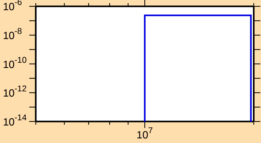
\sigma vs. E for ^{261}\text{Lw}(n,nt)
